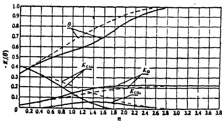
Figure 4. The distributions of the dimensionless temperature \theta and the mass ratio K_i (i = CO, CO_2, O) along \eta in the combustion of carbon monoxide. T_w = 6000K T_\infty = 2000K P = 3.5 \text{ atm} -f_w = 0.25 Le = 1.2 Pr = 0.71 Key: 2. wall surface reaction, 3. equilibrium: the reaction in the boundary layer is CO + O = CO_2 (assuming nitrogen does not recombine), 4. equilibrium distribution, 5. frozen distribution.
