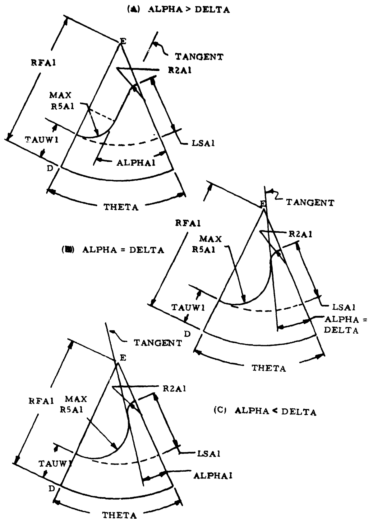
Figure 41. Definition of DELTA, Type 1 Grain
