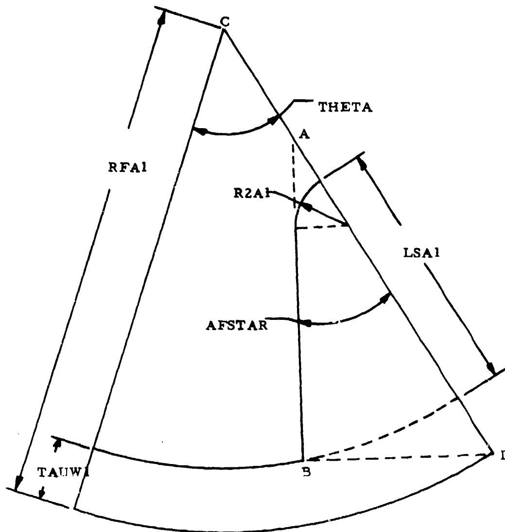
Figure 39. Definition of AFSTAR, Type 1 Grain
