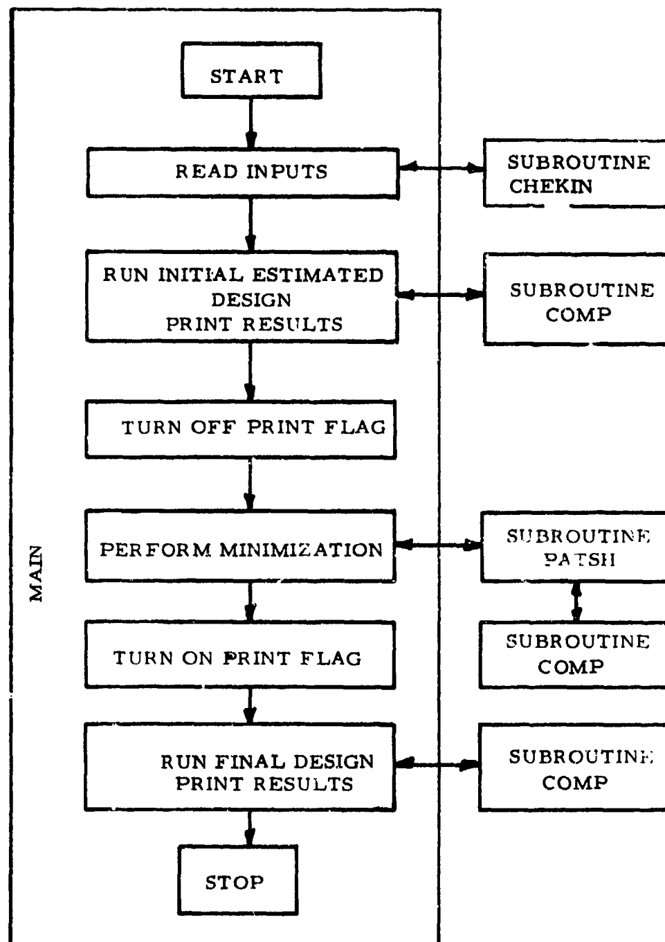
Figure 6. Overall Code Flowchart
