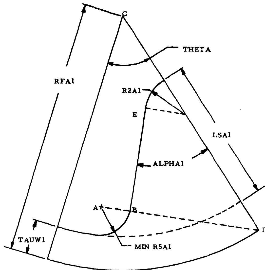
Figure 40. Minimum RFAI when ALPHA1 > AFSTAR, Type 1 Grain
