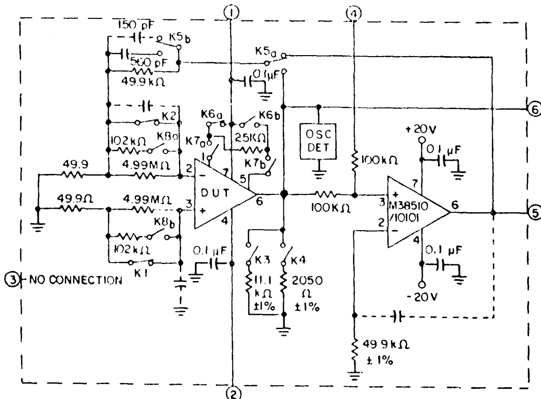
Figure 3-2. Test Circuit for Static Tests
