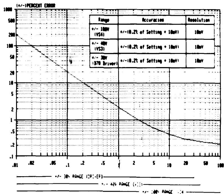
Figure 2-10. S3260/70 - Forcing Voltage Accuracies
