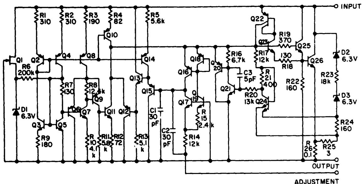
Figure 11-2. Schematic Diagram of 3-Terminal Adjustable Positive Voltage Regulator
