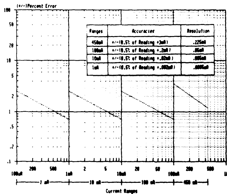
Figure 2-5. S3260/70 - Current Measurement Accuracies (Cont'd.)
