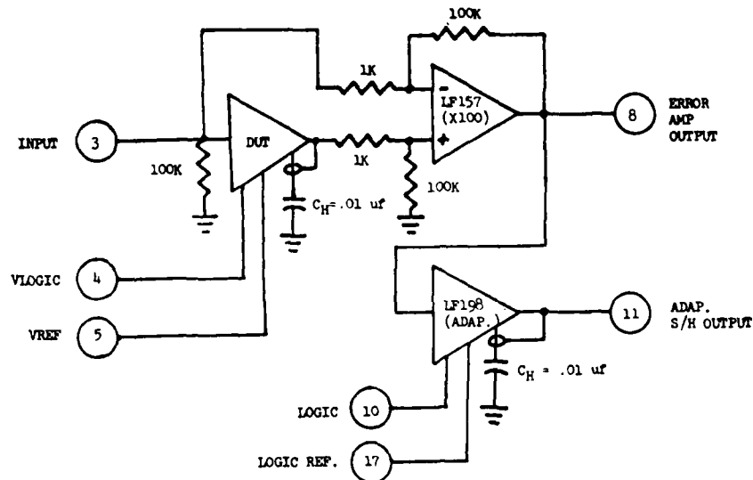
Figure 5-5. Acquisition Time and Aperture Time Test Circuit
