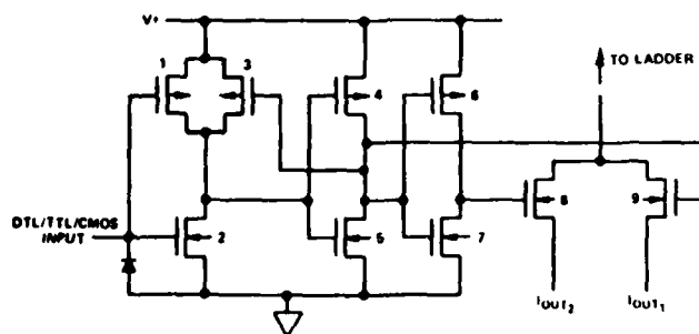
Figure 8-2. CMOS Switch Schematic.
