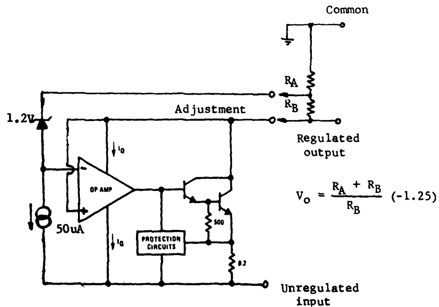
Figure 12-2. Block Diagram of 3-Terminal Adjustable Negative Voltage Regulators.
