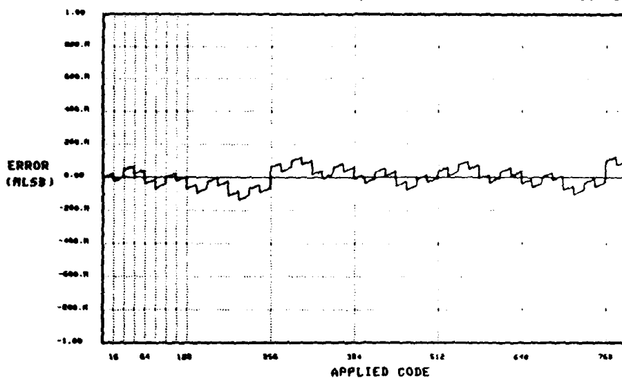
Figure 2-17. LINEARITY ERROR (ALL CODES)
