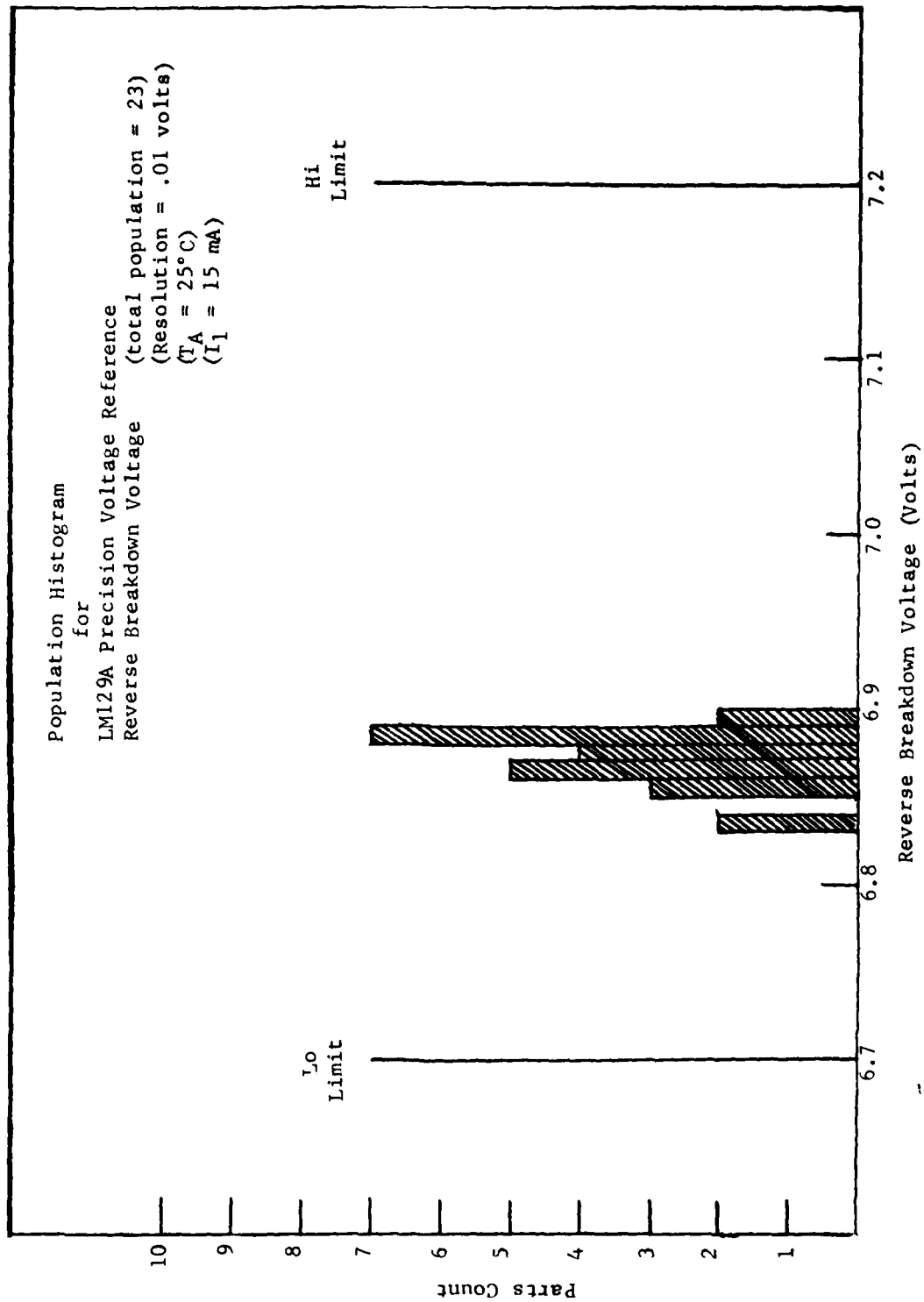
Figure 13-4. Population histogram for LM129A precision voltage reference.
