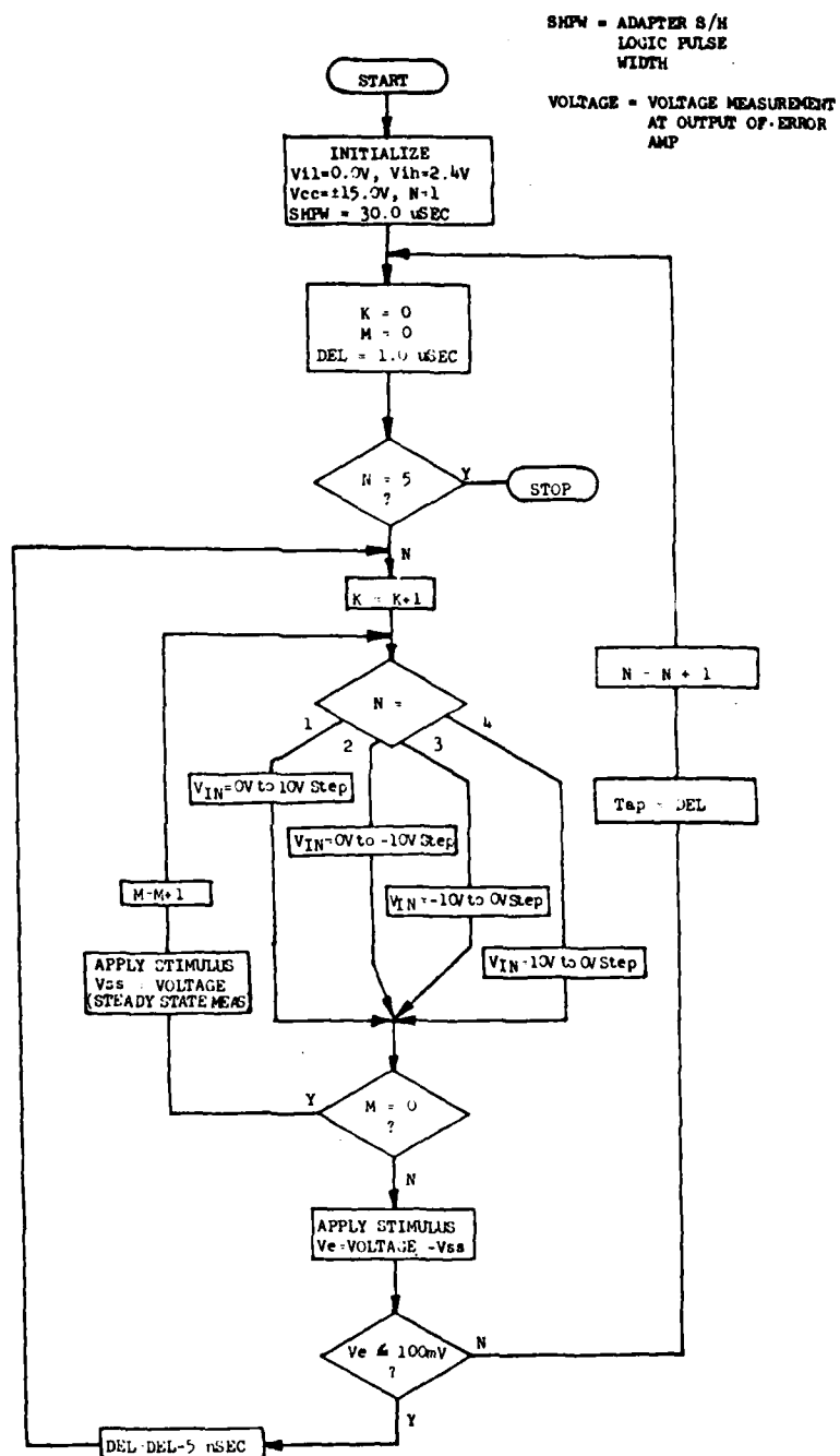
Figure 5-9. Aperture Time Flow Chart
