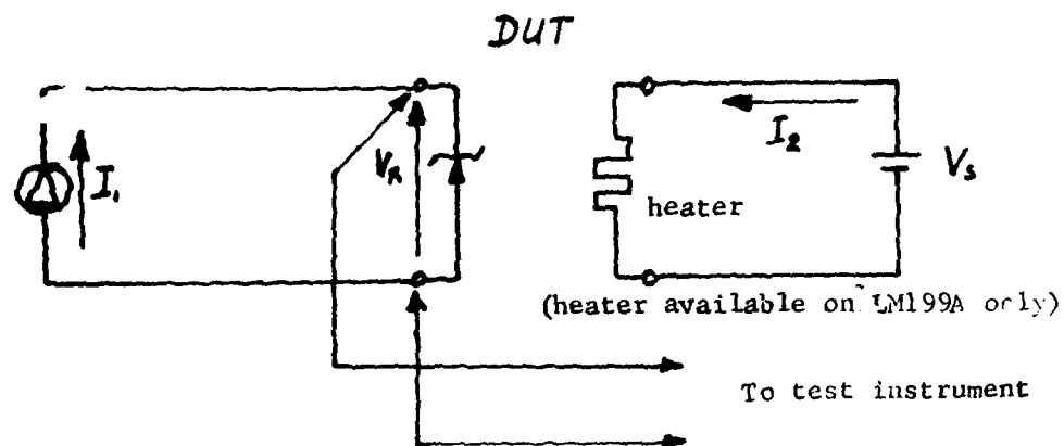
Figure 13-2. Reference voltage and noise test circuit.
