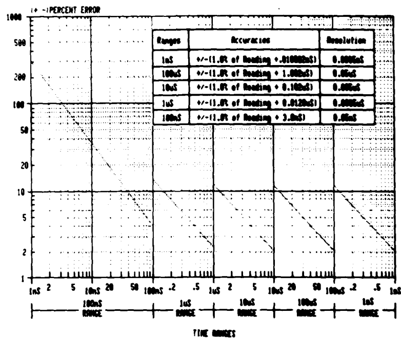
Figure 2-6. S3260/70 - Time Measurement Accuracies
