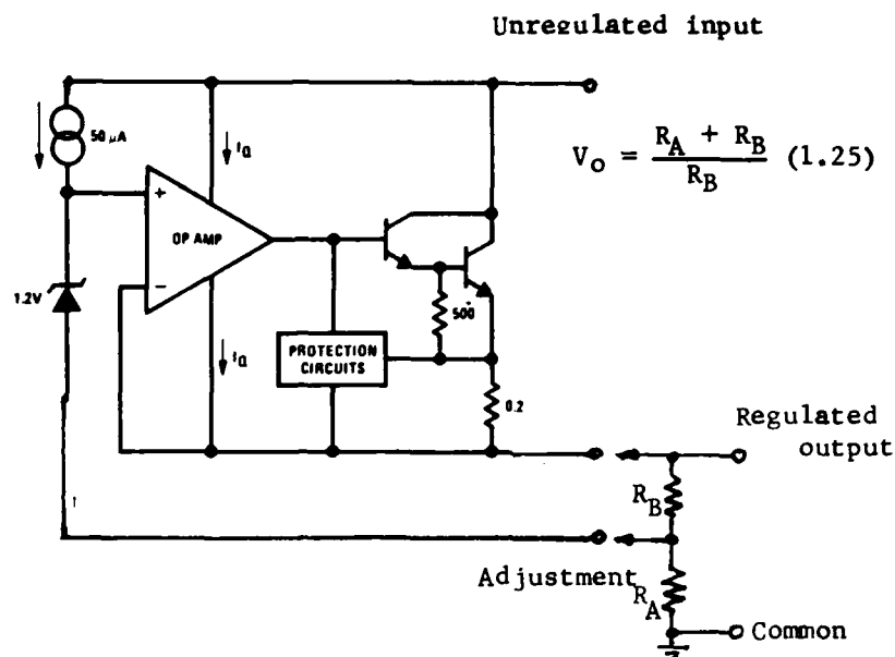
Figure 10-2. Block Diagram of 3-Terminal Adjustable Positive Voltage Regulators.)
