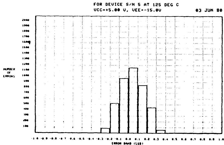
Figure 2-19. LINEARITY ERROR DISTRIBUTION 562-12 BIT D/A CONVERTER
