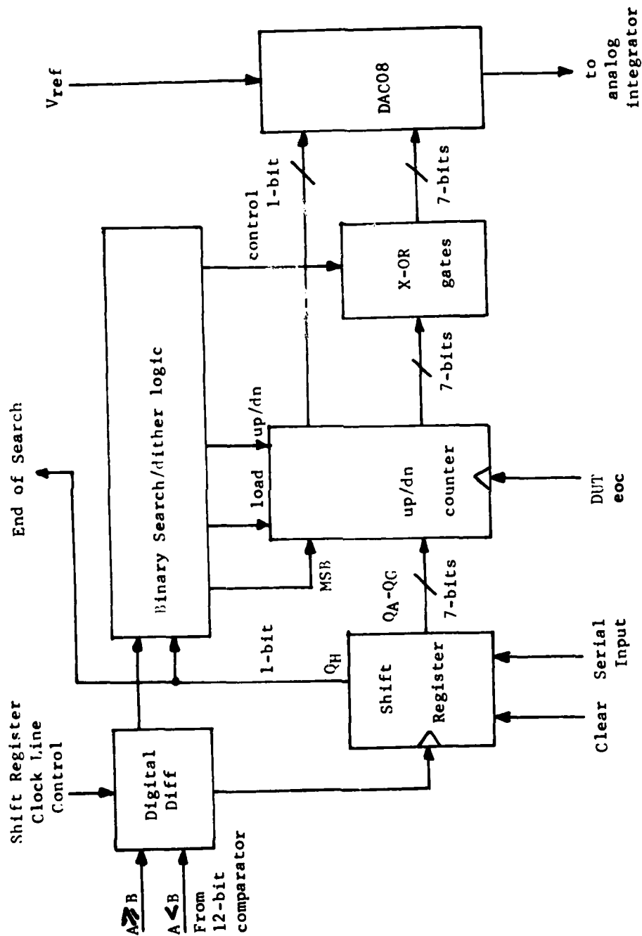
Figure 9-21. Block Diagram of Binary Search and Dither Circuit
