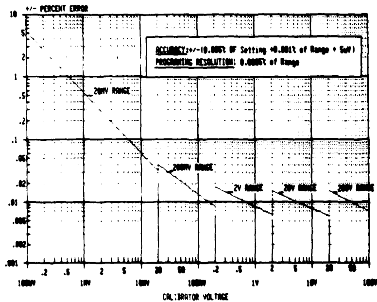
Figure 2-12. Fluke 8100B Meter Calibrator - Forcing Voltage Accuracies
