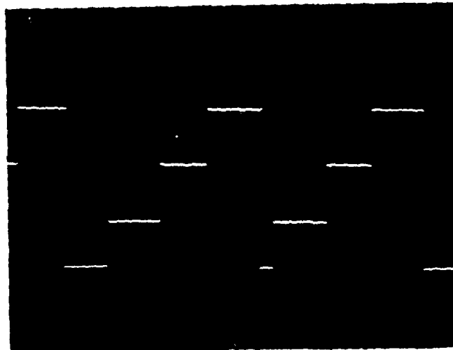
Figure 9-14. DUT Output at Mid-range showing Narrow Step Width for Code-word 1000 0000 0000.
