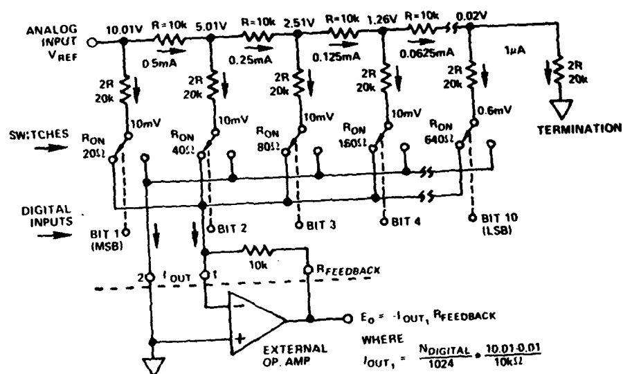
Figure 8-3. Typical Voltage Output Functional Schematic.
