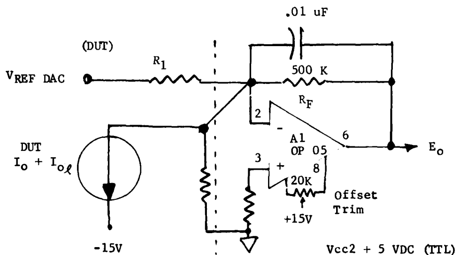
Simplified schematic of error amplifier.
