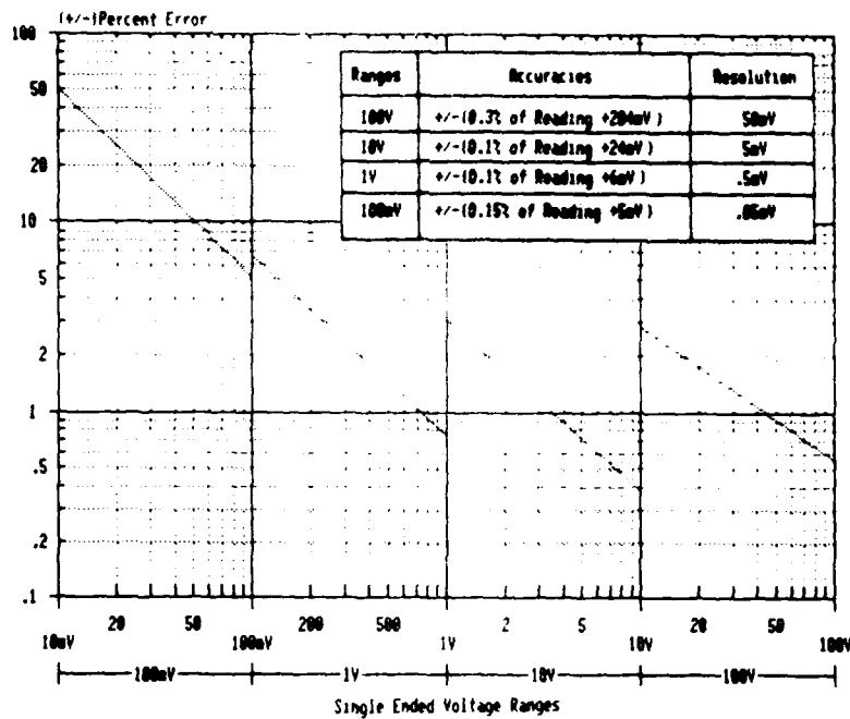
Figure 2-1. S3260/70 - Single Ended Voltage Accuracies
