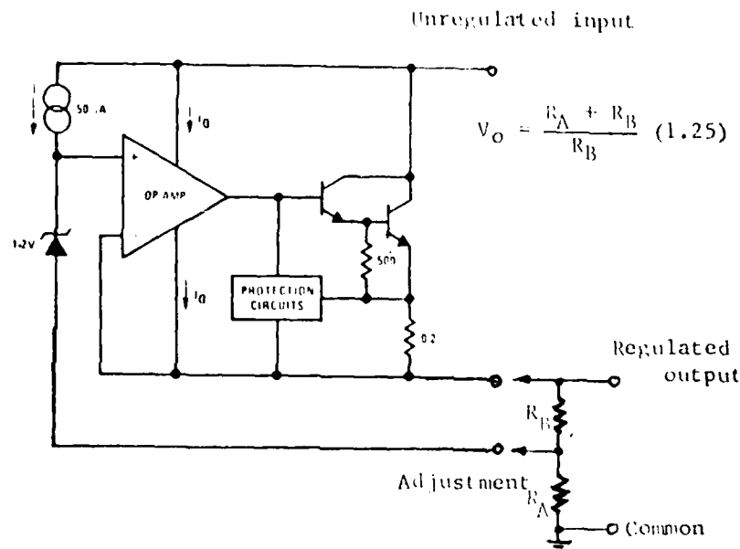
Figure 11-1. Block Diagram of 3-Terminal Adjustable Positive Voltage Regulators
