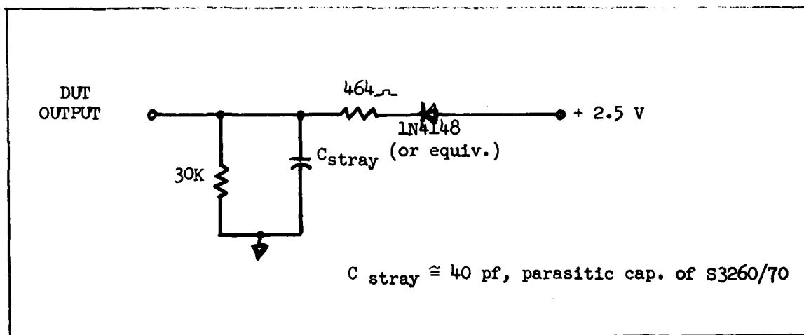
Figure 9-7 A/D Converter Load Circuit
