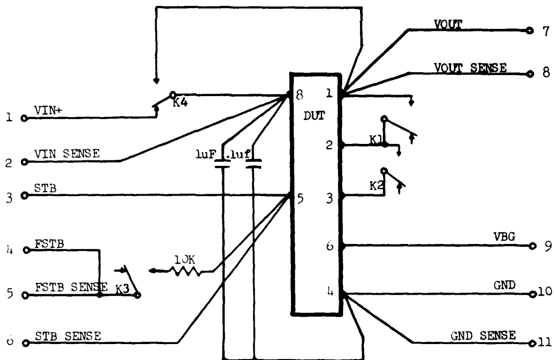
Figure 14-2. S3270 Test Circuit for Static Tests.
