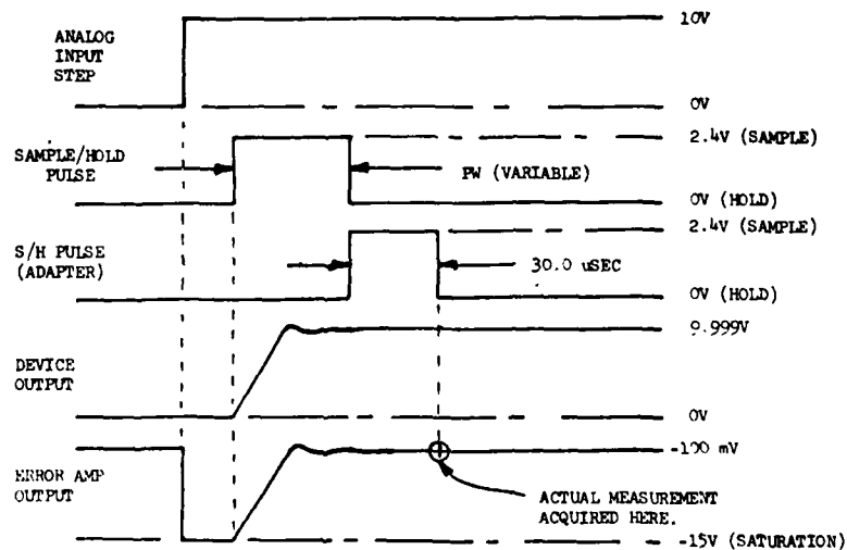
Figure 5-6. Acquisition Time Test Timing Diagram
