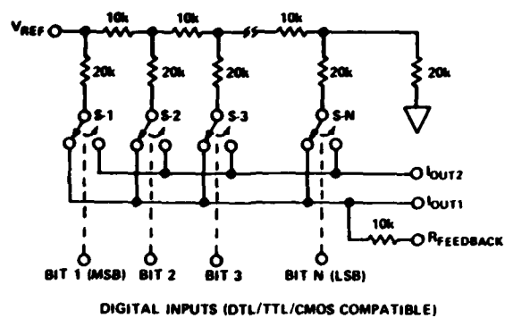
Figure 8-1. CMOS Multiplying DAC Schematic.
