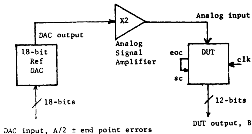
Figure 9-18. Simple Digital Measurement Technique
