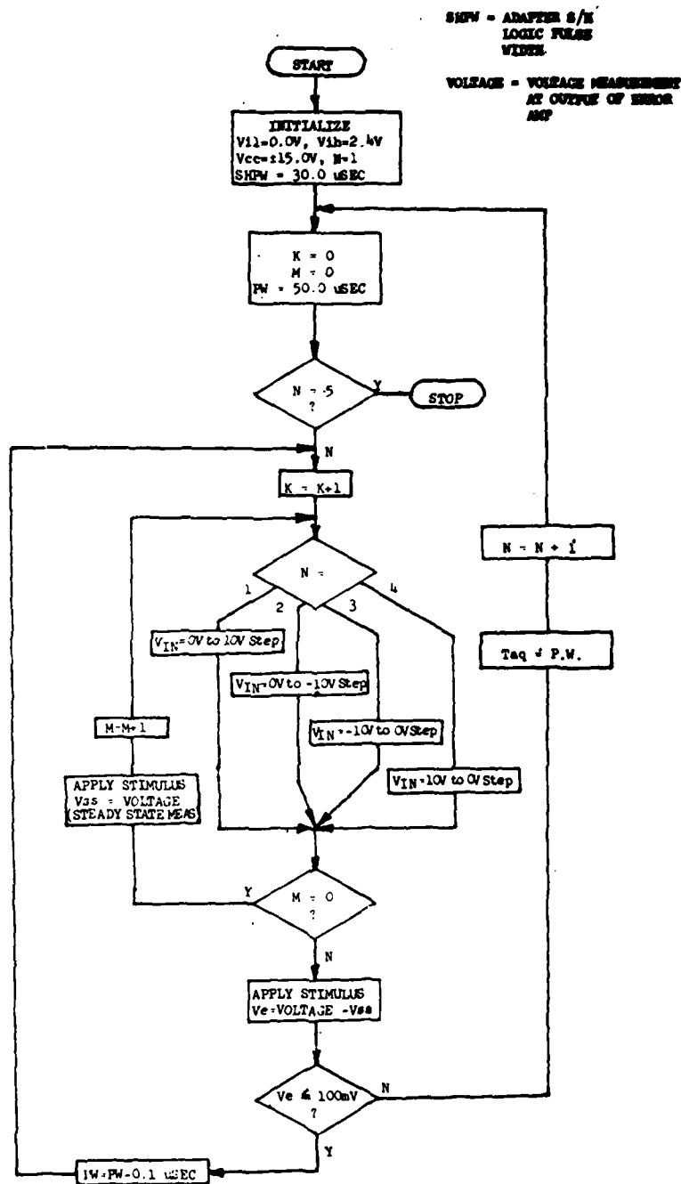
Figure 5-7. Acquisition Time Flow Chart
