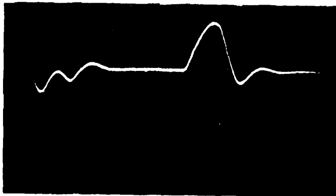
Figure 12-8 Oscilloscope of LM137H Line Transient Response Test
