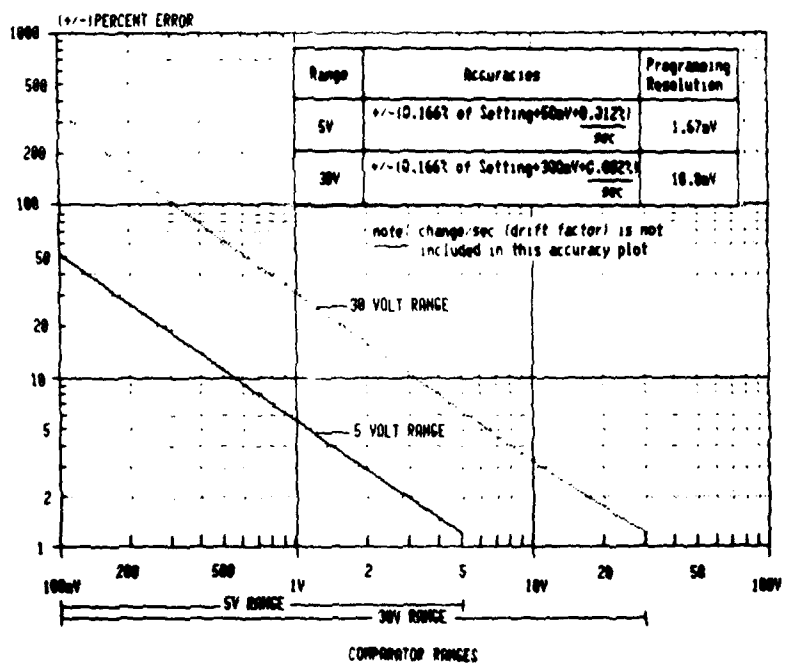
Figure 2-9. S3260/70 - D70 Pin Electronics Card Accuracies
