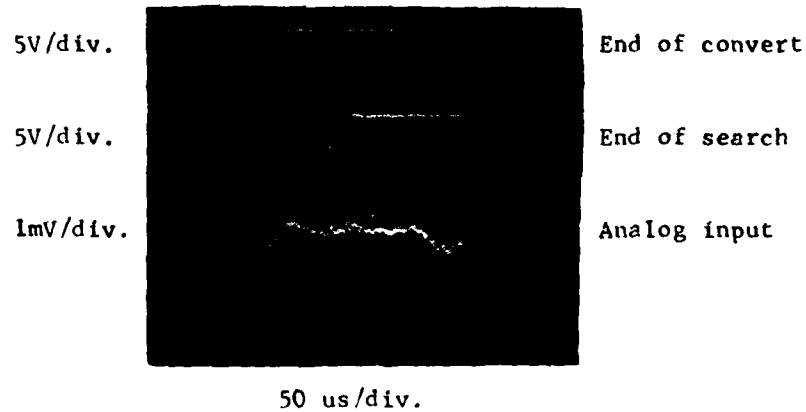
Figure 9-22. DUT Analog Input Voltage During Search Mode
