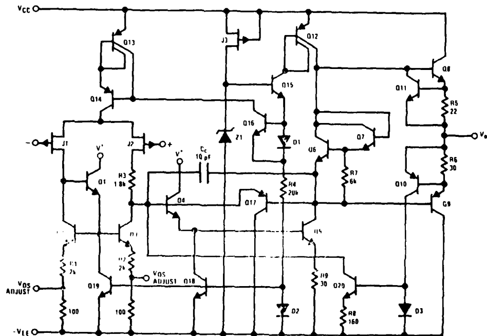
Figure 4-4. LF151, 153, 147 Op Amp Schematic
