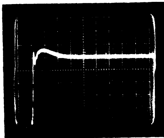
Figure 5-13. LF198 Transient Response vs Manufacturer and Hold Capacitor Size.
