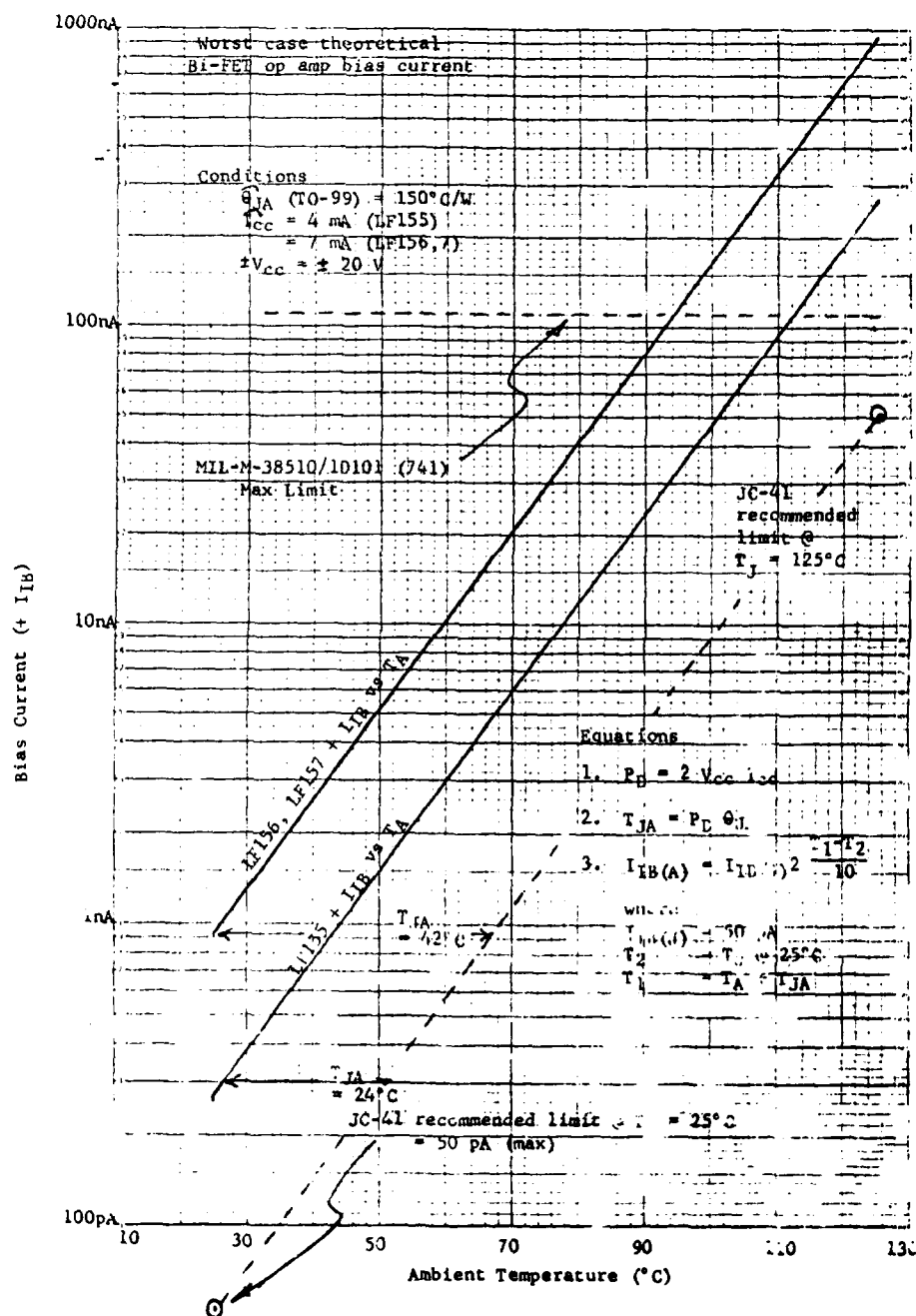
Figure 3-12. Worst Case Input Bias Current vs. Ambient Temperature.
