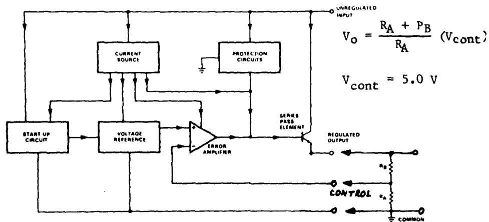
Figure 10-1. Block Diagram of 4-Terminal Adjustable Positive Voltage Regulators.)
