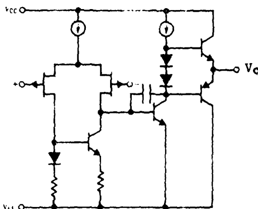
Figure 4-1. BI-FET Op Amp Simplified Schematic.
