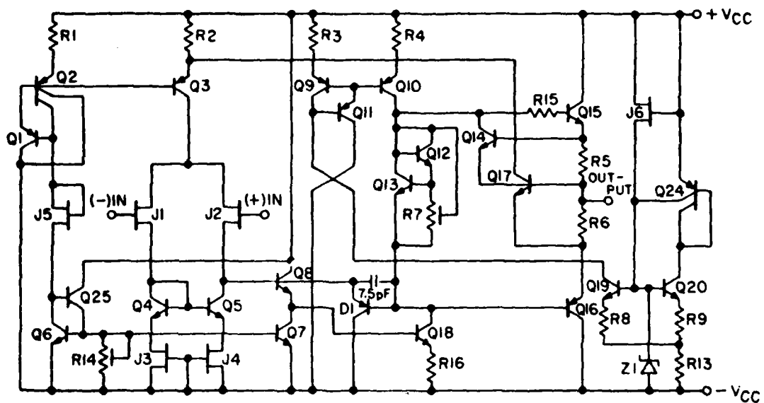
Figure 4-3. TL061 Series Op Amp Schematic
