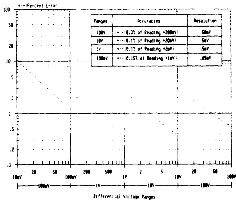
Figure 2-2. S3260/70 - Differential Voltage Accuracies
