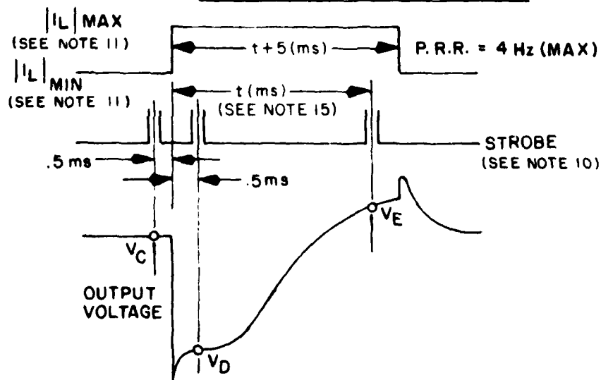
Figure 11-3. Test circuit for static tests for device types 05 and 06. (cont'd)
