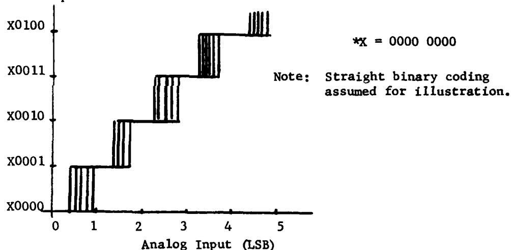
Figure 9-6. Transition uncertainty due to noise.
