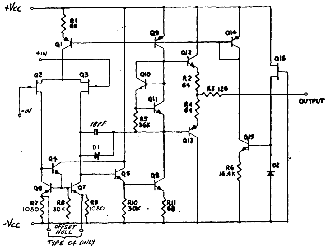
Figure 4-2. TL071 Series Op Amp Schematic.
