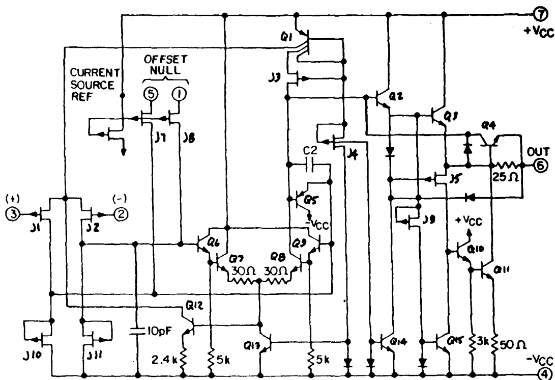
Figure 3-1. Typical BI-BET Op Amp Schematic (LF155/156/157)
