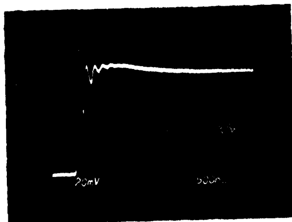
Figure 5-14. LF198 Transient Response vs Common Mode Voltage.
