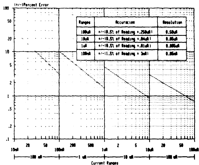
Figure 2-4. S3260/70 - Current Measurement Accuracies
