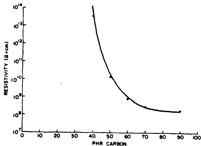
Fig. 7.1 - Resistivity of Neoprene GRT vs concentration of SRF black
