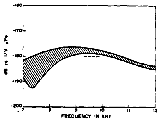
Fig. 14.4 - Free-Field Voltage Sensitivity. Shaded area includes all combinations of sensitivities over a range of temperatures and hydrostatic pressures 3 to 30°C and 40 to 6895 kPa (4 to 700 m). Dashed line indicates minimum sensitivity level between 9.3 and 9.9 kHz.
