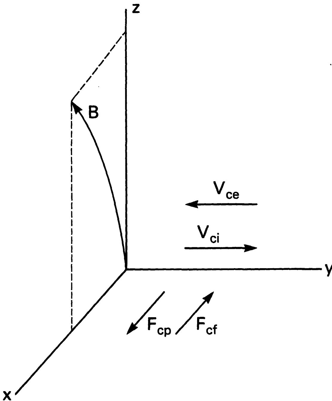
Fig. 1 — Slab geometry used in the analysis with B = B_x \hat{e}_x + B_z \hat{e}_z . Here, F_{cp} is the centripetal force, F_{cf} is the centrifugal force and \bar{V}_{c\alpha} is the curvature drift of species \alpha .
