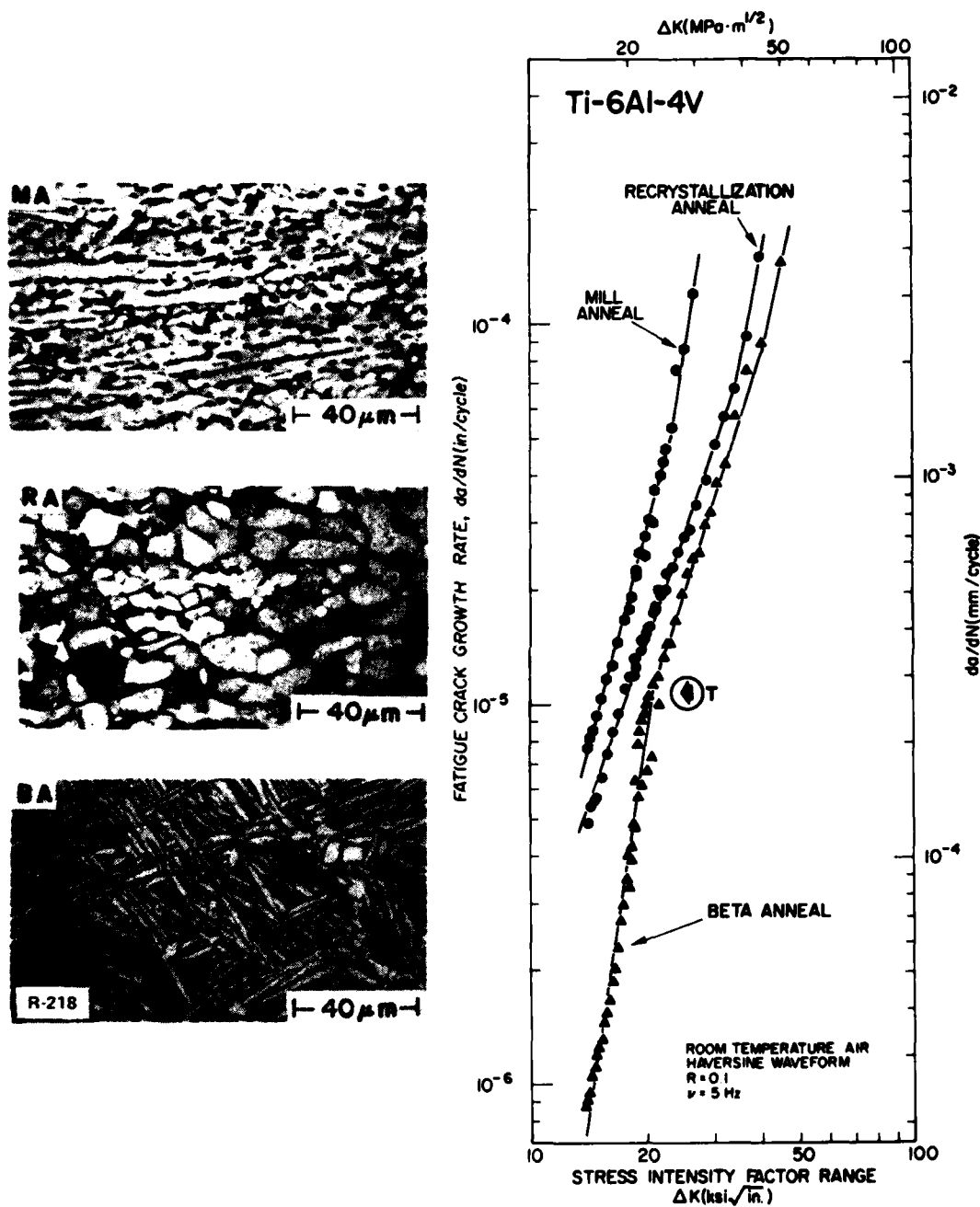
Fig. 2 — Microstructures and fatigue crack growth characteristics in an ambient air environment for the Ti-6Al-4V materials
