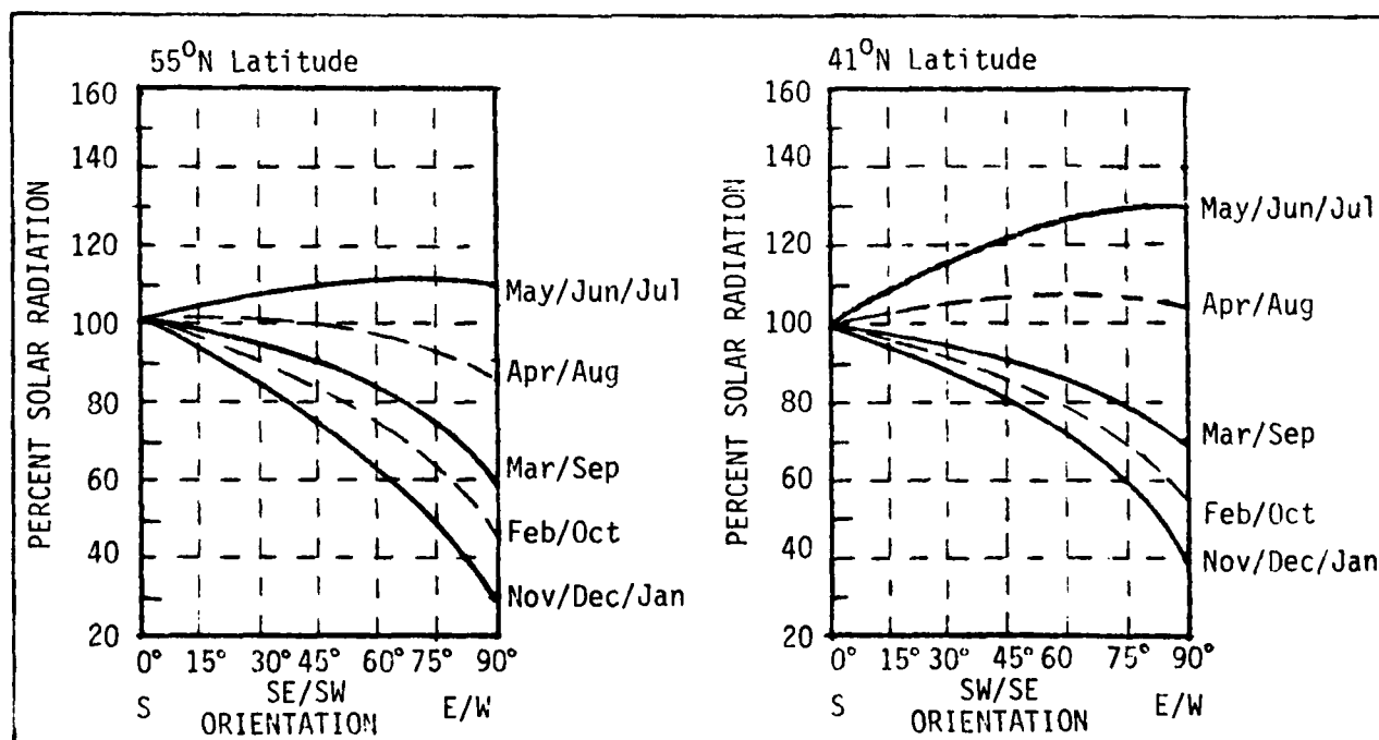
Figure 5.5 Percent of Average Solar Radiation Received on Vertical Walls Deviating from True South at 41^{\circ} and 55^{\circ}\text{N} Latitude (Ref. [12])
