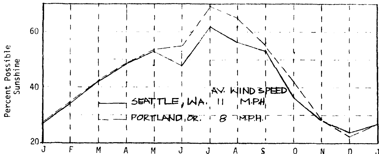
Figure 5.1 Mean Percent Sunshine Possible in Pacific Northwest Locations (averaged from data in Reference [13]).
