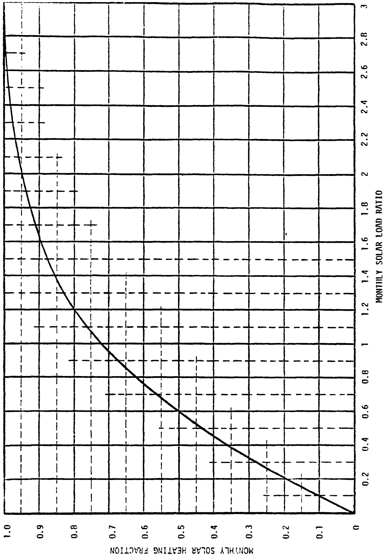
Figure 5.7 Monthly Passive Solar Heating Estimator
