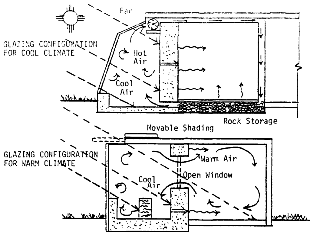
Figure 2.4 Heating of Living Space with Solar Greenhouse
