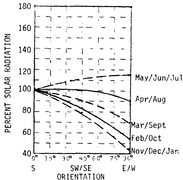
Figure 5.5 Percent of Average Solar Radiation Received on Vertical Walls Deviating from True South at Bremerton, Washington (Ref. [12])
