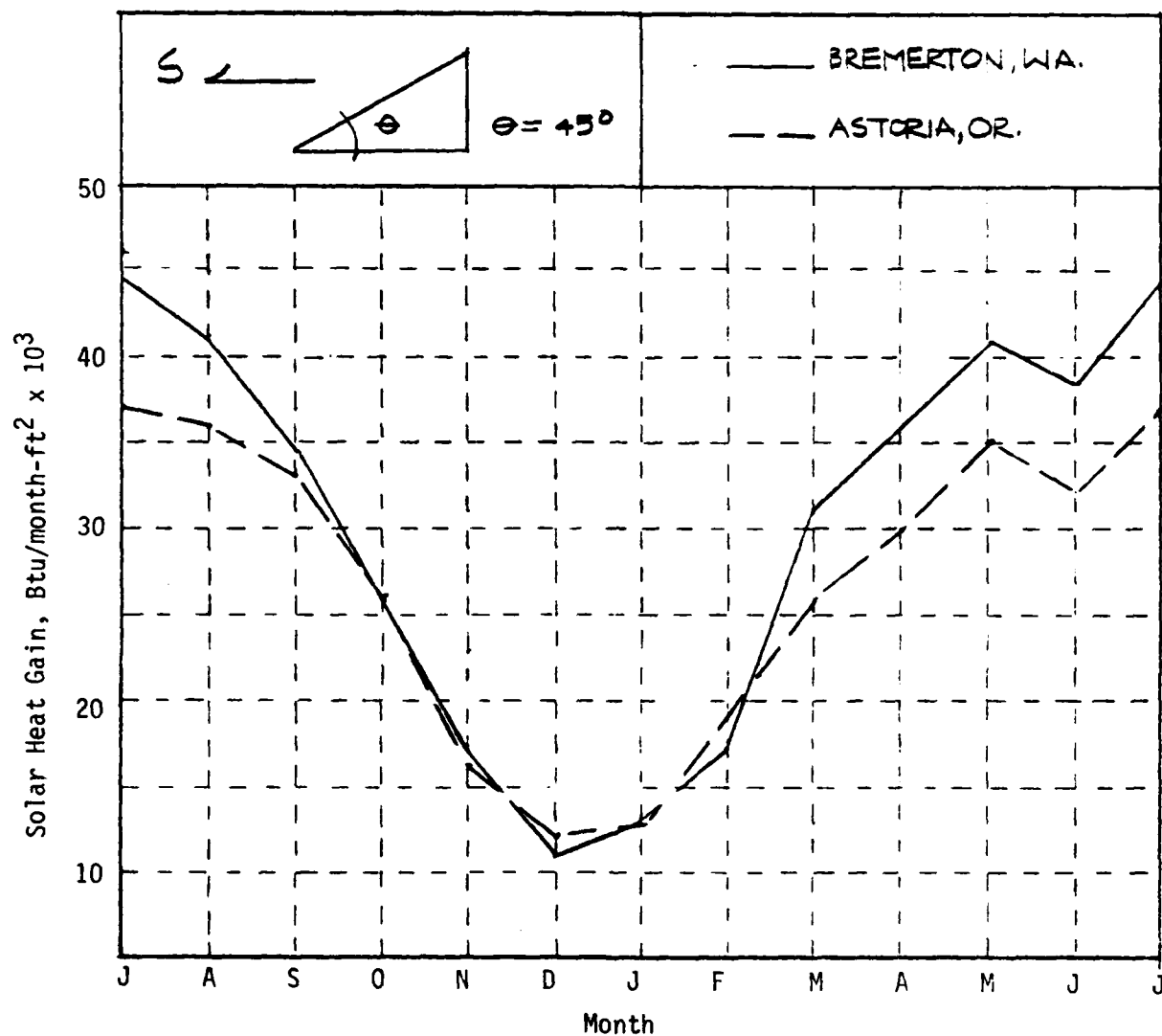
Figure 5.3 Monthly Average Solar Heat Gain Through South-Facing Single Glazing at 45° Tilt (Pacific Northwest)
