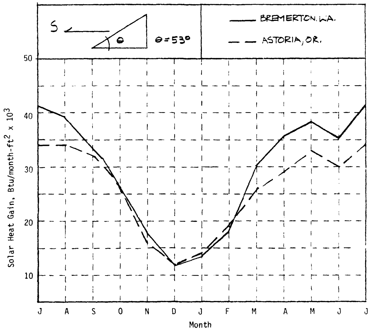
Figure 5.4 Monthly Average Solar Heat Gain Through South-Facing Single Glazing at 53° Tilt (Pacific Northwest)
