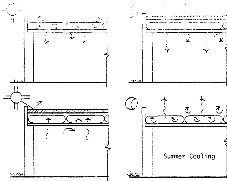
Figure 2.6 The Roof Pond in Warm Climate
