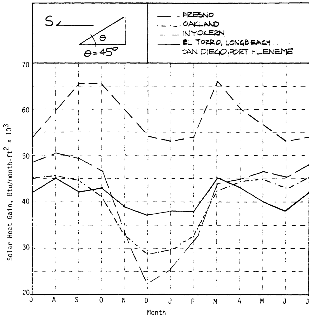
Figure 5.3 Monthly Average Solar Heat Gain Through South-Facing Single Glazing at 45^\circ Tilt (California)
