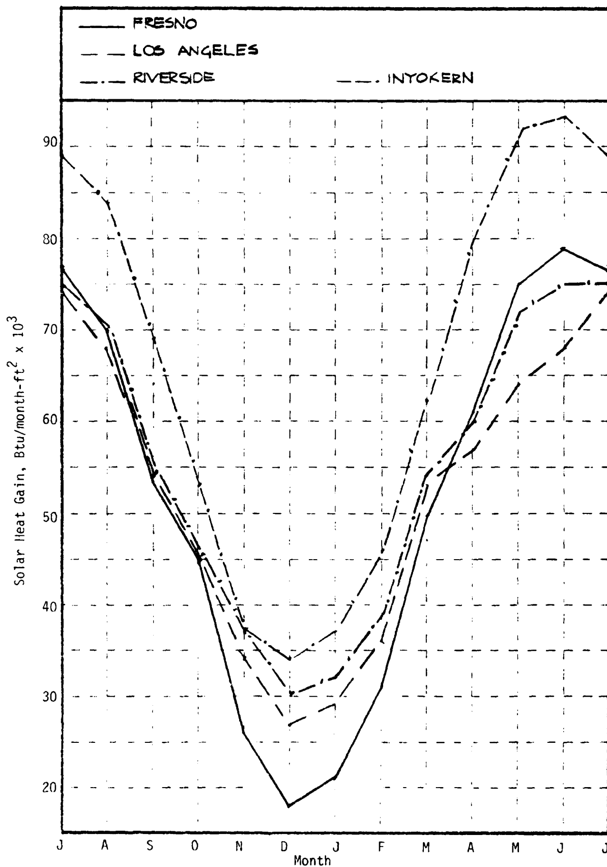
Figure 5.4 Monthly Average Solar Radiation on a Horizontal Surface (Warm California Location)
