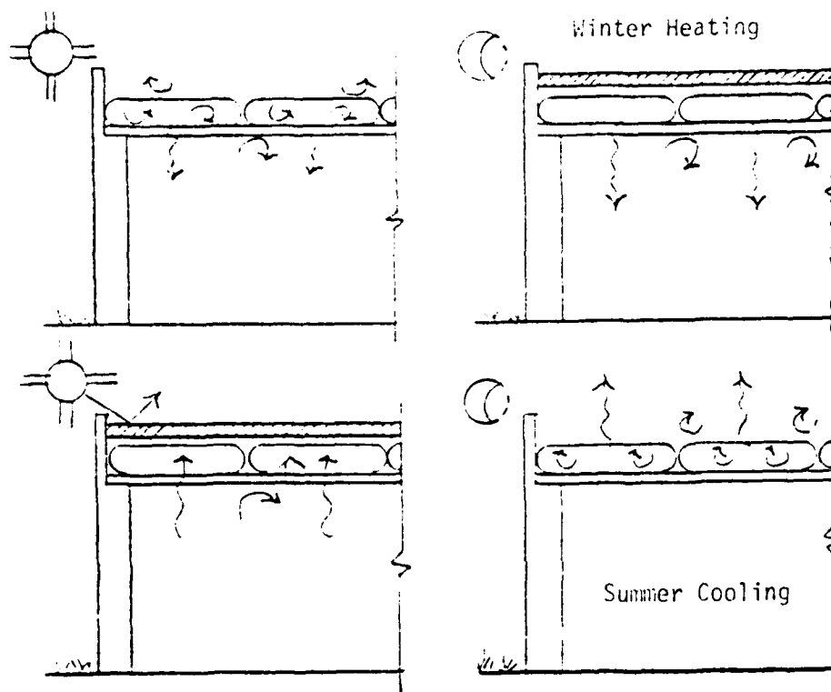
Figure 2.6 The Roof Pond in Warm Climate
