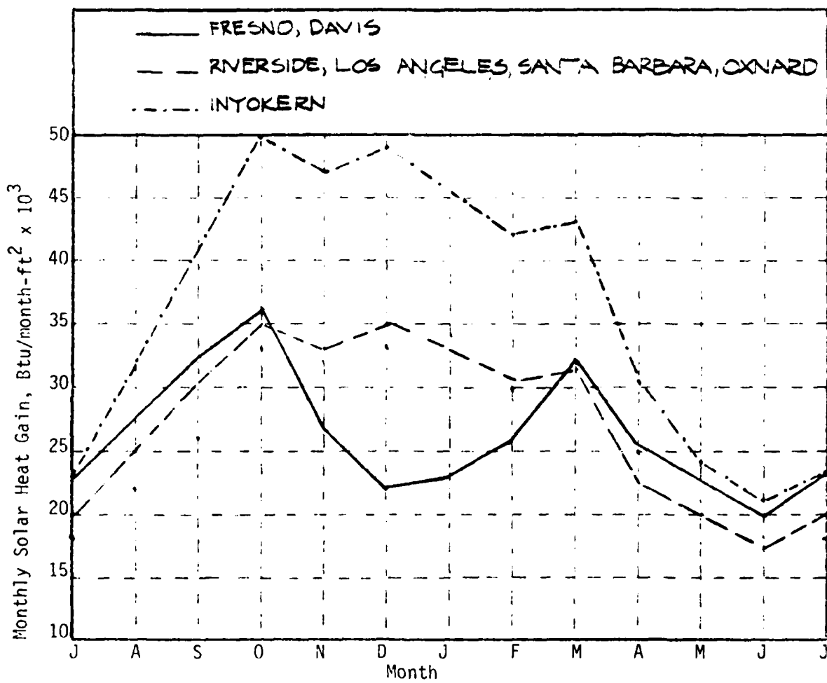
Figure 5.2 Monthly Average Solar Heat Gain Through Vertical South-Facing Single Glazing (California Locations)
