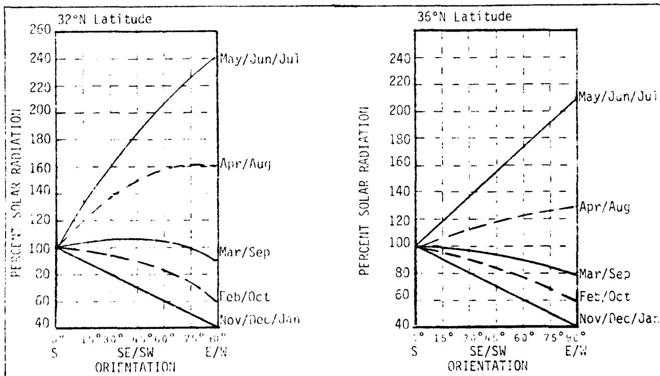
Figure 5.5 Percent of Maximum Solar Radiation Received on Vertical Walls Deviating from true South at 32° and 36° N Latitude (Ref. [6])
