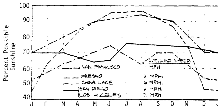
Figure 5.1 Mean Percent Sunshine Possible in Warm California Climatic Regions (averaged from data in Reference [13]).
