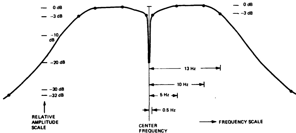
Figure 3-2. System Bandwidth
