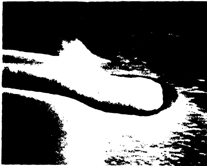
Figure 2-26 SEM photograph of gate finger end, FET R-5 at 18,000X. Estimate 500-1000Å of CR, overlaid by 4500-5000Å of Au.
