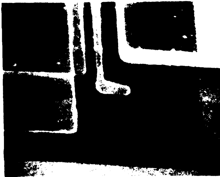
Figure 2-8 FET D-2. (a) 4400X view of gate metal after attempted removal of glass with buffered HF. Two layers are glass and gate metal. (b) Gate finger end, 4100X. Gate length, 0.8 \mu\text{m} ; S-D spacing, 4.0 \mu\text{m} . Glass removed from ohmic contact.
