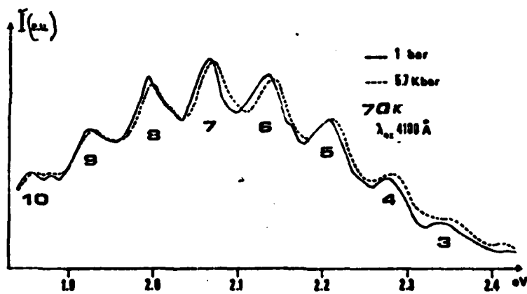
Figure 1 : Scapolite emission spectrum 3, 4, ... = n = vibronic component number
