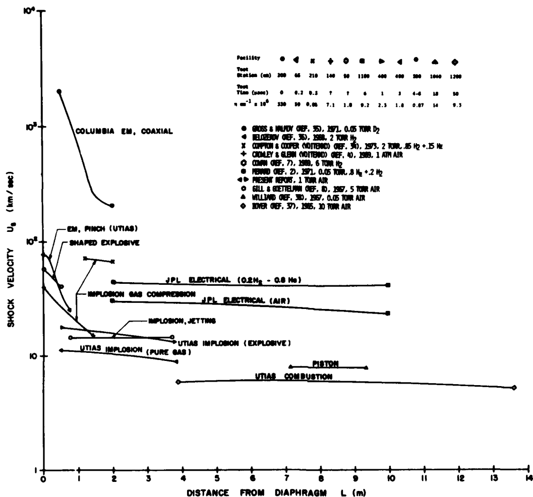
FIG. 23 COMPARISON OF HYPERVELOCITY SHOCK WAVES PRODUCED BY EXPLOSIVE-DRIVEN IMPLOSIONS WITH OTHER FACILITIES.
