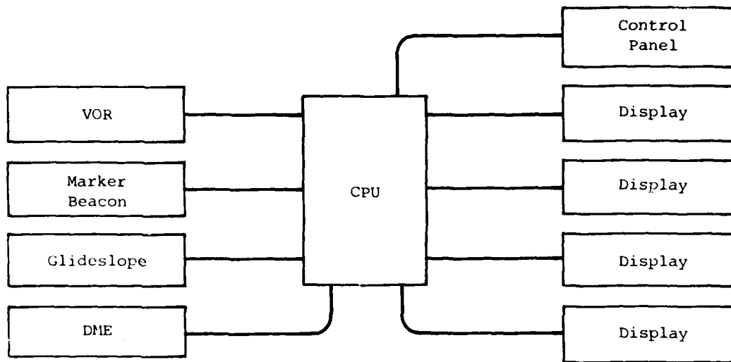
Figure 4-8. CENTRALIZED ARCHITECTURE
