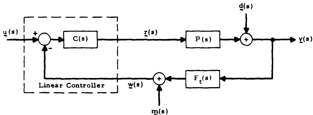
Fig. 2: The classical single-loop servo-regulator configuration
