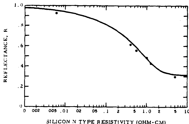
Fig. 3 The reflectance R as a function of resistivity \rho . The points are measured, and the solid line is the theoretical prediction based on the Drude model.
