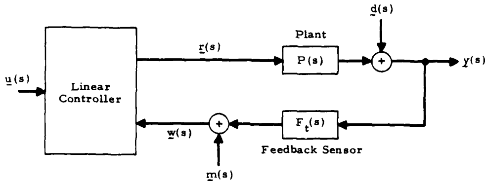
Fig. 1: General multivariable servo-regulator configuration
