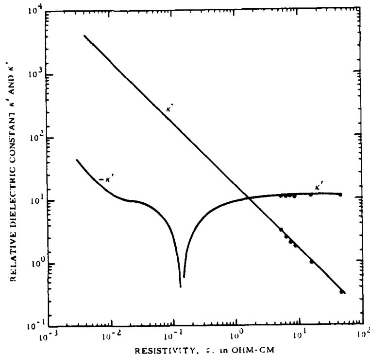
Fig. 2 The real and imaginary parts, \kappa' and \kappa'' , of the relative permittivity as a function of resistivity \rho . The points are measured and the solid line is the theoretical prediction based on the Drude model.
