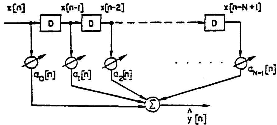
Fig. 1. Adaptive estimator.
