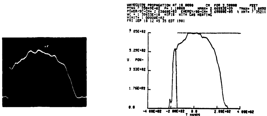
Fig. 3b Comparison of experiment with computer model results for propagation of a 3-GHz, 50-kW 400-ns microwave pulse in a partially evacuated waveguide.
