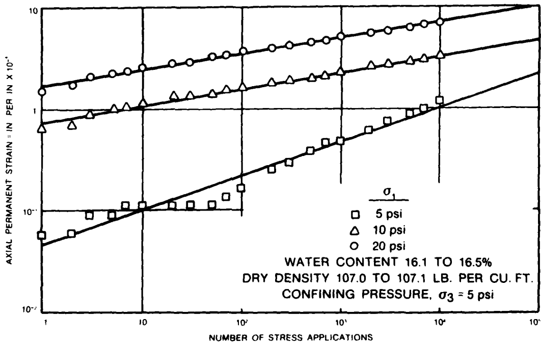
Figure 6. Axial permanent strain versus number of load applications, experimental data and statistical relationship (1 in. = 2.54 cm; 1 psi = 6.89 kPa; 1 lb/cu ft = 16.02 kg/m 3 )
