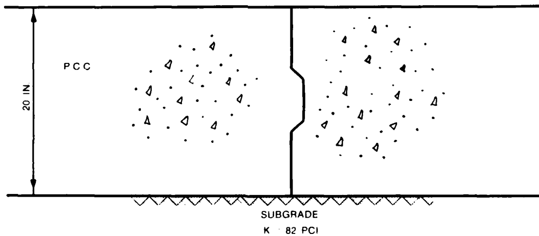
Figure 13. Rigid pavement design (1 in. = 2.54 cm; 1 \text{ pci} = 2.77 \times 10^4 \text{ kg/m}^3 )
