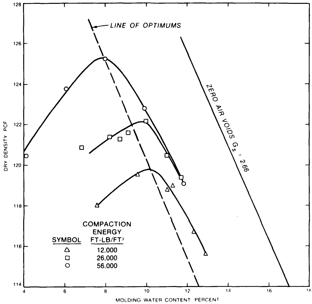
Figure 11. Moisture-density relations for silty sand (1 pcf = 16.02 kg/m 3 ; 1 ft-lb/ft 3 = 0.48 kJ/m 3 )
