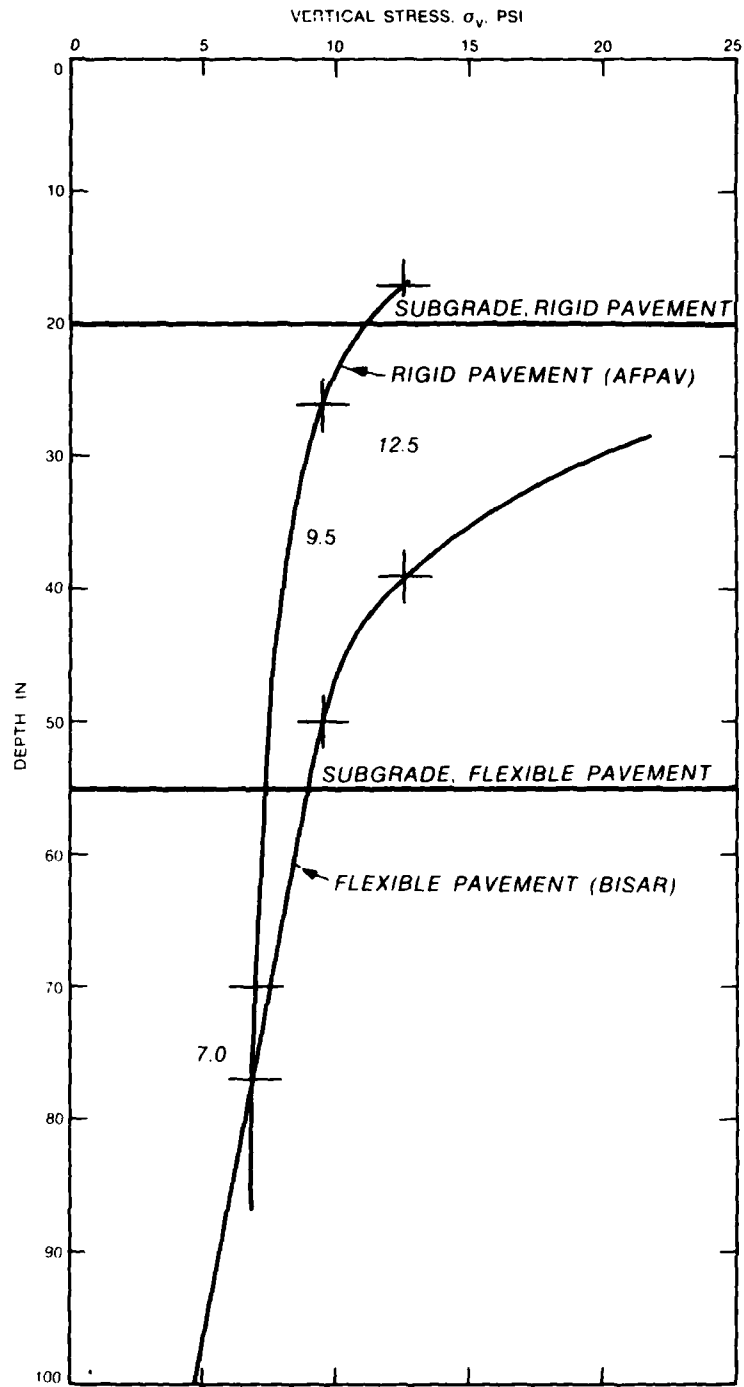
Figure 16. Vertical stress-depth relation for flexible and rigid pavements (1 in. = 2.54 cm; 1 psi = 6.89 kPa)
