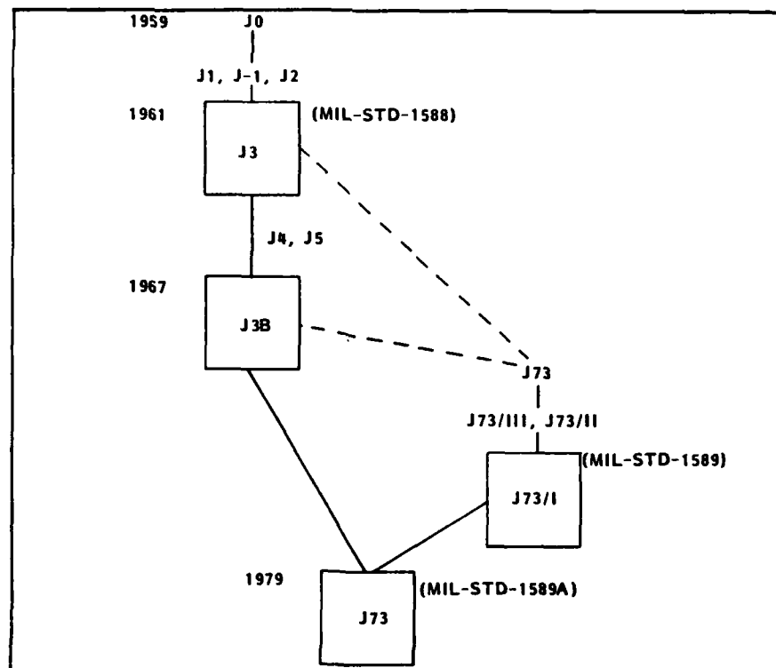
Figure 1-1. The JOVIAL Language Family
