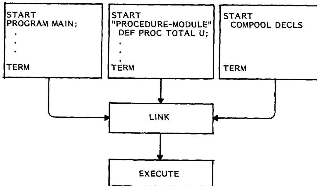
Figure 4-1. A Complete Program
