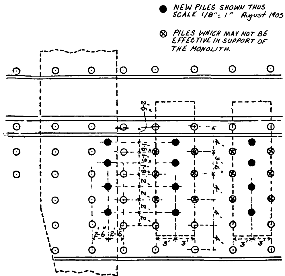
Figure 40. Plan view, south end of dam, showing location of piles
