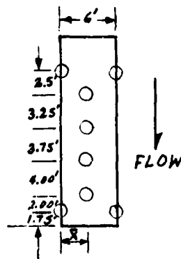
Figure 61. Moment of inertia of pile group (8 piles)
