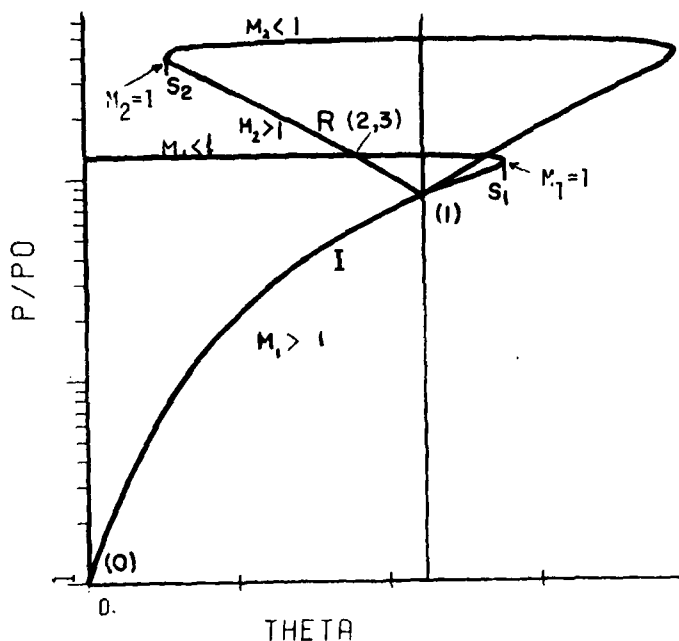
FIG. 18 DOUBLE MACH REFLECTION.
