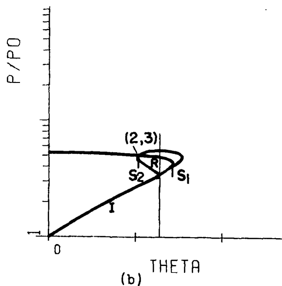
FIG. 8 SINGLE MACH REFLECTION. (a) PHYSICAL PLANE (SCHEMATIC), (b) \theta -P SHOCK POLAR DIAGRAM.
