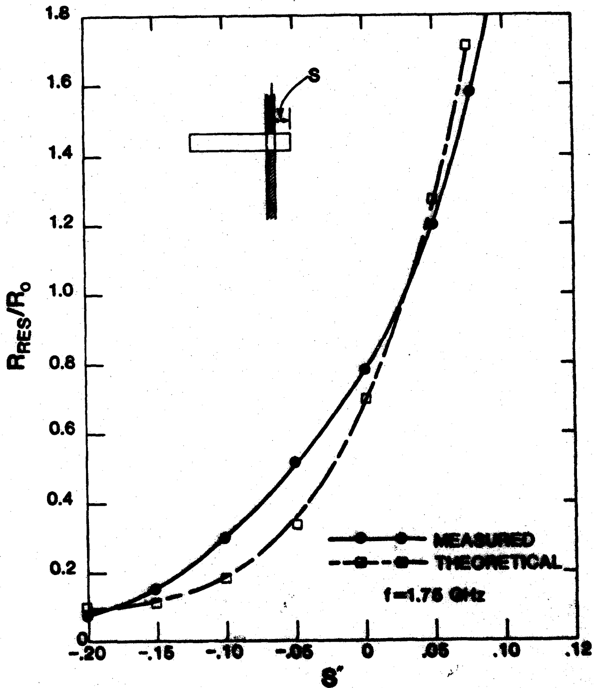
FIGURE 2.5 Normalized resonant slot resistance vs. offset.
