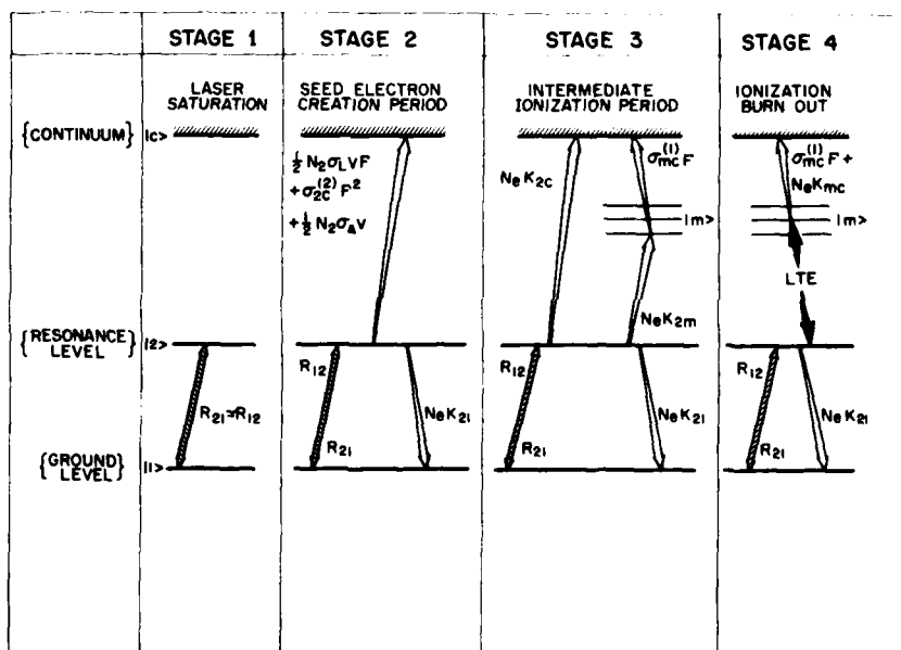
FIG. 1. Four stages of laser ionization based on resonance saturation. STAGE 1. Laser rapidly locks ground and resonance level populations in ratio of degeneracies. STAGE 2. (i) Rapid growth of free electrons due to two-photon ionization of resonance level and laser-induced Penning ionization. Associative ionization is important for some elements. (ii) Free electrons rapidly gain energy through superelastic collisions. STAGE 3. (i) Direct electron impact ionization of resonance level and single-photon ionization of collisionally populated upper levels dominate the rate of ionization. (ii) Electron temperature stabilizes as the rate of superelastic heating balances rate of collisional cooling through excitation. STAGE 4. (i) Runaway collisional ionization of upper levels occurs once a critical electron density achieved. (ii) Superelastic heating can no longer balance collisional cooling and electron temperature falls.
