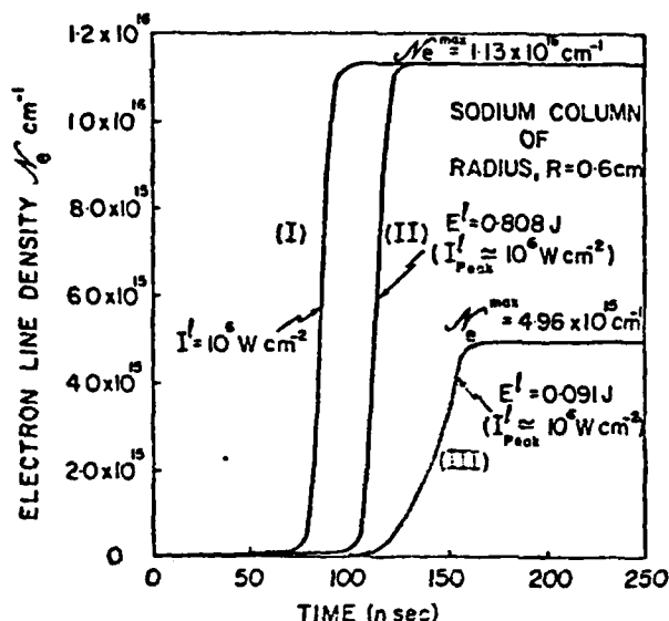
FIG. 6. Comparison of the temporal variation of the free electron line density, N_e , in a sodium column evaluated to a radius of 0.6 cm for the three cases. (I) Steplike, flat laser pulse for I^l = 10^6 \text{ W cm}^{-2} . (II) Laser pulse is assumed to have realistic temporal variation, Eq. (35) of text, but uniform radial distribution out to 0.6 cm. Energy of the pulse is set to be 0.808 J corresponding to a peak irradiance of 10^6 \text{ W cm}^{-2} . (III) Laser pulse is assumed to have both a realistic temporal variation, Eq. (35), and a Gaussian radial distribution with an exponential radius of 0.20 cm and an energy of 0.091 J, giving a peak irradiance of 10^6 \text{ W cm}^{-2} .
