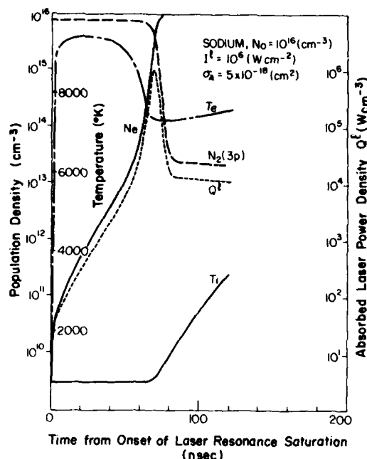
FIG. 8. Time histories of N_0 , T_e , N_2 , Q^I and T_1 as predicted by the full LIBORS computer code (Refs. 15 to 18) for sodium with an original density of 10^{16} \text{ cm}^{-3} and a laser irradiance I^I = 10^6 \text{ W cm}^{-2} .
