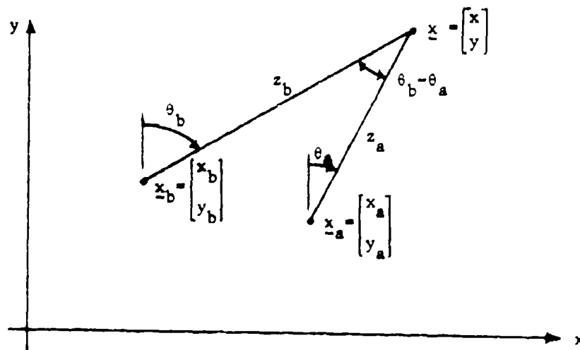
Figure 1. Geometry of a Planar Range Navigation System
