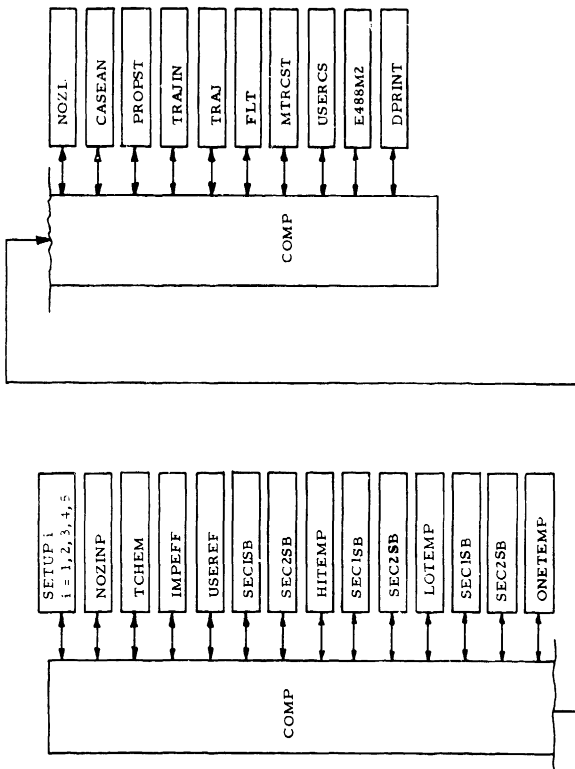
Figure 6. Subroutine COMP
