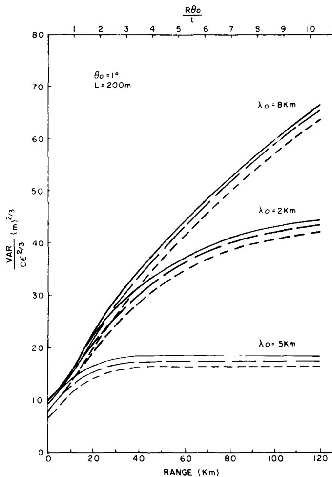
Figure 5b. Doppler Spectrum Variance (VAR) Normalized to C\epsilon^{2/3} Versus Radar Range, Turbulence Outer Scale Lengths are \lambda_0 = 0.5, 2, 8 km. Full half-power beamwidth is 1^\circ and pulse volume depth is 200 m. Ratio of pulse volume width to depth ratio at top
