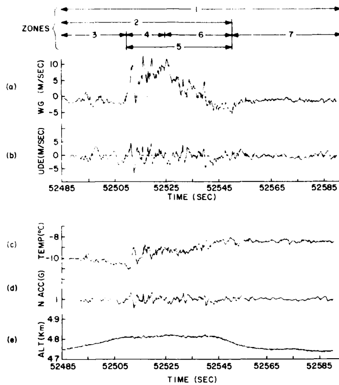
Figure 8. Aircraft Time Series Data for Early Aircraft Run of (a) Vertical Gust Velocity, (b) Derived Gust Velocity, (c) Environmental Temperature, (d) Normal Acceleration, (e) Barometric Altitude. Analyzed segments are labeled 1 through 7
