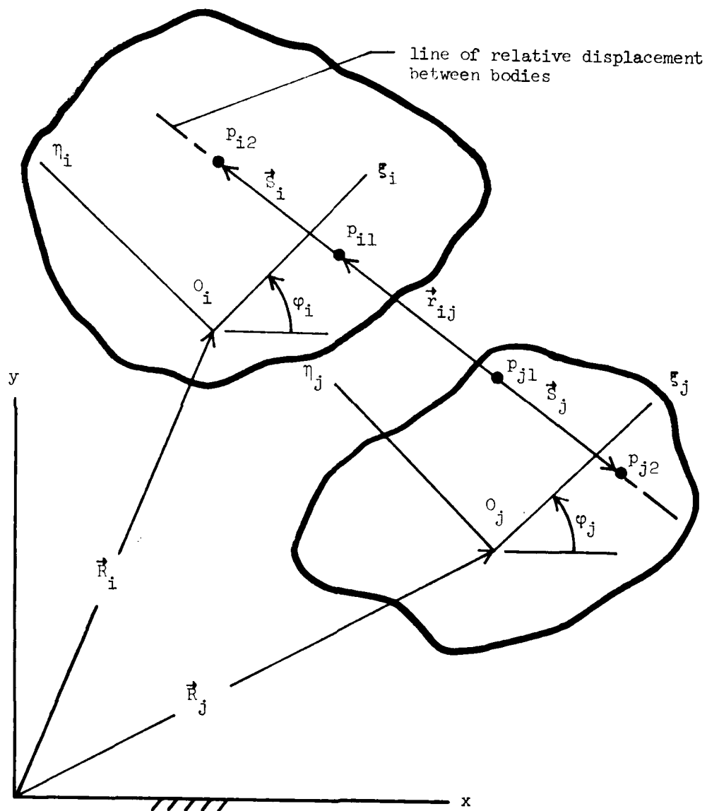
Figure 2.2. Rigid bodies connected by a translational joint.
