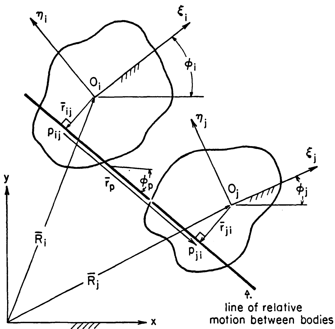
Figure 2.3 Translational Joint
