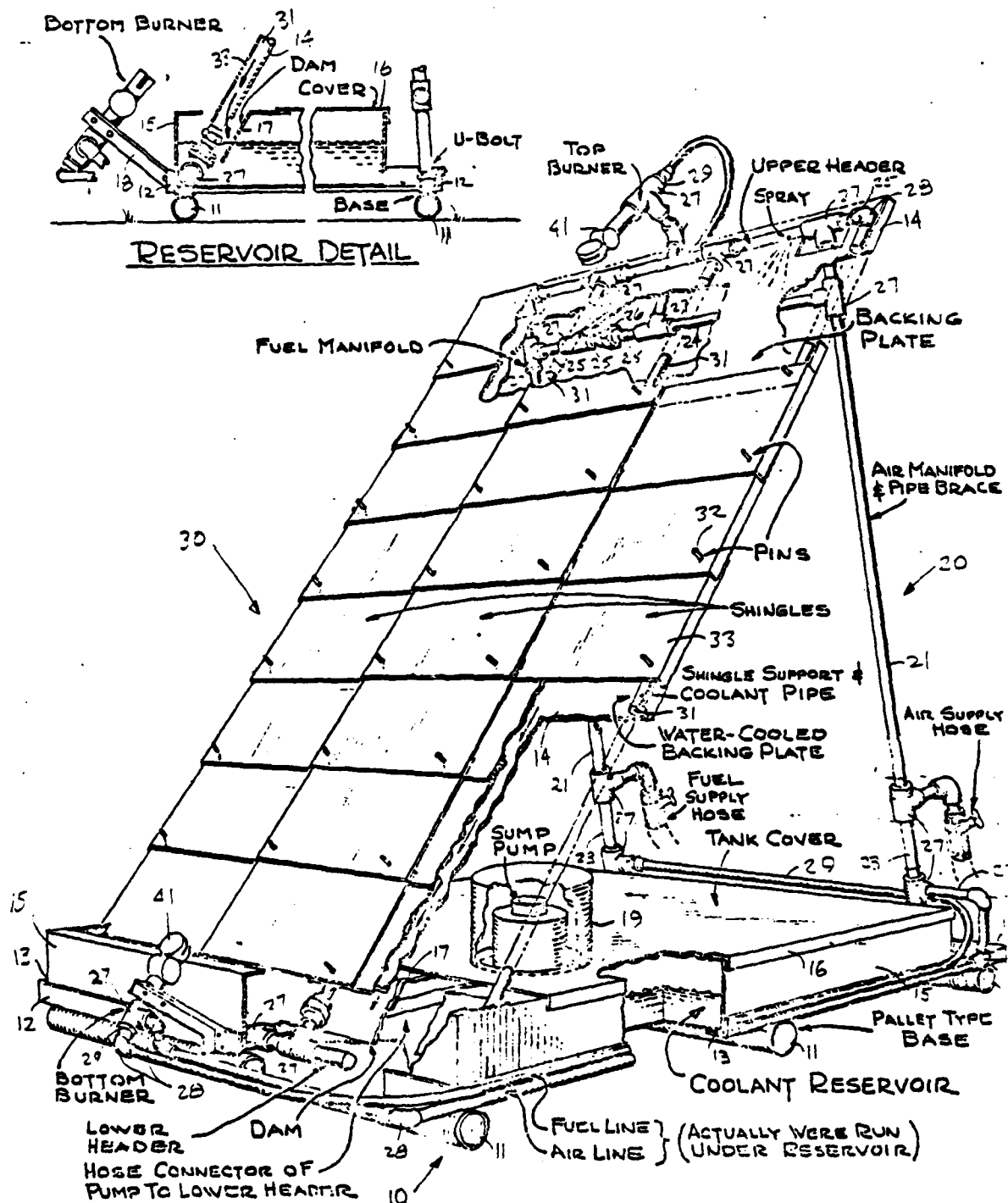
Fig. 2 - SMOKELESS CASCADE FIRE TEST DEVICE
