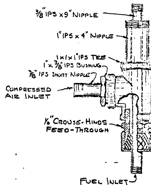
BURNER ADAPTOR
