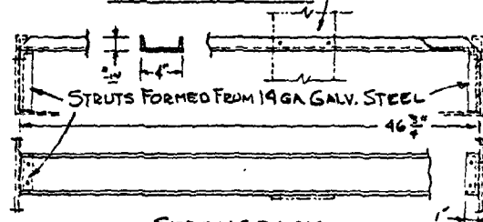
STRONGBACK
