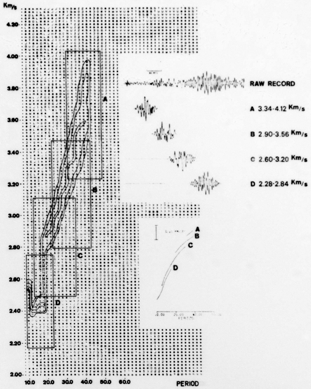
Figure 5. Analysis process for reducing a raw seismogram to a final phase velocity curve. The first step is to identify group arrival times for the mode and period range of interest (boxes A to D). By windowing the record in this manner (records A to D) higher modes or multipathed arrivals can be excluded from the analysis. Finally, phase velocities are computed from the windowed records (curves in the lower right). For clarity these four phase curves have been offset from each other by 0.1 km/s.
