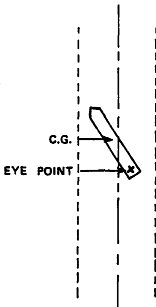
Figure A.11. Effect of Wheelhouse Location when Crabbing in a Channel
