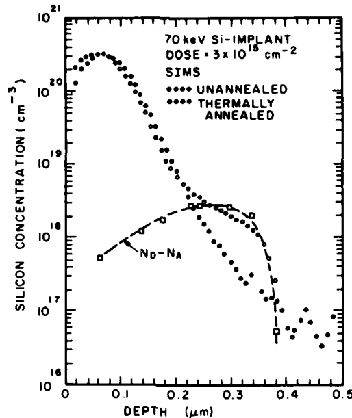
Figure 4. SIMS profile of a Si-implanted GaAs sample before and after thermal annealing, 70 keV, 3 \times 10^{15} \text{ cm}^{-2} .
