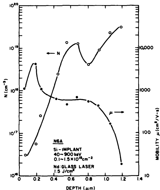
Figure 81. Depth distribution of carrier concentration and mobility of multiple-implanted GaAs; laser-irradiated at 1.5 \text{ J/cm}^2 .
