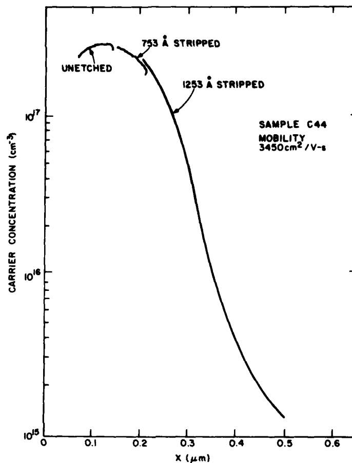
Figure 43. Electron density profile of double-implanted GaAs sample C44.
