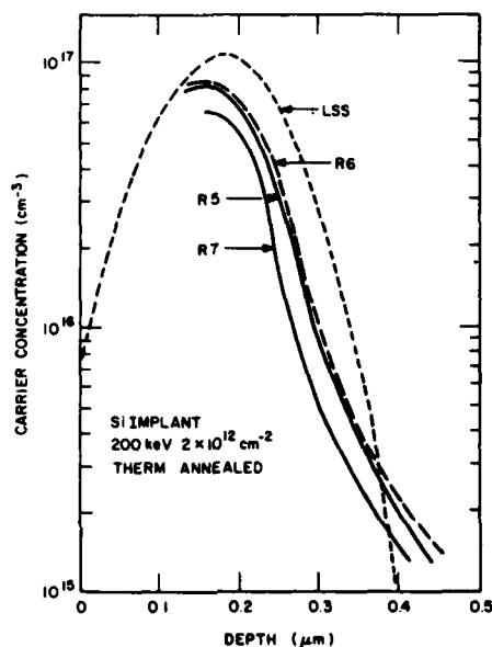
Figure 50. Electron density profiles of R5, R6, and R7, three Si implants in substrates pretreated with ^{40}\text{Ar} implant plus anneal; the ^{40}\text{Ar} doses are 5 \times 10^{12} , 1 \times 10^{13} , and 5 \times 10^{13} \text{ cm}^{-2} , respectively.
