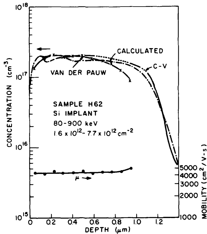
Figure 40. Multiple-implant profiles of H62: calculated and measured. Mobility profile also included.
