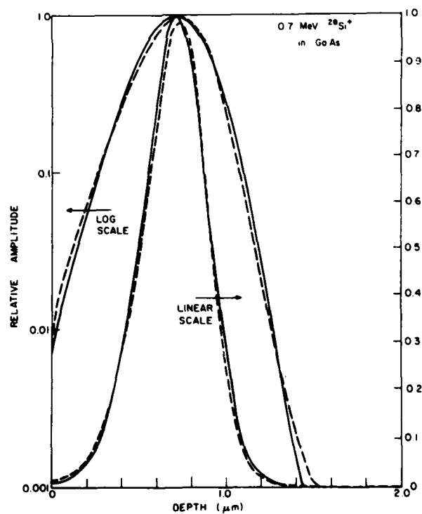
Figure 27. Curve-fitting to experimental data, 0.7-MeV 28 Si + into GaAs.
