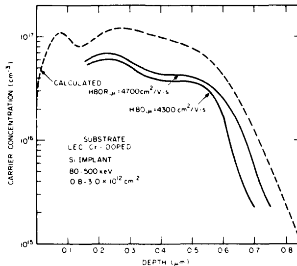
Figure 45. Electron density profiles of multiple Si-implanted n-layers on Si GaAs substrate with (H8OR) and without (H8O) ^{40}\text{Ar} pretreatment. Calculated profile is shown by dashed line.
