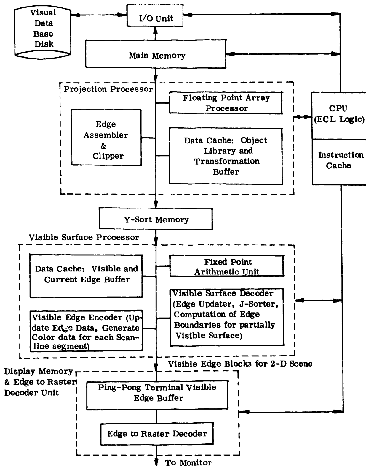
Figure 2.2.1.2.6-1. ATS Computrol System
