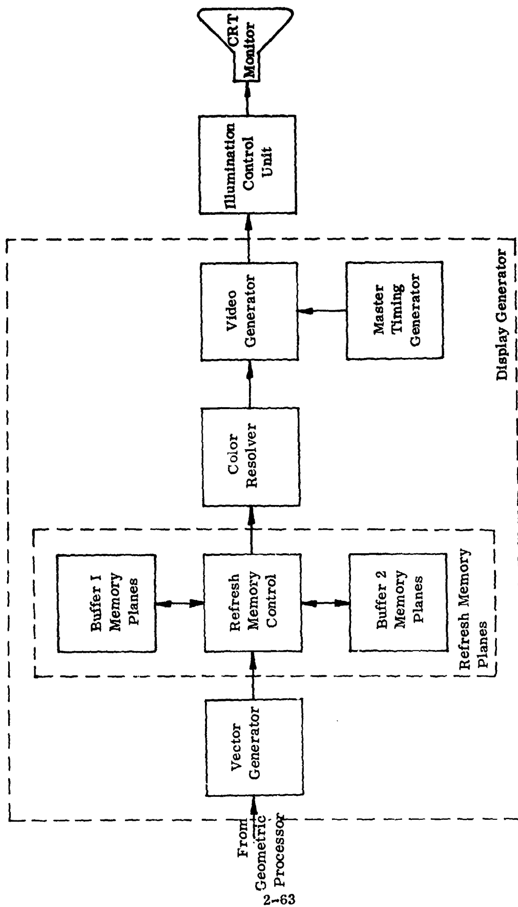
Figure 2.2.1.2.3-lb. Gould GVS-1 System (Part 2)
