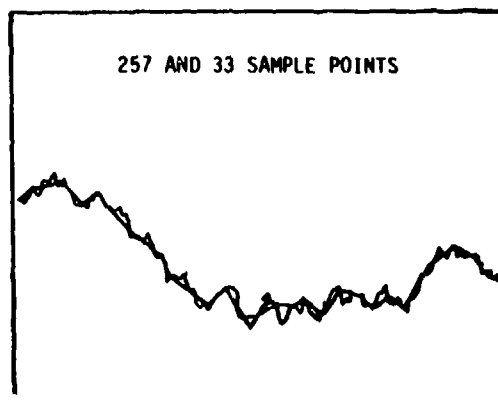
Figure 3.2.4.2-10. Fractal Curves From [Fournier and Fussel, 1980]
