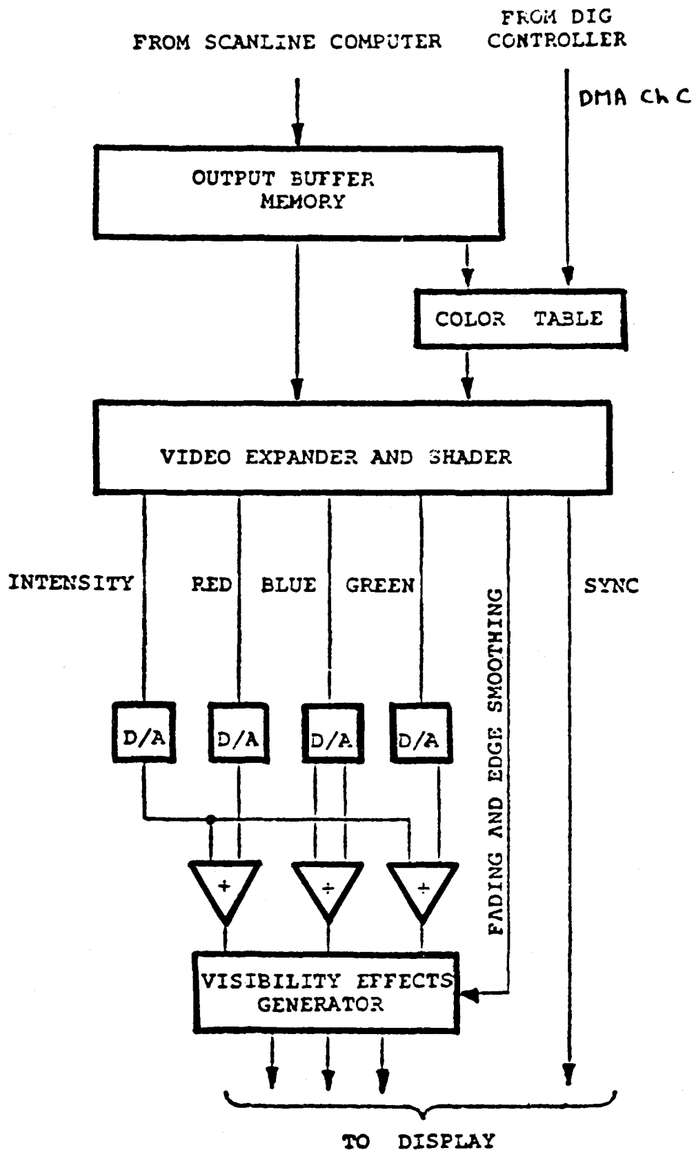
Figure 2.2.1.2.1-7. Output Buffer and Video Generator
