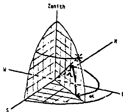
Figure 3.2.3-1. Height Field Illumination by Point Source
