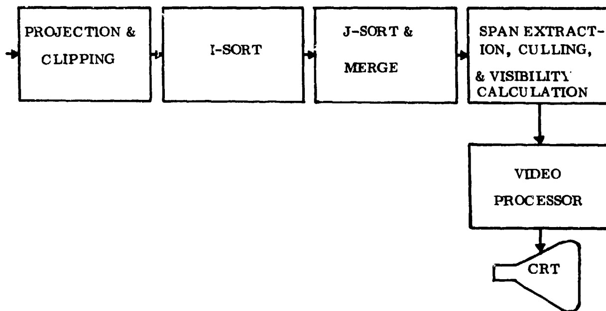
Figure 2.2.1. 1.2-3. Generic Scanline Coherence Processing
