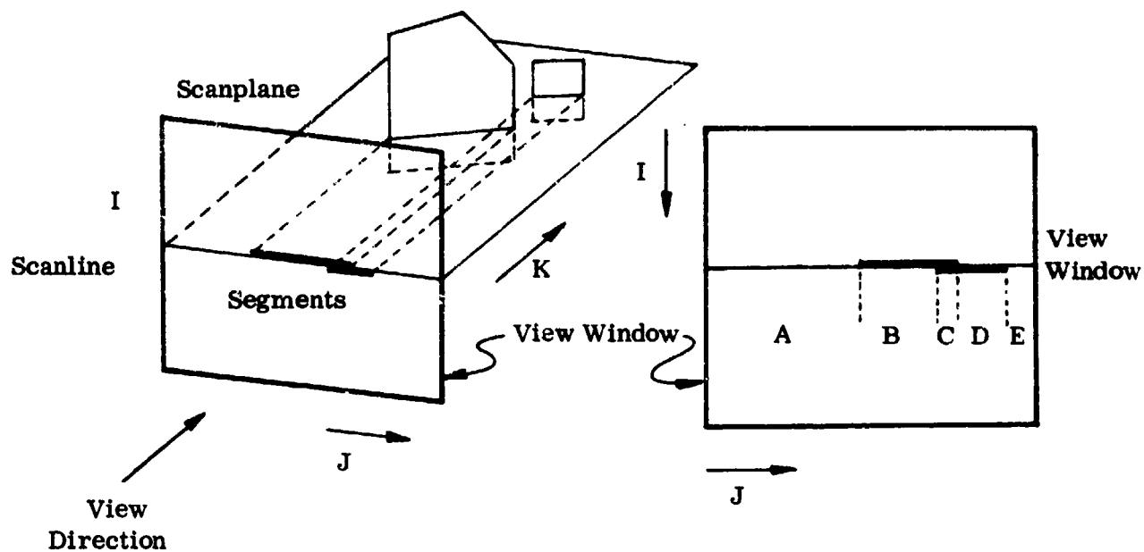
Figure 2.2.1.1.2-1. Scanplane Projection to View Window
