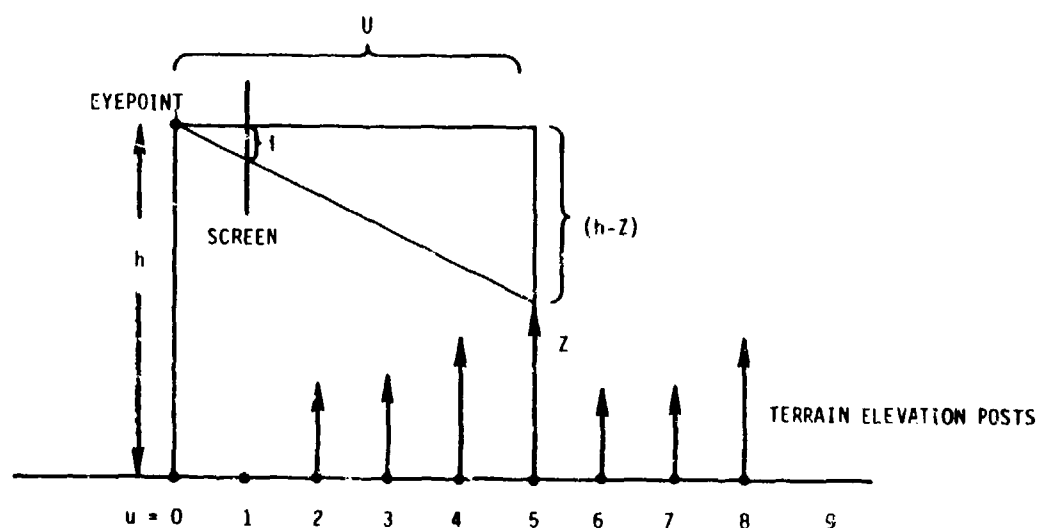
Figure 3.2.4.2-7. Side View of Perspective Screen Projection
