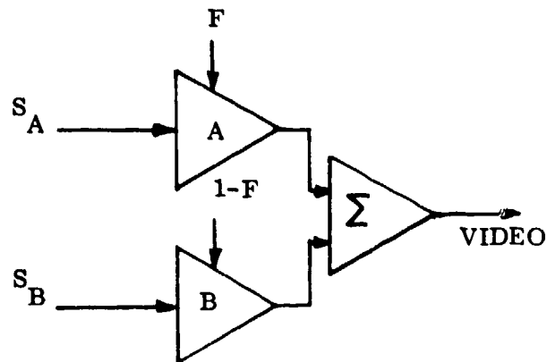
Figure 2.2.1.2.5-2. Variable Gain Amplifiers used for Texture Component Fading
