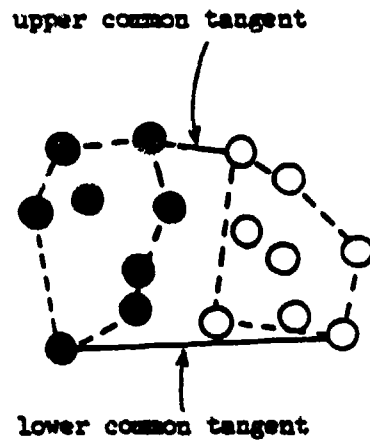
Figure 6 Illustration of the upper and lower common tangents of two convex hulls.
