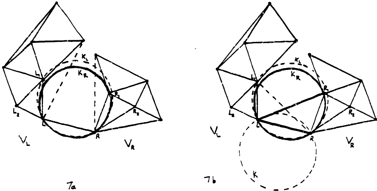
Figure 7 Illustration for the merge process. Solid lines are new Delaunay edges introduced by the MERGE algorithm.
