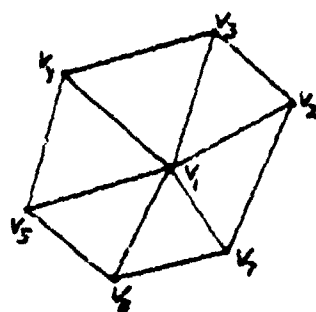
Figure 5 Example illustrating a doubly-linked circular list.
