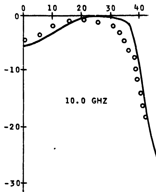
Figure 6-14 Measured and Calculated H-Plane Transmission Characteristics at Various Frequencies
