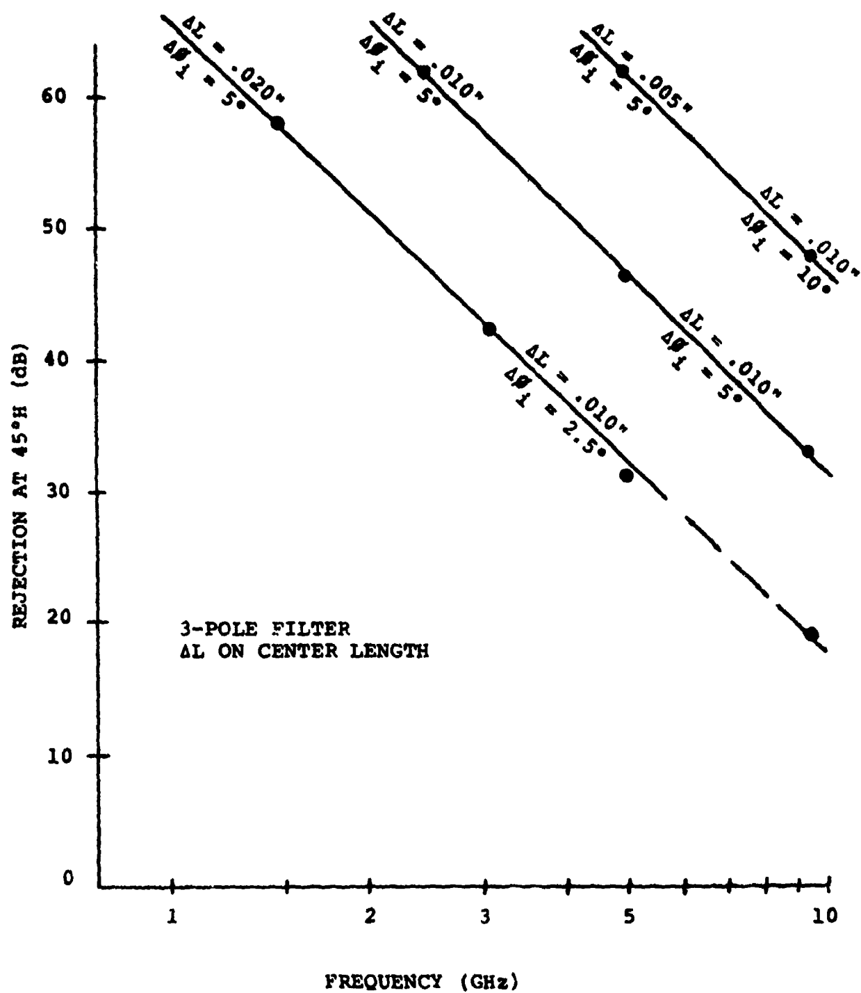
Figure 5-1 Allowable Rejection vs. Frequency
