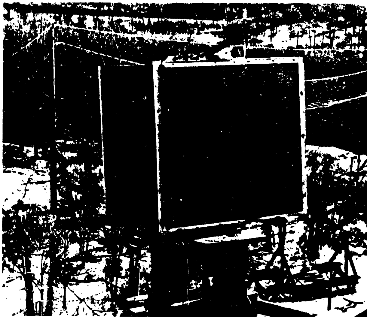
Figure 1-1 Photograph of Spatial Filter in Front of Antenna on Antenna Range
