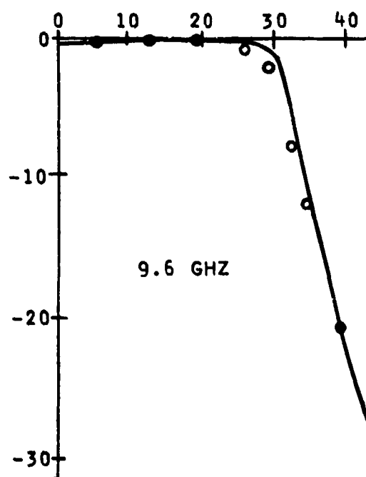
Figure 6-14 Measured and Calculated H-Plane Transmission Characteristics at Various Frequencies
