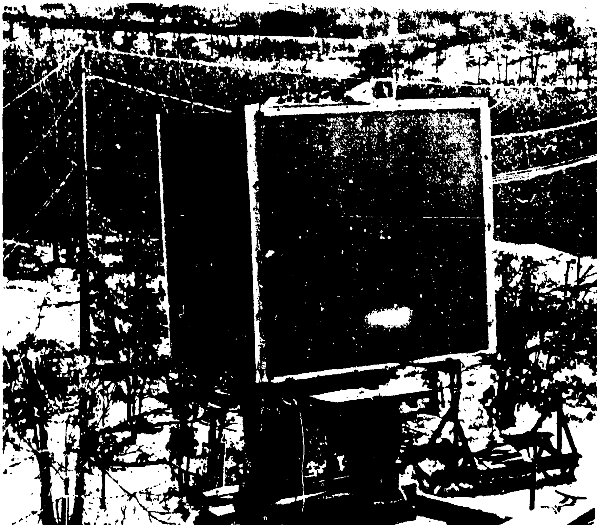
Figure 6-5 Photograph of Spatial Filter on Antenna Range
