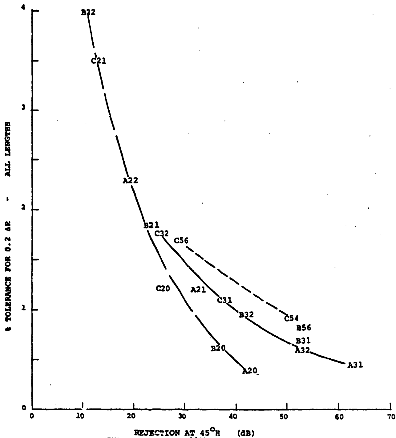
Figure 4-10 Tolerance on All Lengths Cumulative vs. Rejection, for 0.2 \Delta R Allowable
