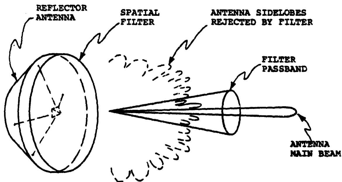
(b) application to reflector antenna
