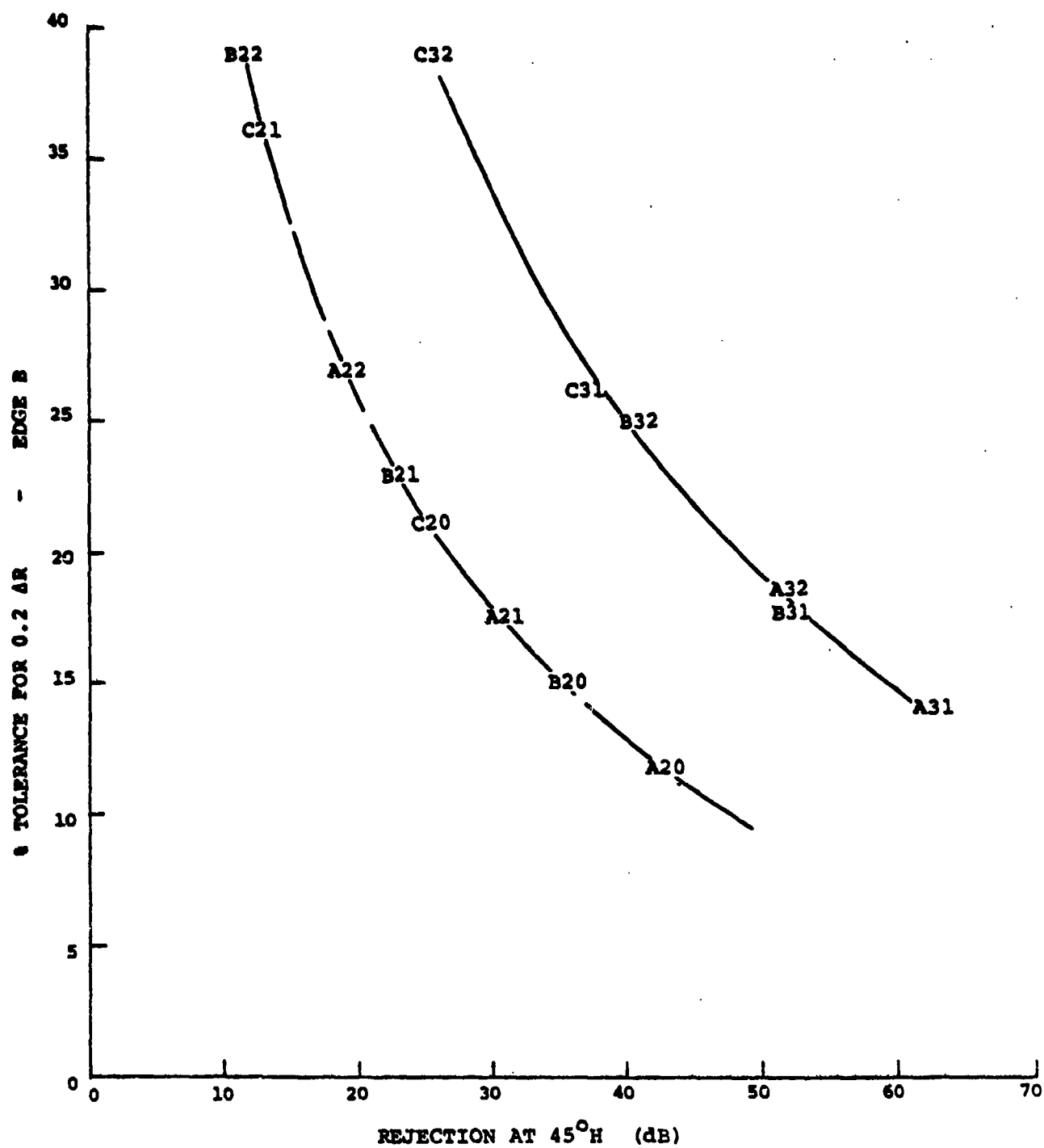
Figure 4-8 Tolerance on Edge Susceptance vs. Rejection, for 0.2 ΔR Allowable
