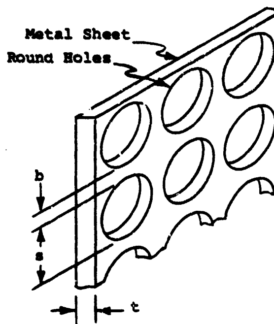
(b) hole configuration
