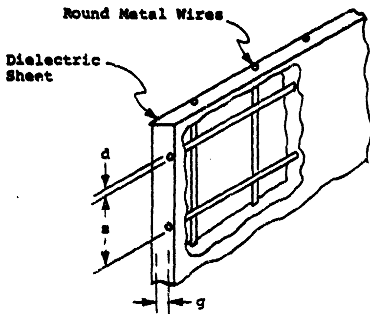
(a) wire configuration
