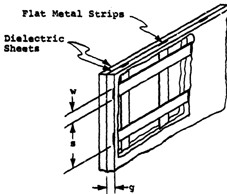
(b) strip configuration
