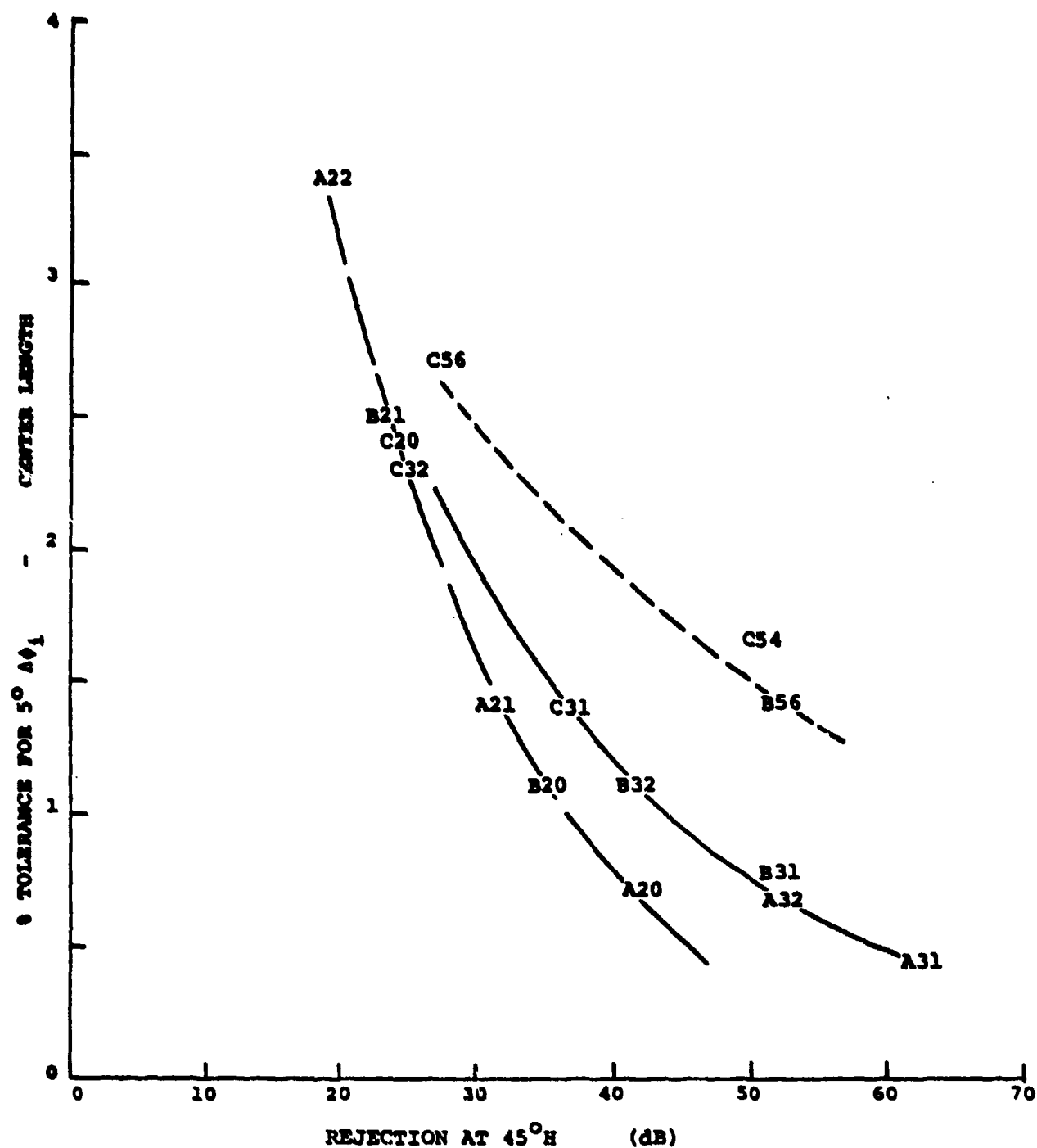
Figure 4-5 Tolerance on Center Length vs. Rejection, for 5° Δφ i Allowable
