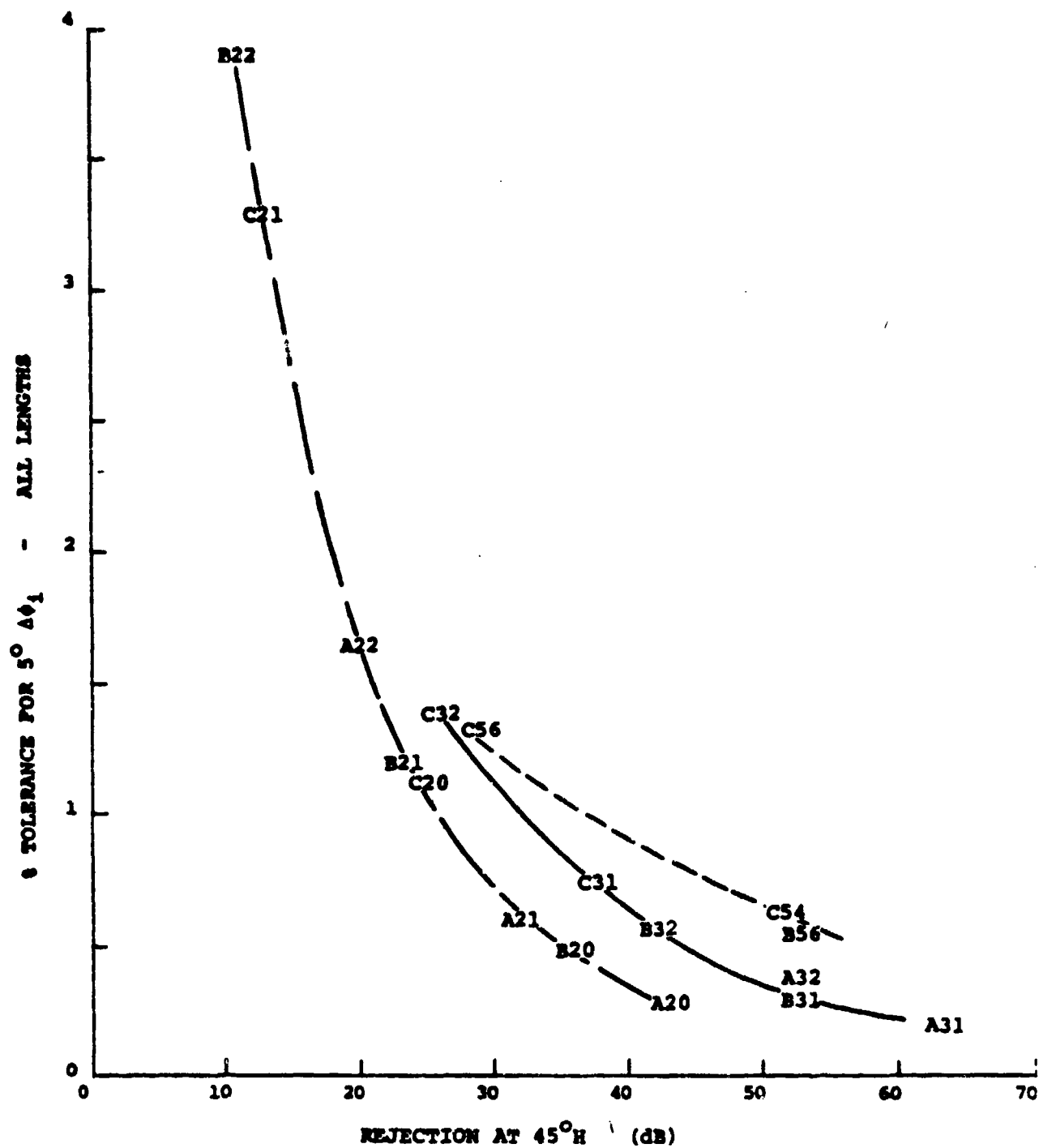
Figure 4-9 Tolerance on All Lengths Cumulative vs. Rejection for 5° Δφ i Allowable
