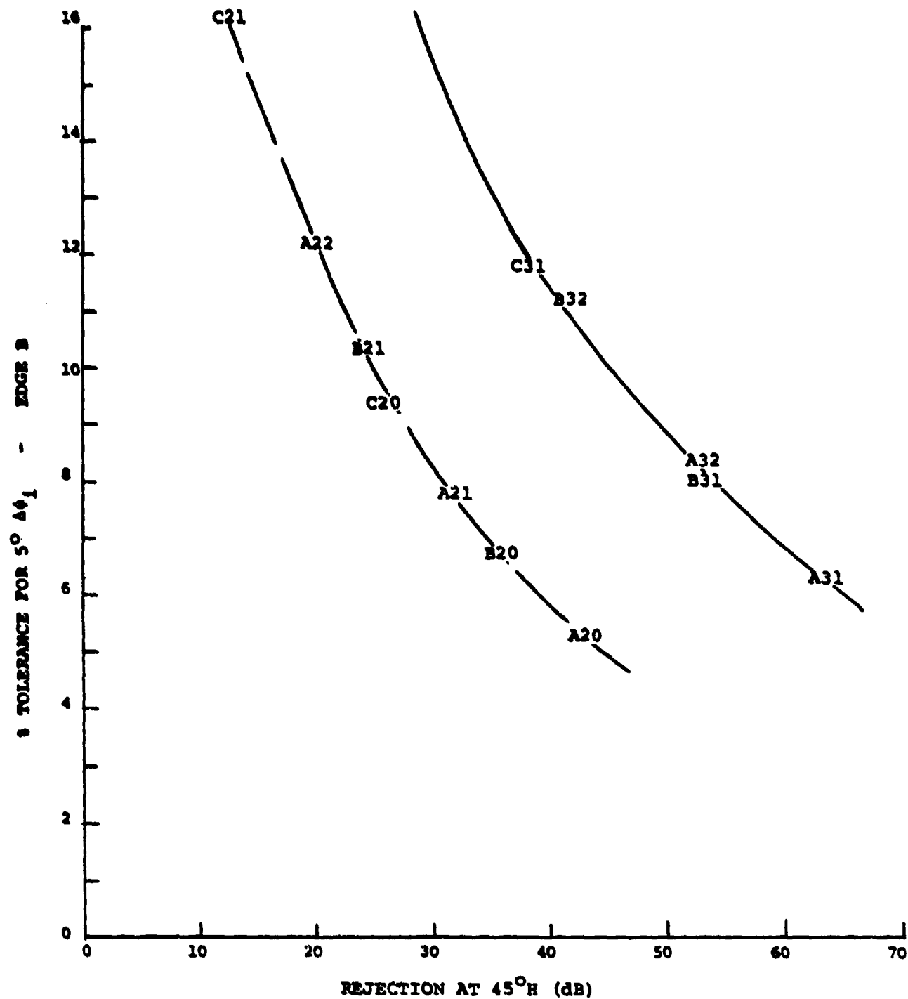
Figure 4-7 Tolerance on Edge Susceptance vs. Rejection, for 5° Δφ i Allowable
