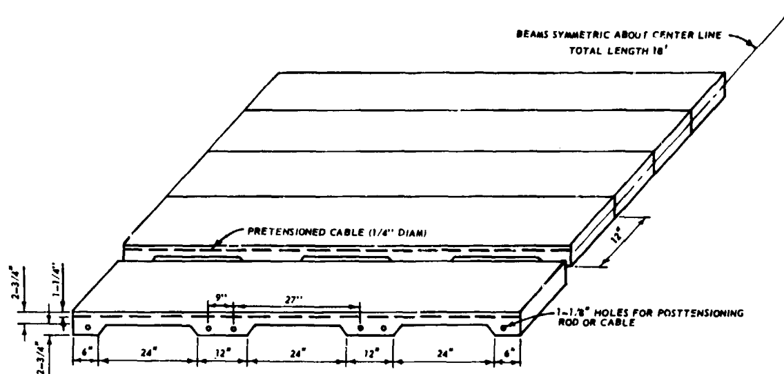
Figure 1. Precast, prestressed concrete missile mat
