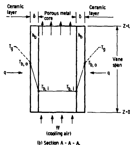
Figure 5. - Vane mathematical model.
