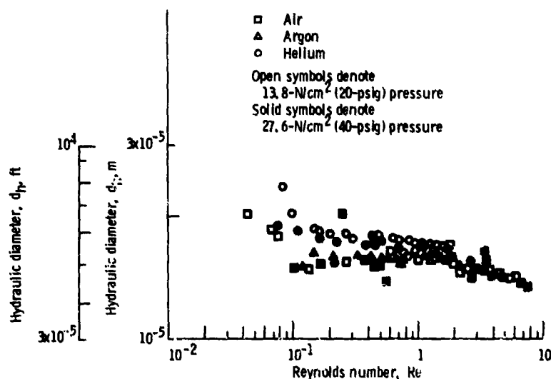
Figure 8. - Calculated hydraulic diameter as function of Reynolds number for gas flow through porous metal (75 percent porosity).
