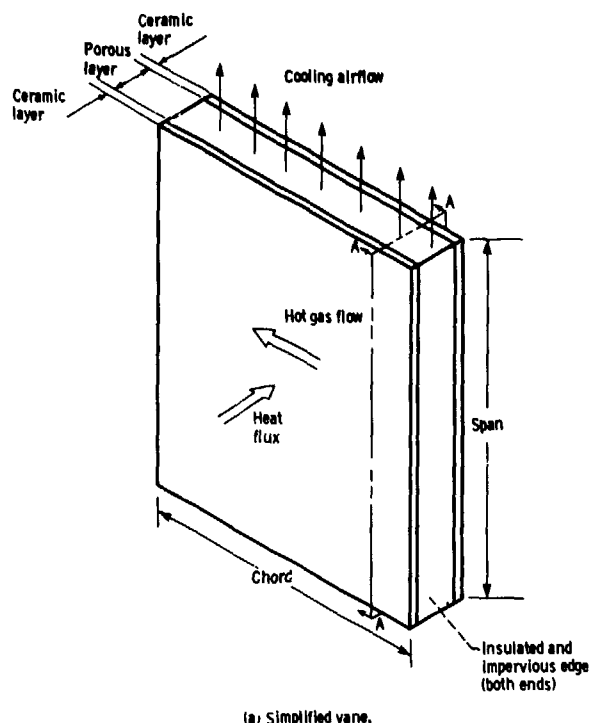
(a) Simplified vane.
