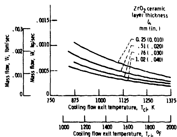
Figure 13. - Cooling mass flow in trailing edge (trailing-edge ejection) as function of cooling flow exit temperature for various ceramic thicknesses.
