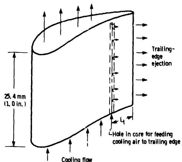
Figure 4. - Sketch of test vane core showing location of trailing-edge cooling hole.
