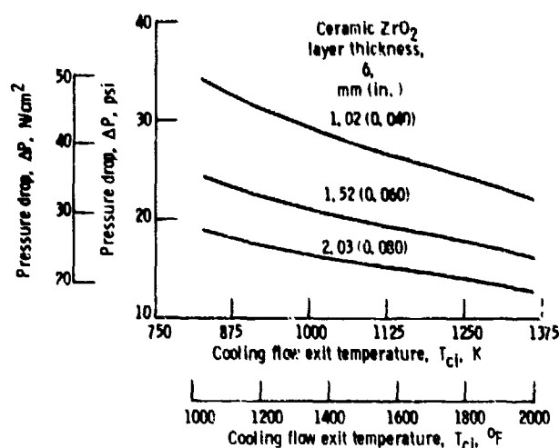
Figure 11. - Pressure drop as function of porous metal exit core (cooling flow exit) temperature.
