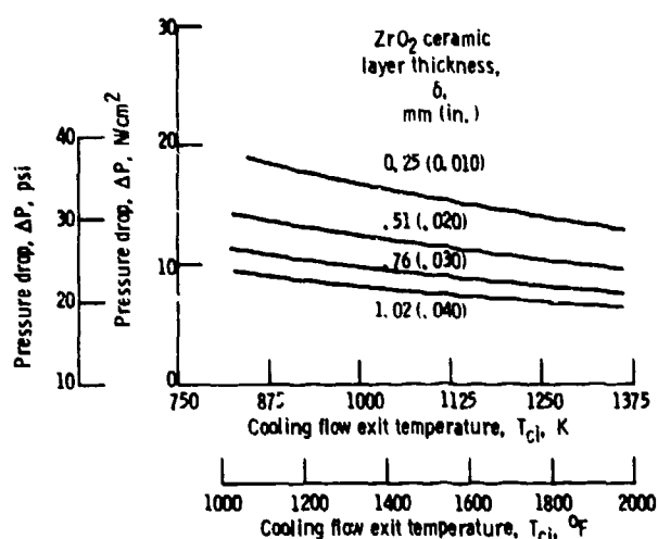
Figure 14. - Pressure drop in trailing edge (trailing-edge ejection) as function of cooling flow exit temperature for various ceramic layer thicknesses.
