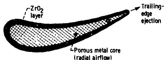
Figure 1. - Ceramic-coated porous metal vane concept.
