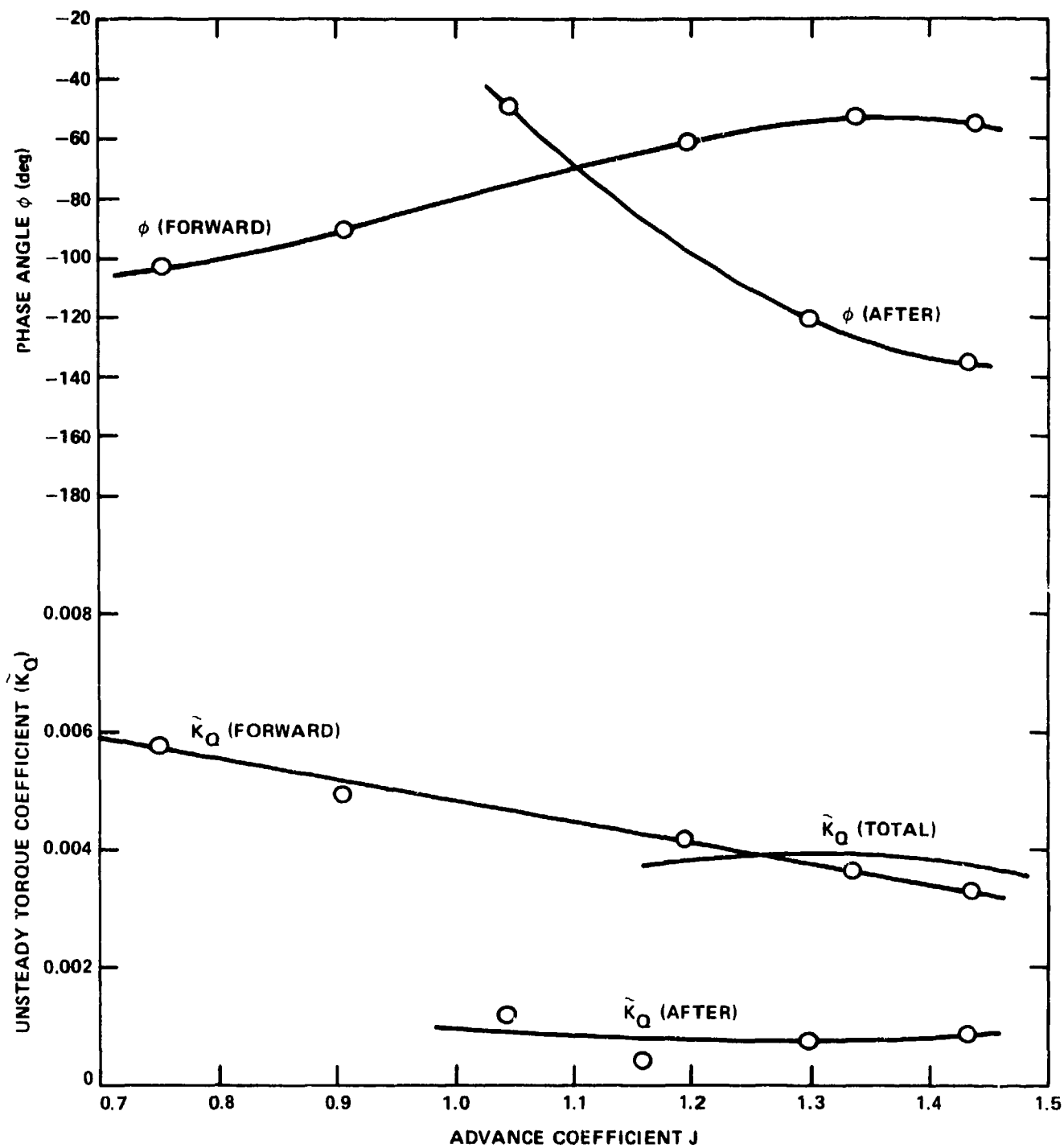
Figure 21 - Unsteady Torque on 4 \times 4 Set at 16 Times Shaft Frequency in 4-Cycle Wake
