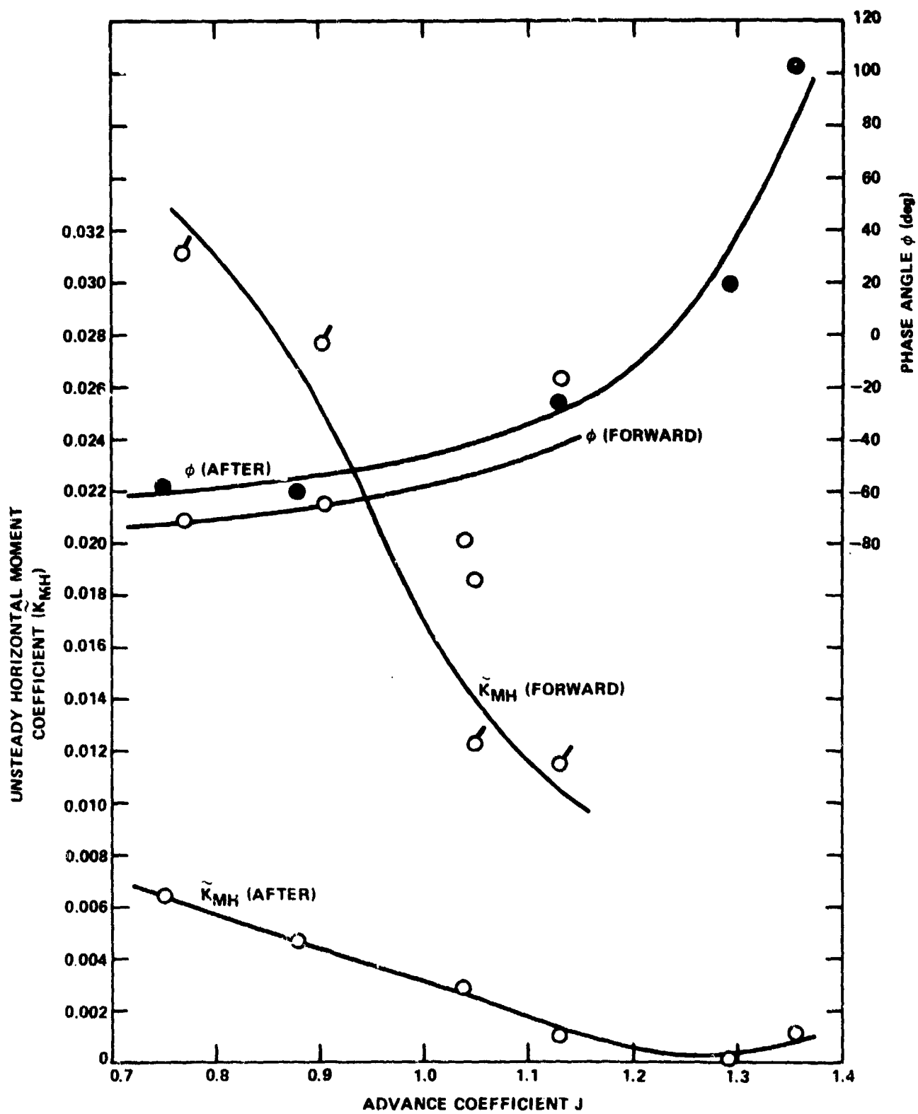
Figure 29 - Unsteady Horizontal Bending Moments on 4 × 5 Set at 9 Times Shaft Frequency in 4-Cycle Wake
