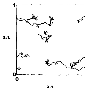
FIG. 8. The trajectories of five molecules in the xz plane during the \rho=1.01304 and \dot{\epsilon}_{xx}=0.7168 segment. The molecules originated from within a xz slice of thickness \sim L/10 taken through the center of the cell.
