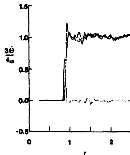
FIG. 12. The normalized angular rotation function 3\theta(r)/\dot{\epsilon}_{xz} averaged over the time regions 0.17 to 0.33 (—), 1.54 to 2.05 (---), and 3.85 to 4.46 (.....) for the segmented \rho = 1.01304 and \dot{\epsilon}_{xz} = 0.7168 calculation.
