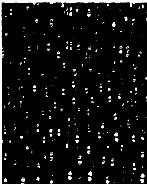
Figure 5.-- P. glycyphloea , pore and parenchyma arrangement (IPTw 12968, Bahia) X 30.
