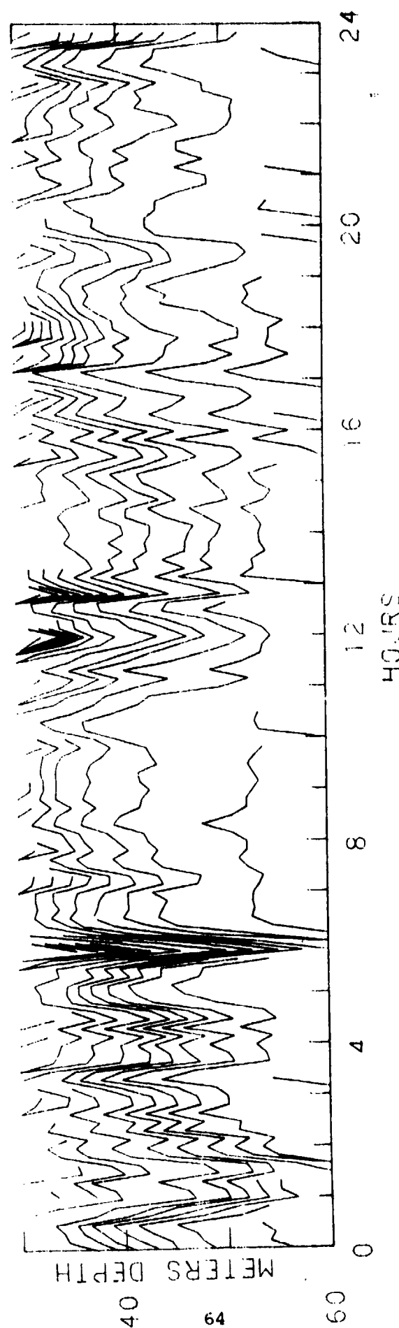
Figure 16. Isotherm depths for .2° increments ranging from 10.2° to 12.4°.
