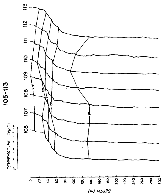
XBT Section 10.
