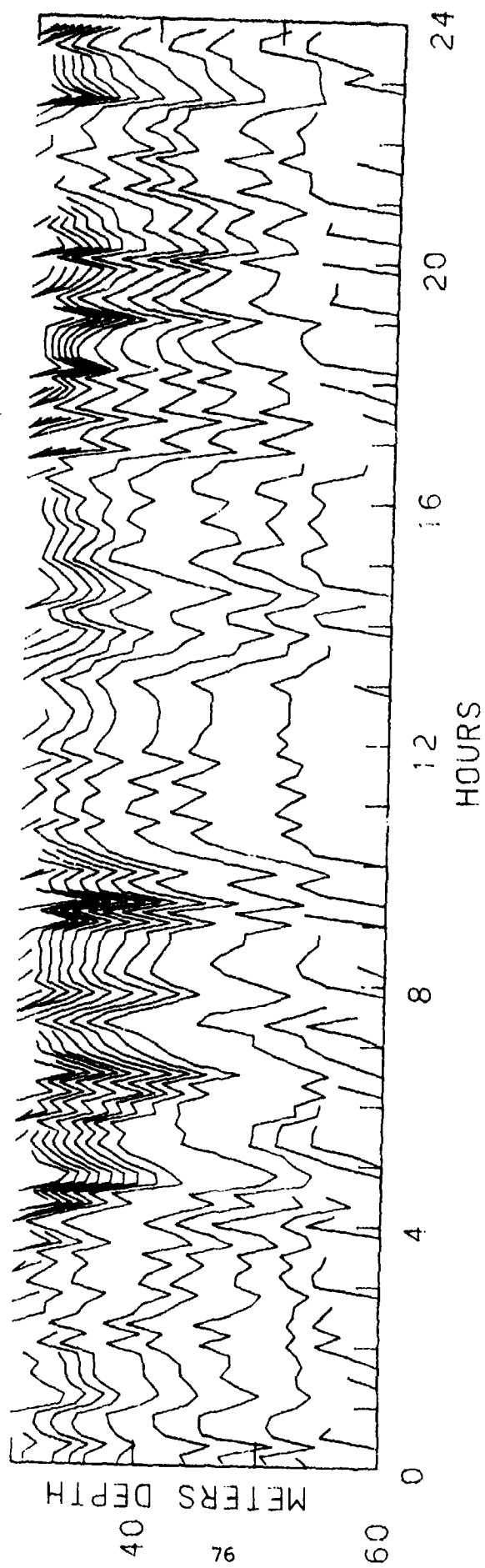
Figure 16. Isotherm depths for .2° increments ranging from 10.2° to 13.0°.
