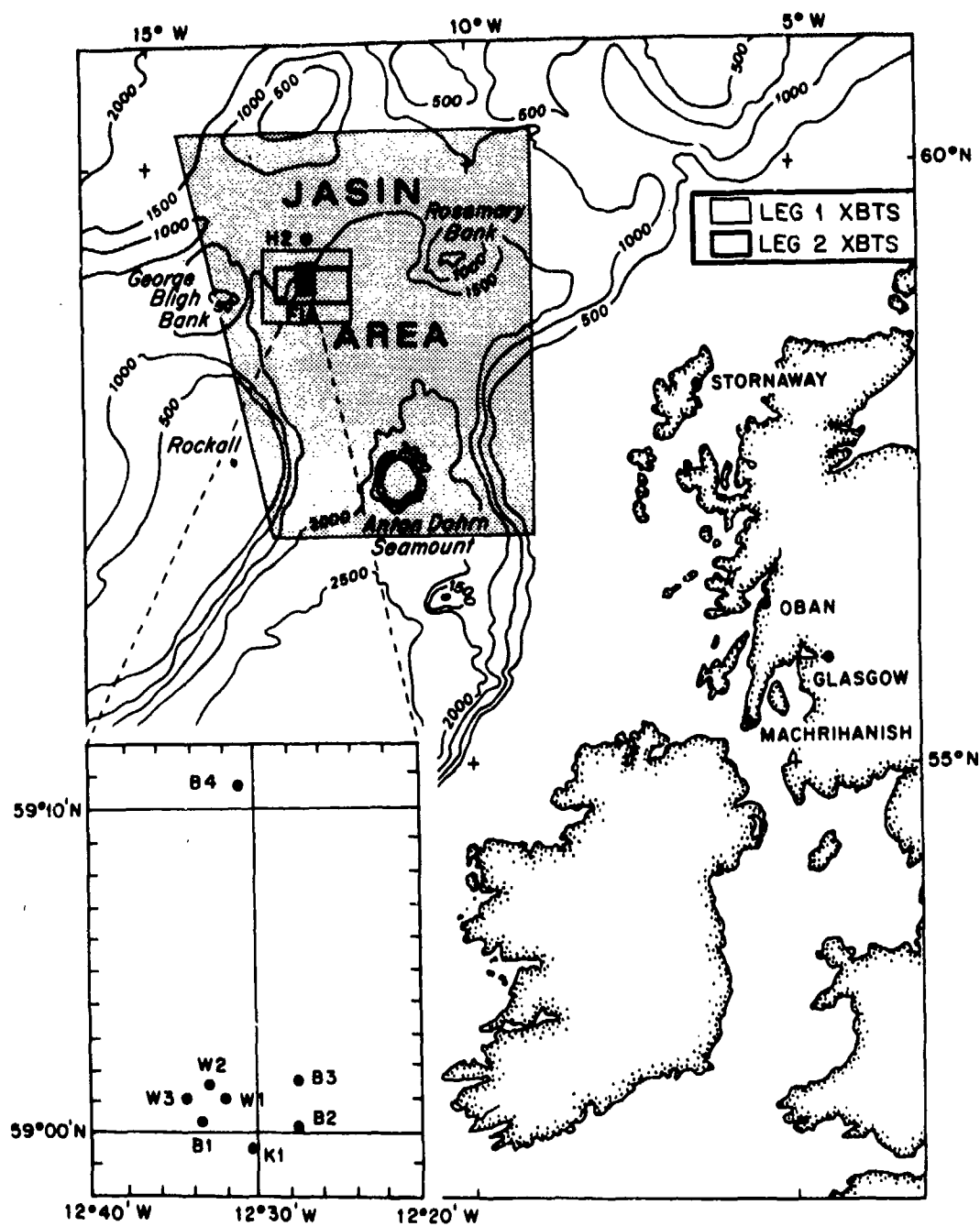
Figure 17. XBT positions.
