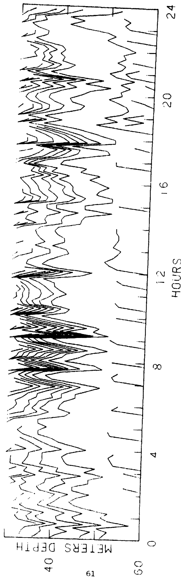
Figure 16. Isotherm depths for .2^{\circ} increments ranging from 10.0^{\circ} to 12.2^{\circ} .
