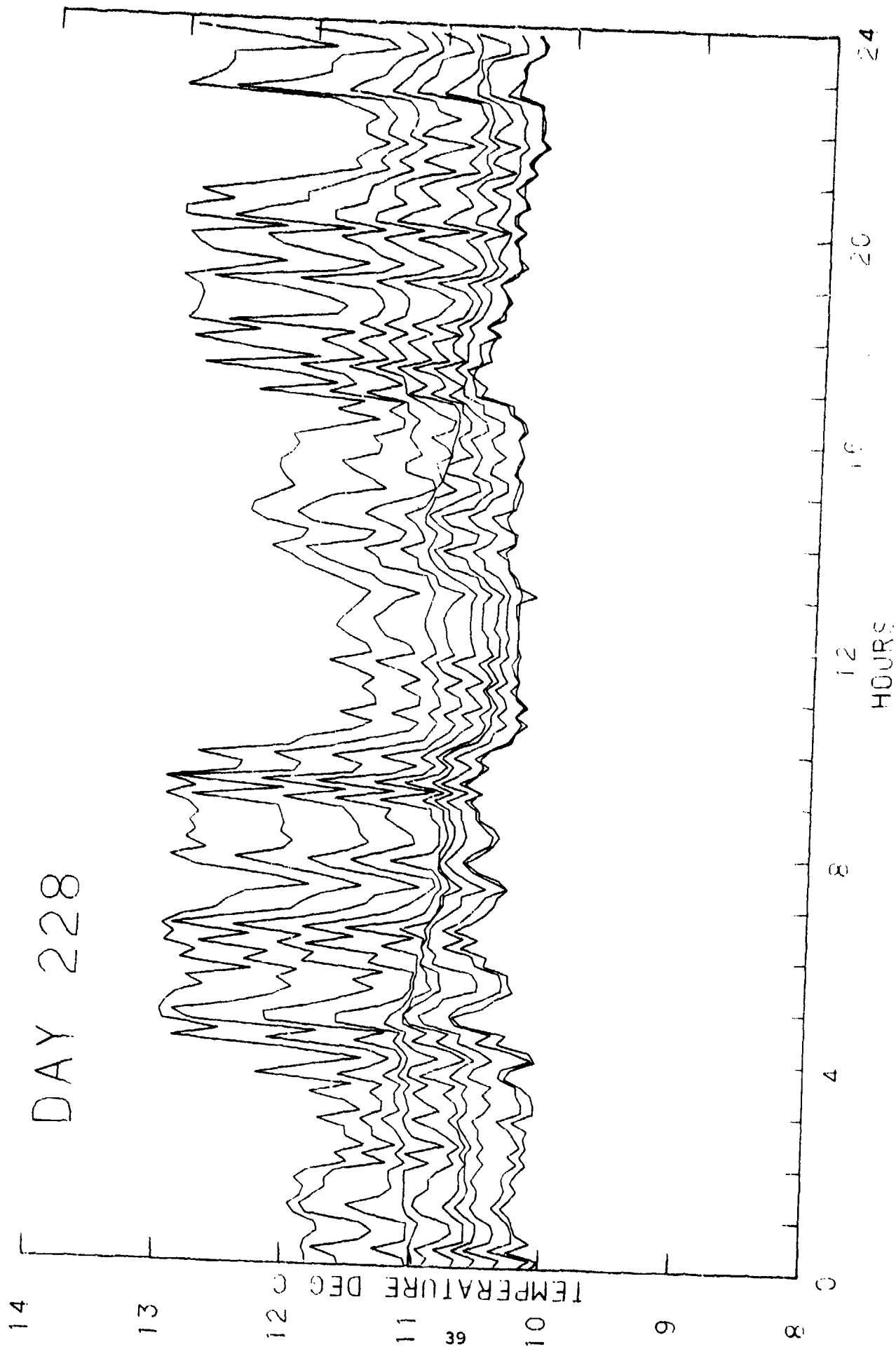
Figure 15. Temperature at 31, 34, 37, 40, 43, 46, 49, 52, 55 and 58 m (nominal depths).
