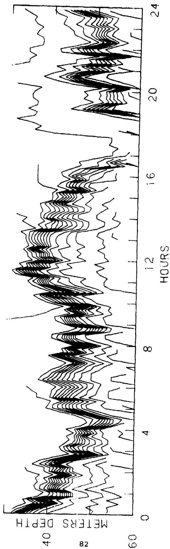
Figure 16. Isotherm depths for .2° increments ranging from 9.8° to 12.4°.
