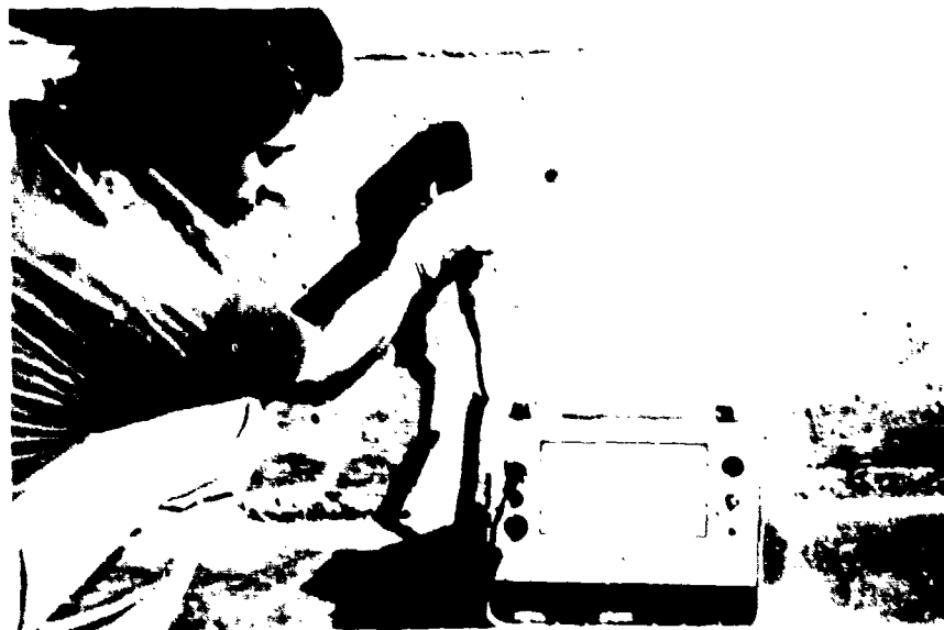
Fig. 21 Use of a "Cover Meter"
