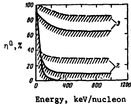
Fig. 16--Conversion coefficients for hydrogen ions into neutrals in gas targets (solid lines) and plasma targets (broken lines) for 1-- H^+ ; 2-- H_2^+ and H_3^+ ; and 3-- H^- [65]
