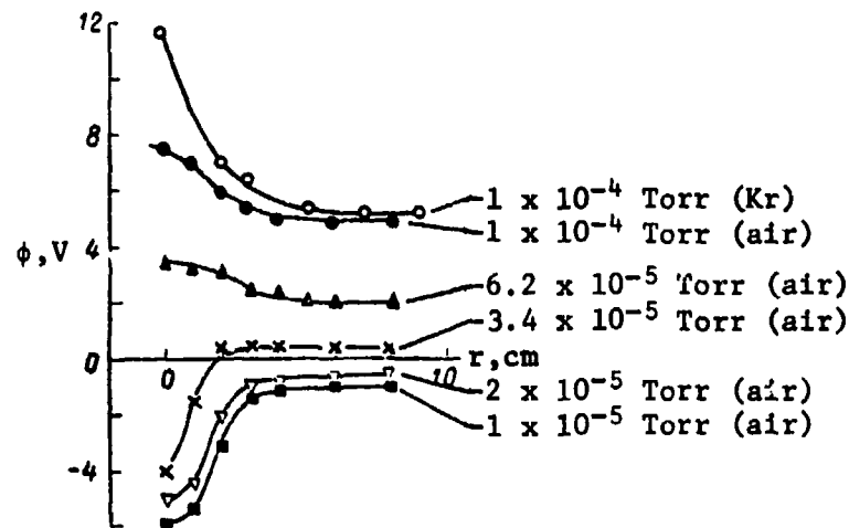
Fig. 26--Radial potential distribution as function of pressure [76] (By permission of American Institute of Physics)
