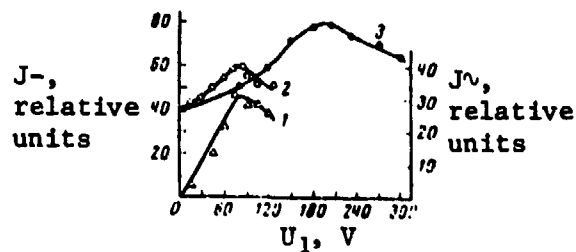
Fig. 29--Current density of alternating beam J_\nu (curve 1) and constant beam J_- (curve 2) as functions of voltage amplitude U_1 of modulating generator; dependence of J_- on constant voltage applied to modulator (curve 3) [82] (By permission of American Institute of Physics)
