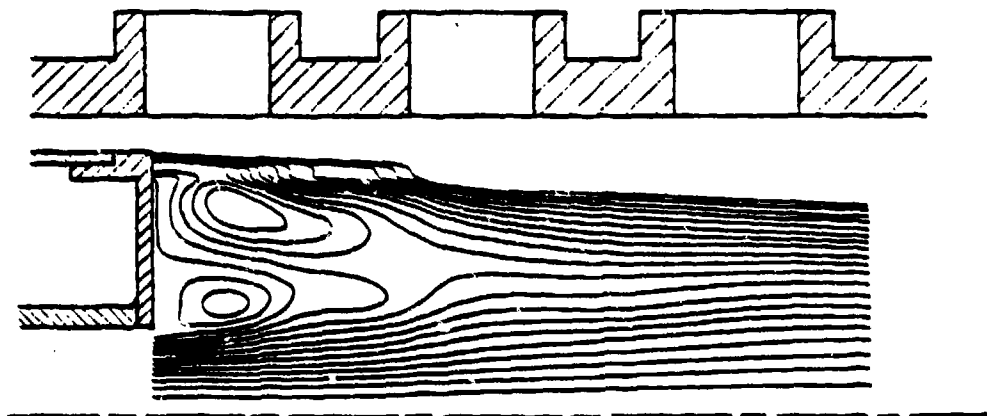
Figure 1c. Streamline contours
