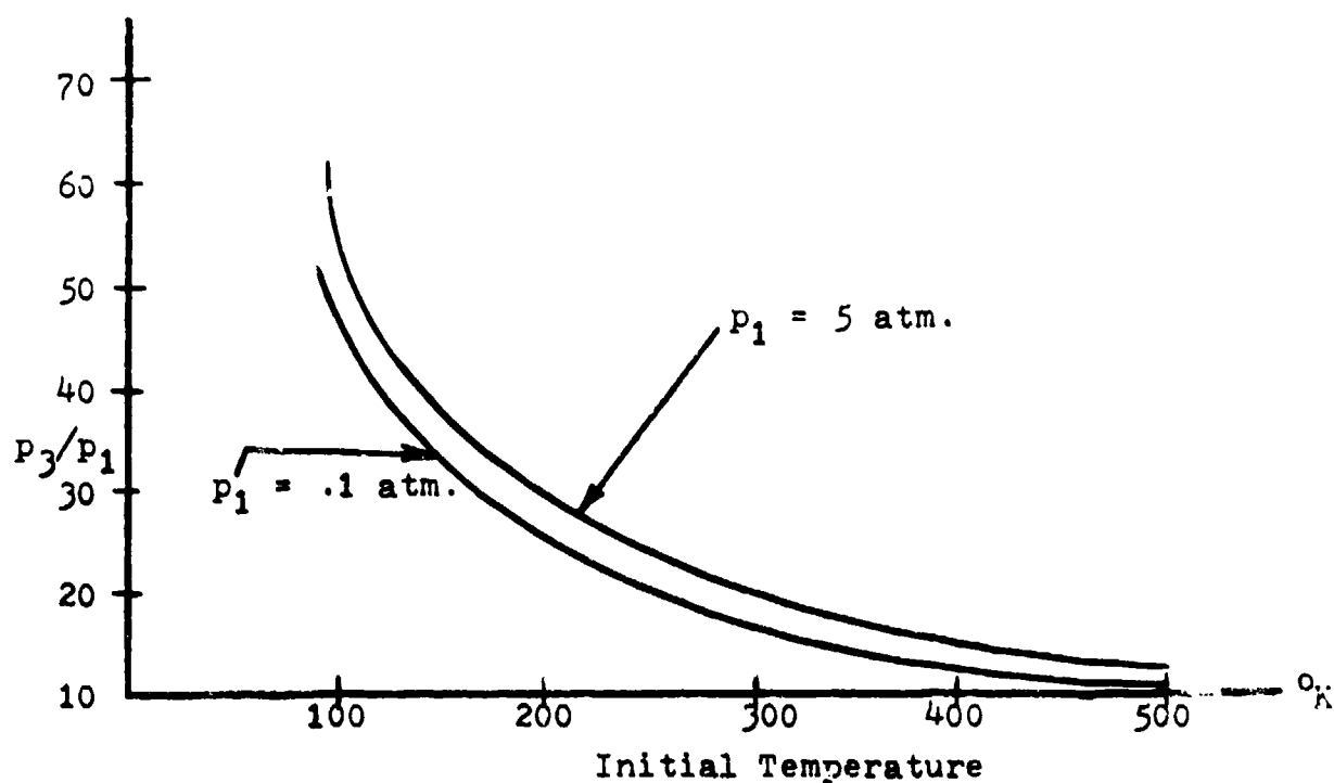
Figure 2 P_3/P_1 vs. T_1 For \frac{1}{2}\text{O}_2 + \text{H}_2 + \text{He}
