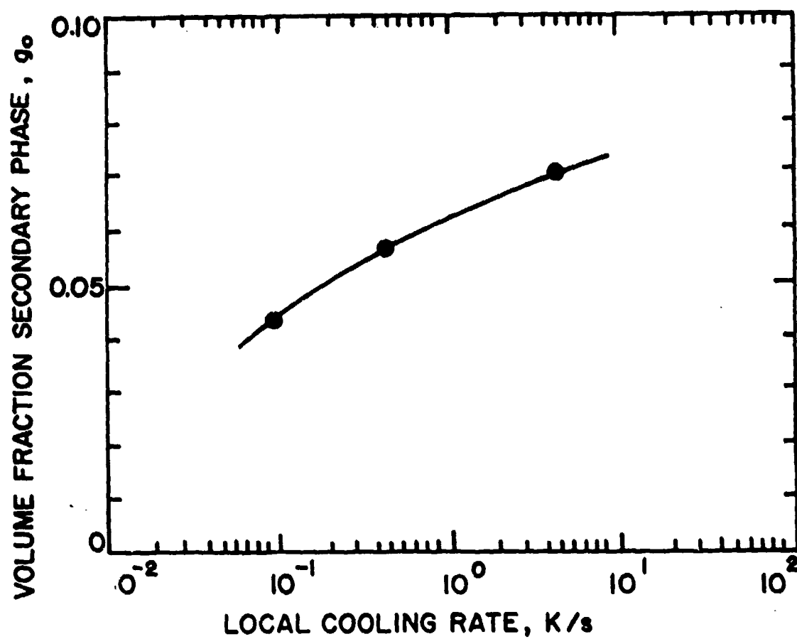
Fig. 23: Volume fraction of interdendritic \gamma' phase, g_0 , versus local cooling rate. Ni-19.2at%Al-11.9at%Cr.
