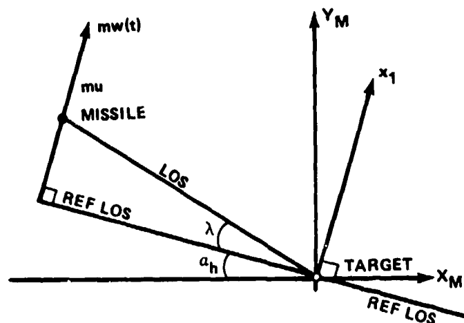
Figure 1. Relative intercept geometry.
