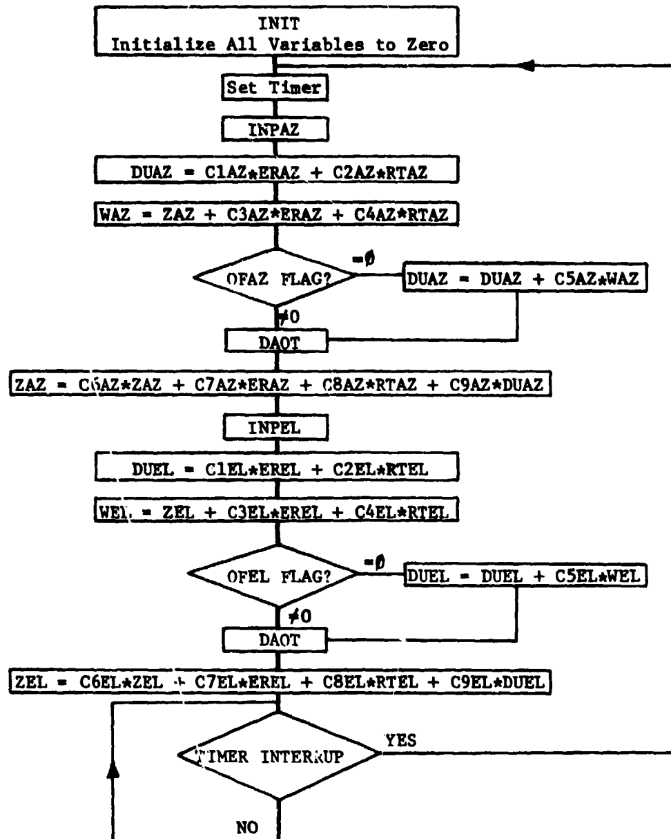
Fig. 8 XM-97 OPTIMAL CONTROLLER FLOW CHART (INCLUDING DISTURBANCE CANCELLATING CONTROL)
