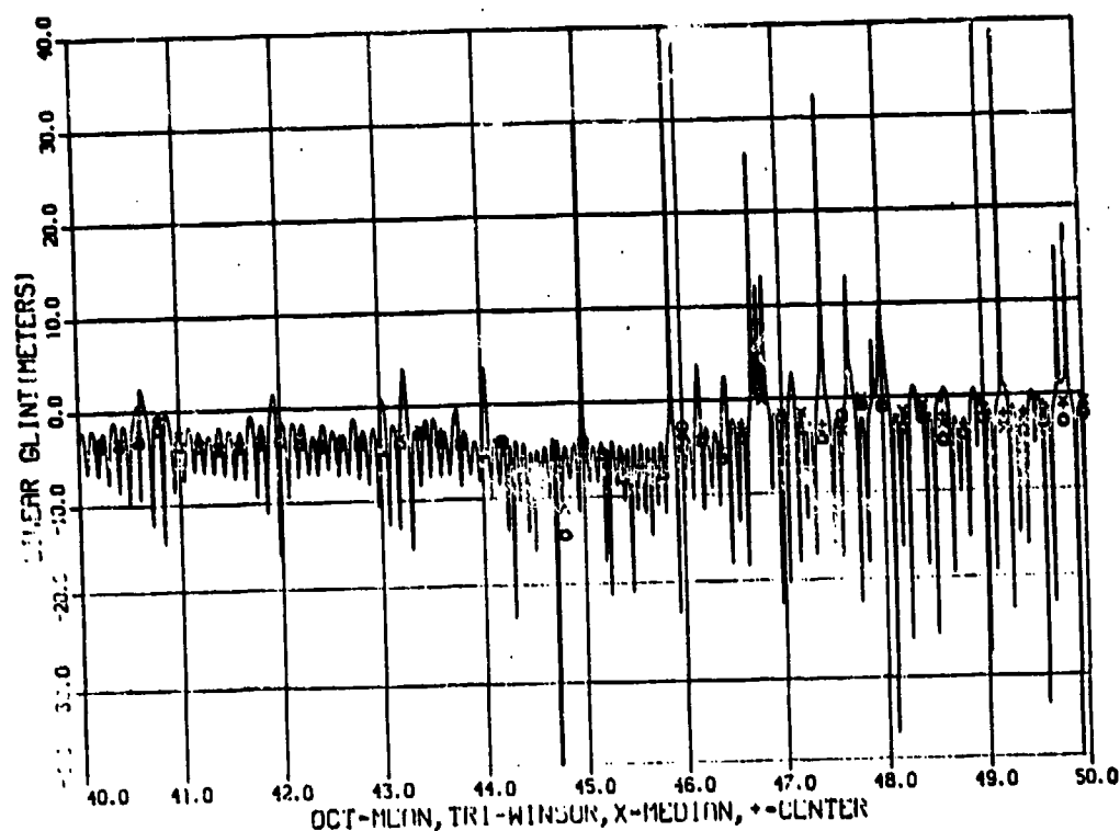
FIGURE 6. Location Comparison (N-Shape Glint).
