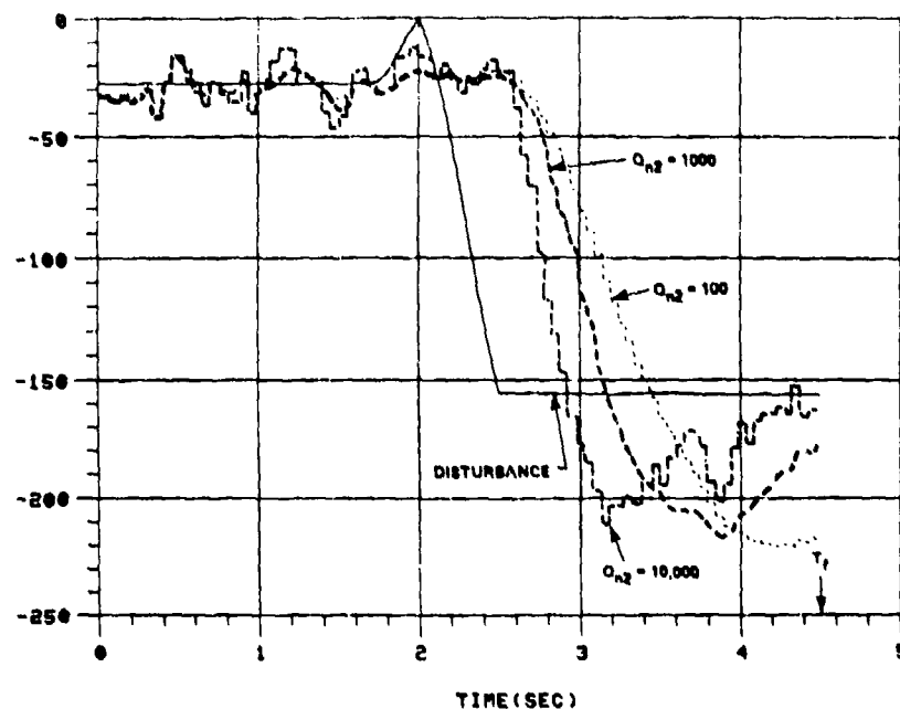
Figure 8. Effect of choice of \tilde{Q}_{n2} on lag in disturbance estimate ( \tilde{S}=100 ).
