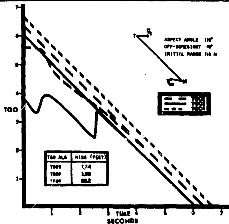
FIGURE 4 TGO2, TGO3, TGO4 VERSUS TRUE TIME-TO-GO
