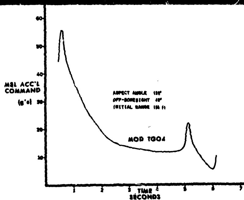
FIGURE 4 MB1 ACC'L COMMAND VERSUS TIME FOR MODIFIED T004
