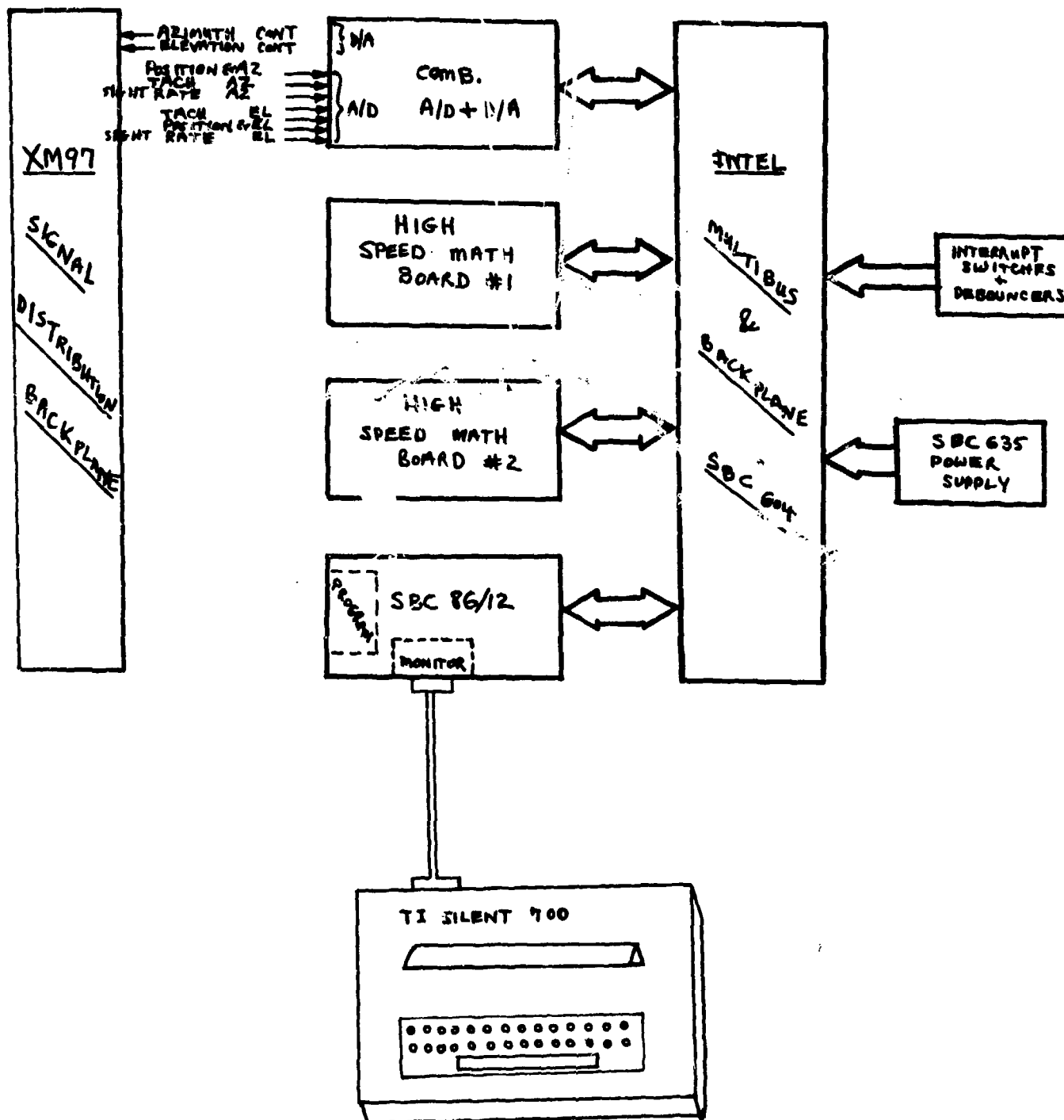
Fig. 7 XM-97 DIGITAL CONTROLLER HARDWARE
