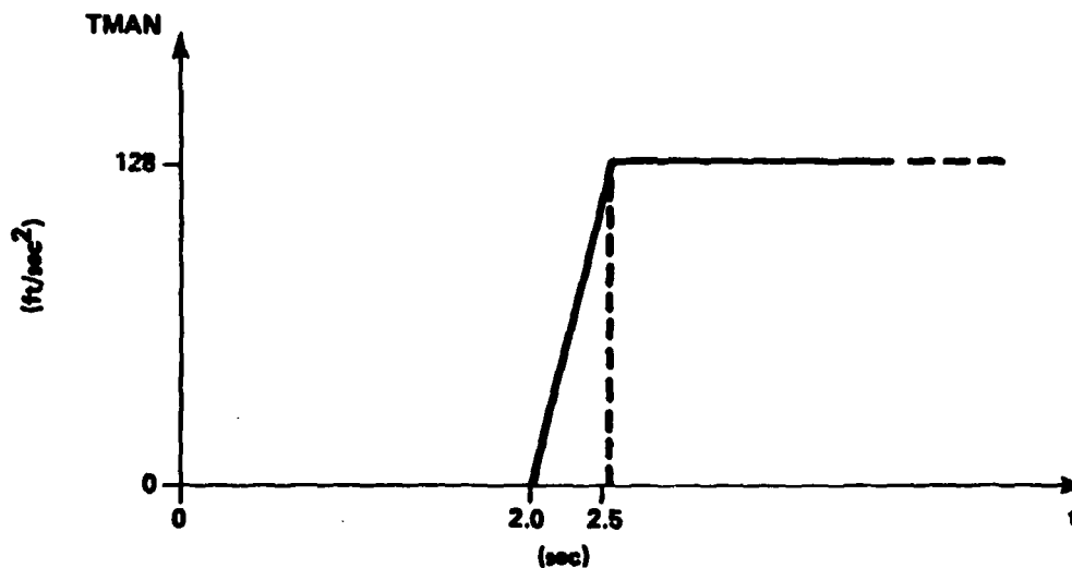
Figure 3. Actual maneuver disturbance (TMAN) input.
