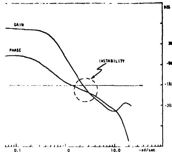
Fig. 11. DR Gunner-Vehicle Open-Loop Transfer Function, K_R=0.5
