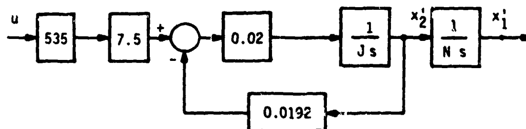
Fig. 4 SIMPLIFIED OPEN-LOOP XM-97 HELICOPTER TURRET CONTROL SYSTEMS WITH J=3 \times 10^{-4} (AZ) AND J=2.7 \times 10^{-4} (EL)
