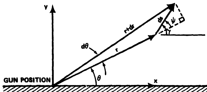
Figure 9 Geometrical Relationships for Prediction Error Analysis
