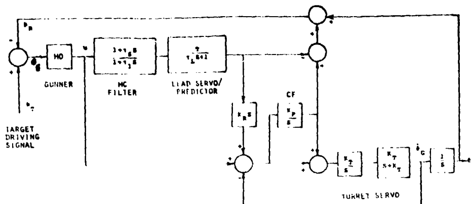
Fig. 3. Disturbed Reticle Design, State Variable Model.
