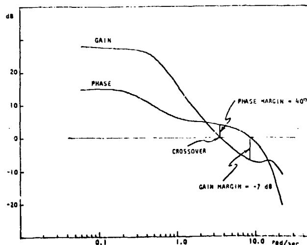
Fig. 10. DR Gunner-Vehicle Open-Loop Transfer Function, K_R=1
