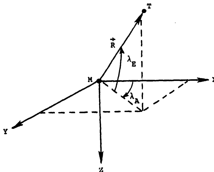
FIGURE 2: MISSILE-TARGET LINE-OF-SIGHT GEOMETRY IN INERTIAL COORDINATES
