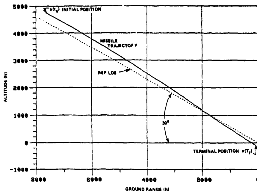
Figure 5. Missile trajectory with terminal weighting \tilde{S}=100 .
