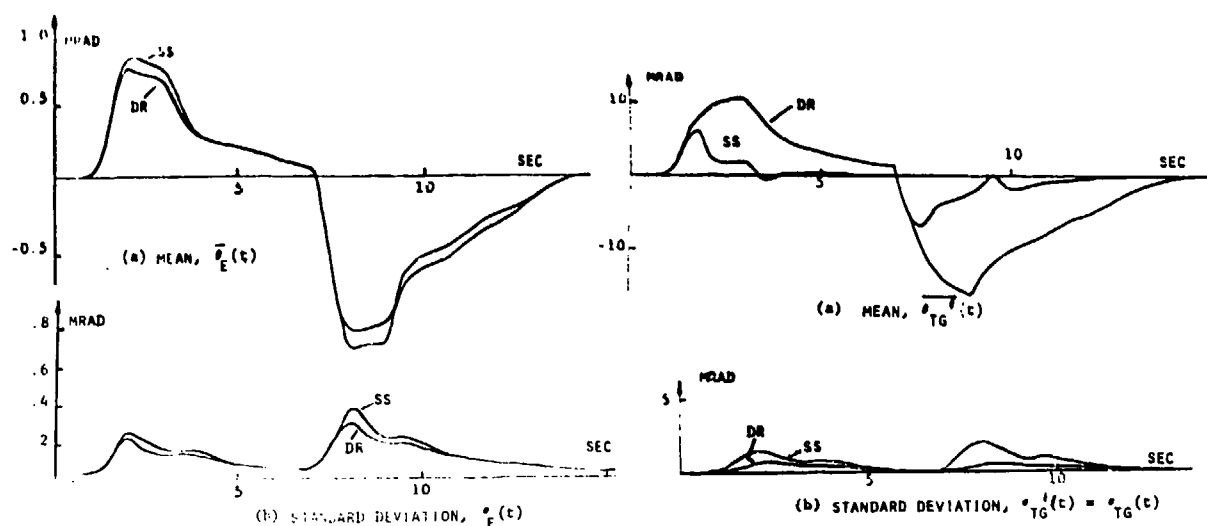
Fig. 14 Tracking Error Ensemble Statistics Fig. 15 "First-Order" Gun Pointing Error Statistics
