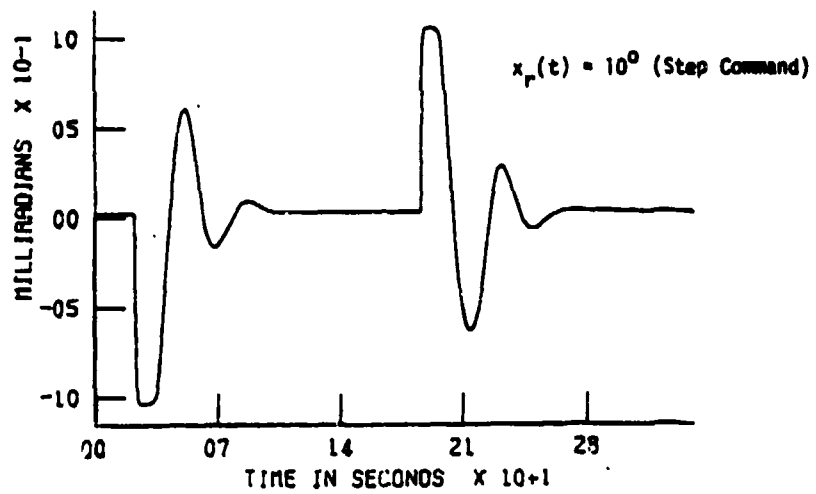
(a) Azimuth Angular Position Error
