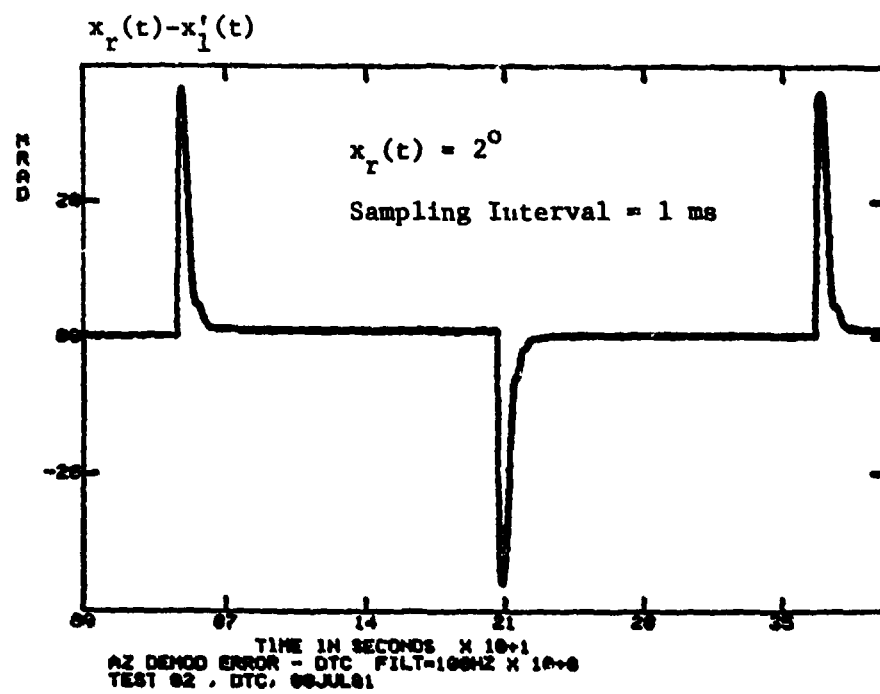
(a) STEP RESPONSE - AZIMUTH CHANNEL
