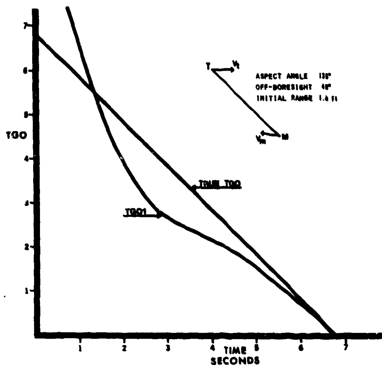
FIGURE 3 TGO1 VERSUS TRUE TIME-TO-GO
