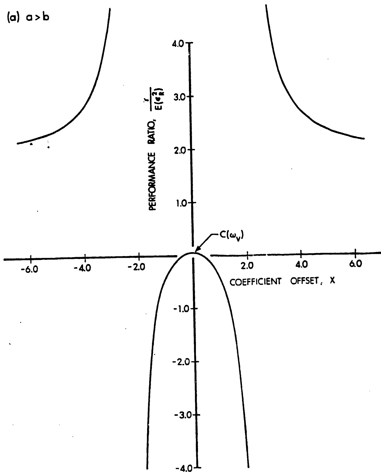
Figure 1 (a) Contours of Predictor, Performance Functions.
