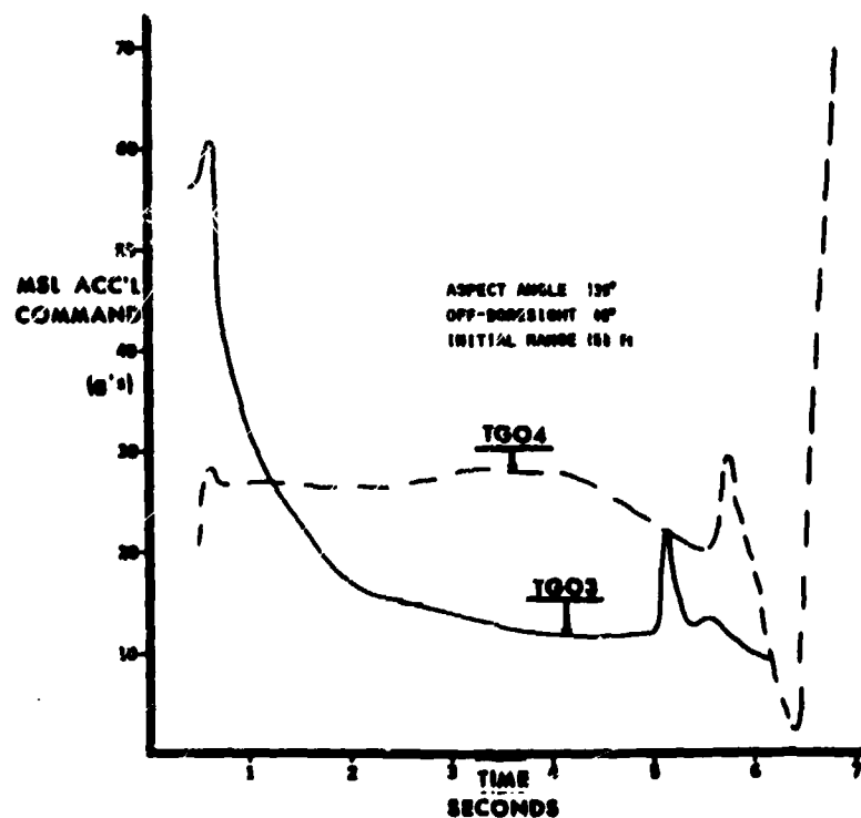
FIGURE 5 MS1 ACC'L COMMANDS VERSUS TIME FOR TGO3 AND TGO4
