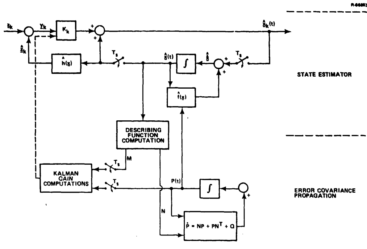
Figure 3 Statistically-Linearized Kalman Filter
