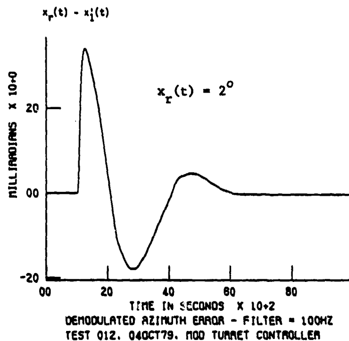
(a) STEP RESPONSE - AZIMUTH CHANNEL
