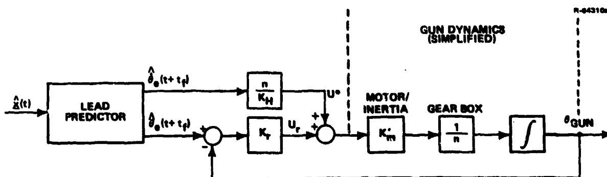
Figure 8 Predictor/Gun Pointing System Structure
