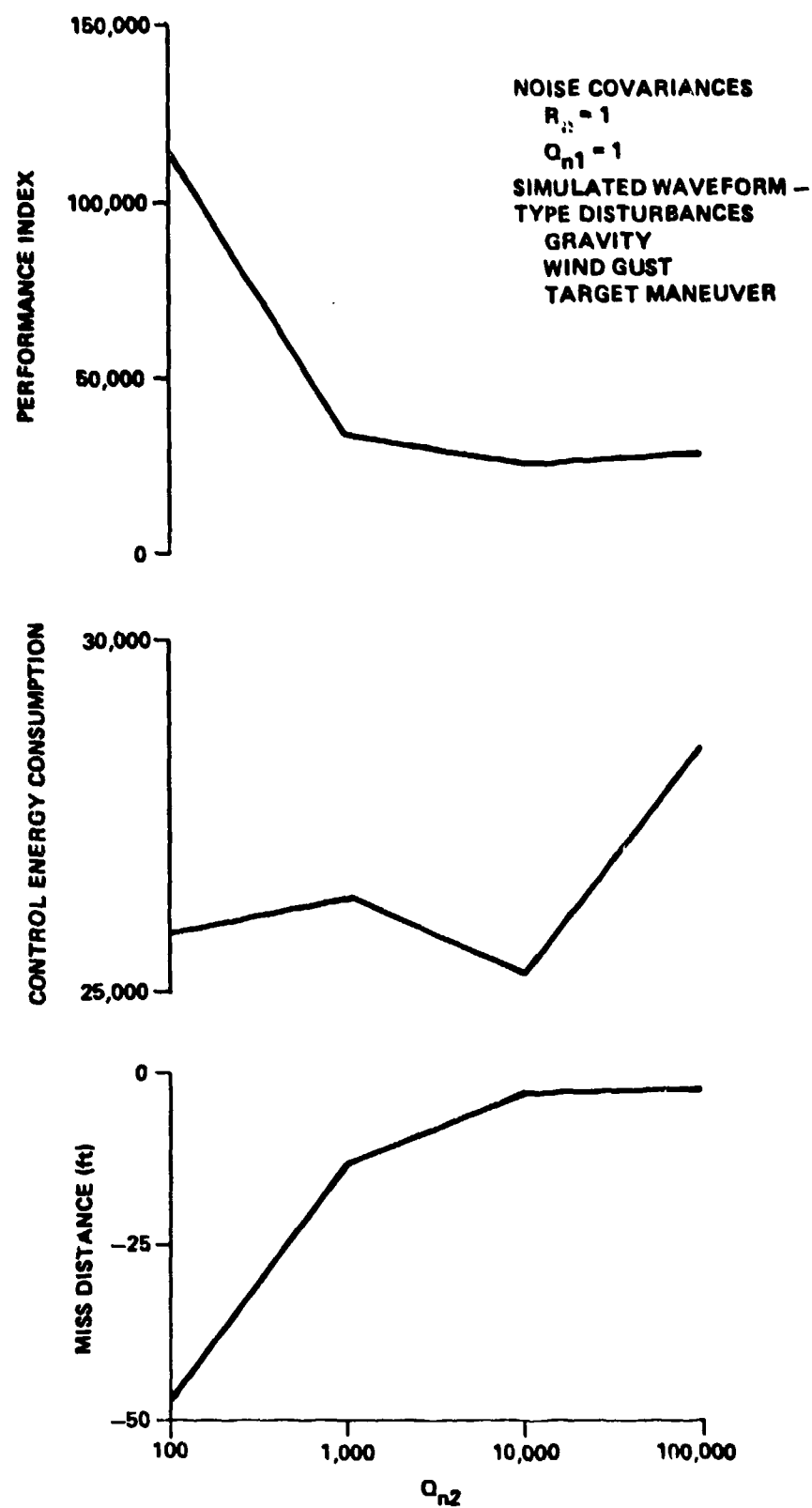
Figure 7. Noisy DUC performance versus choice of Q_{n2} ( \tilde{S} \approx 100 ).
