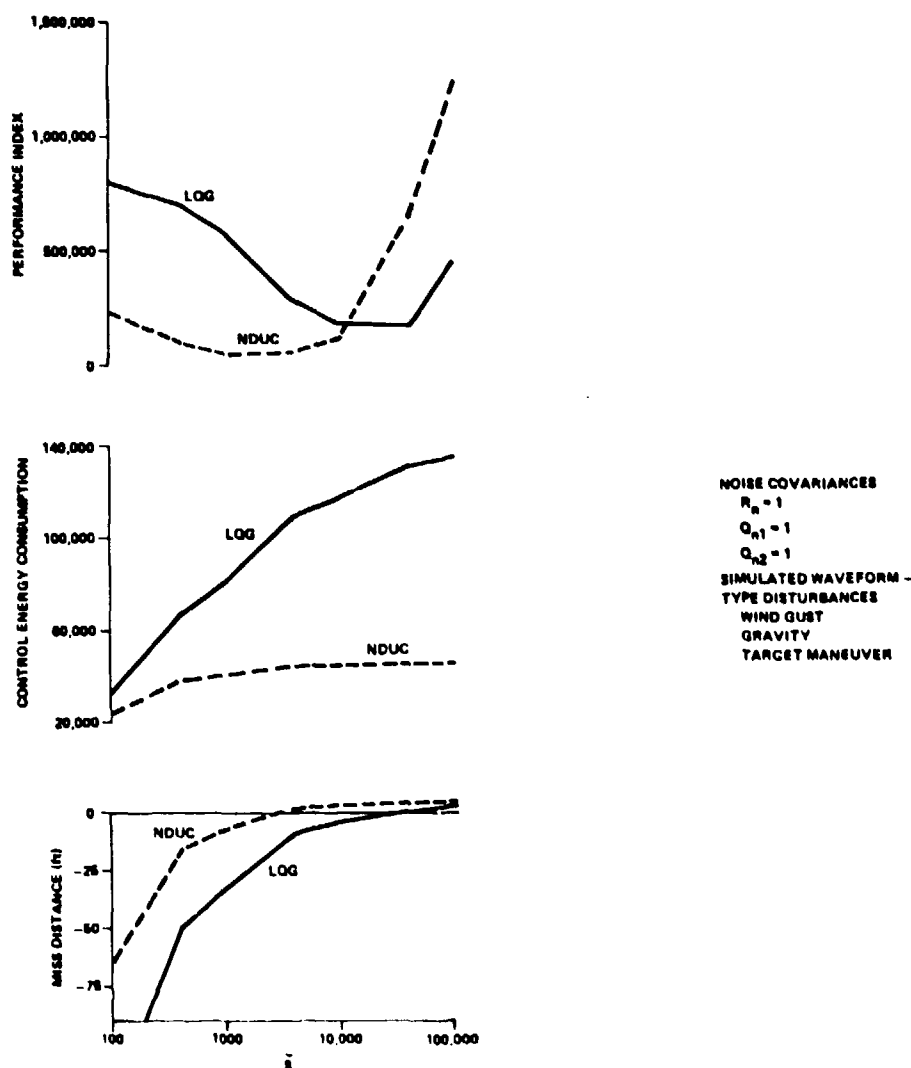
Figure 4. Performance as a function of terminal weighting \tilde{S} .
