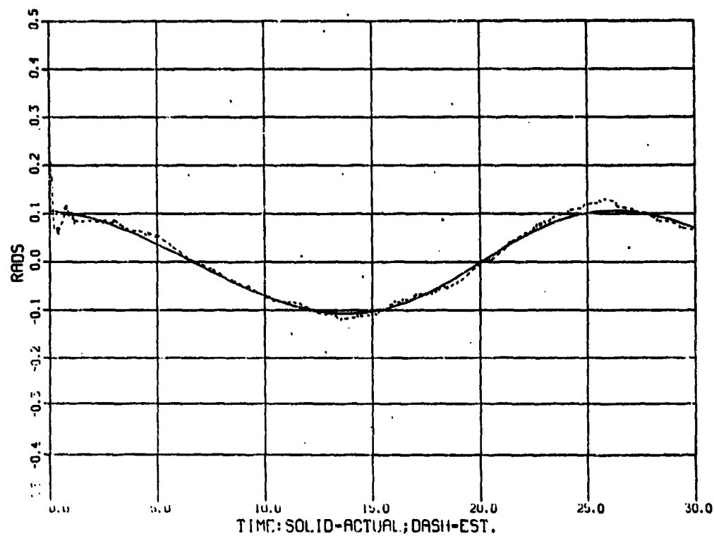
FIGURE 2. Estimated Target Position vs Actual.
