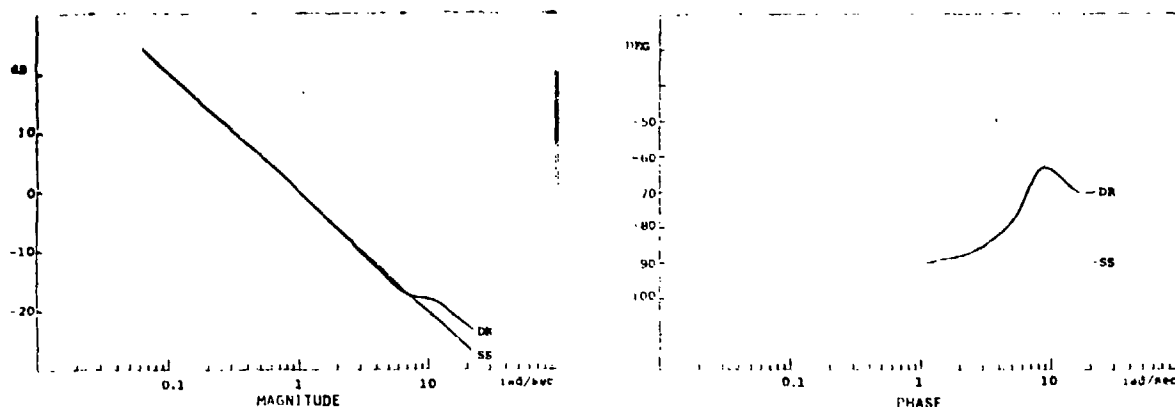
Fig. 4. Controlled Element Dynamics \theta_R(s)/u(s) .
