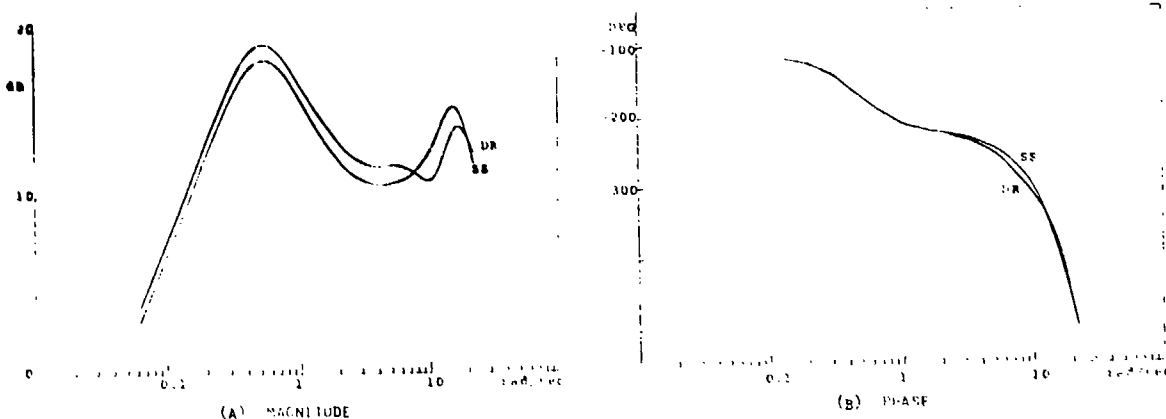
Fig. 9. Gunner Transfer Function, H(s) .
