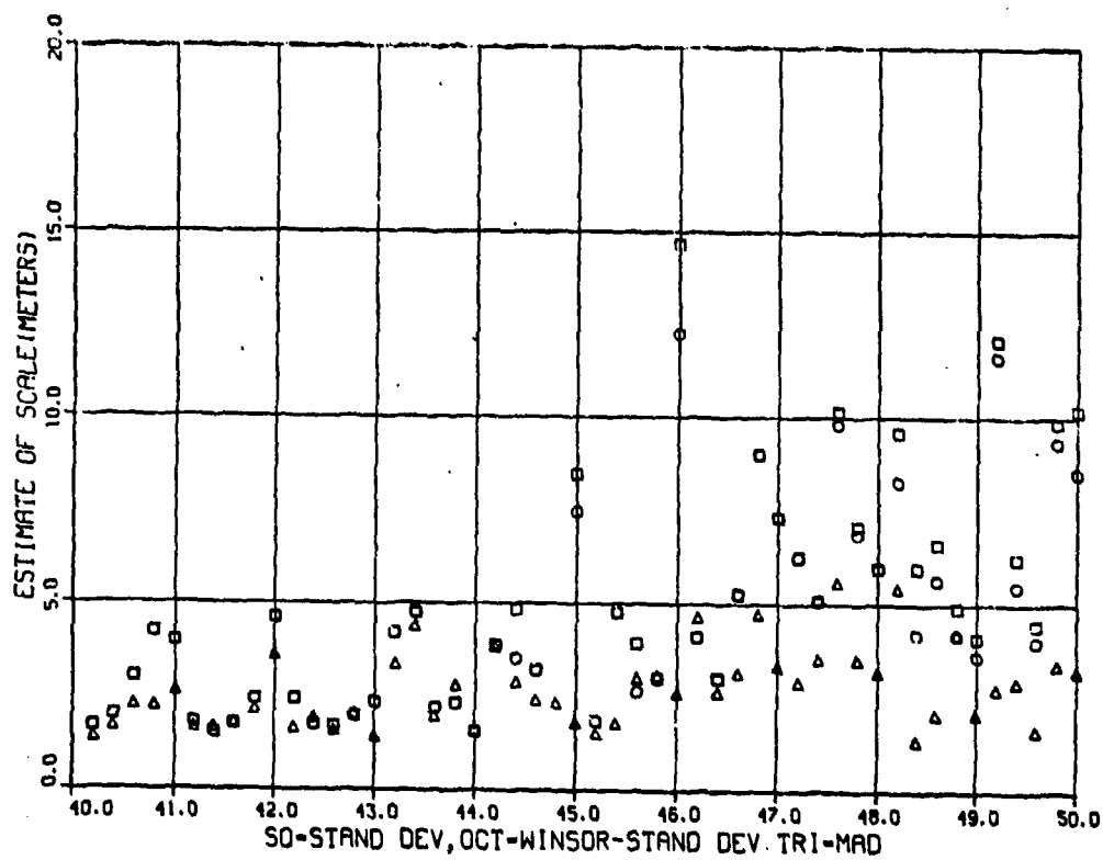
FIGURE 8. Scale Comparison (N-Shape Glint).
