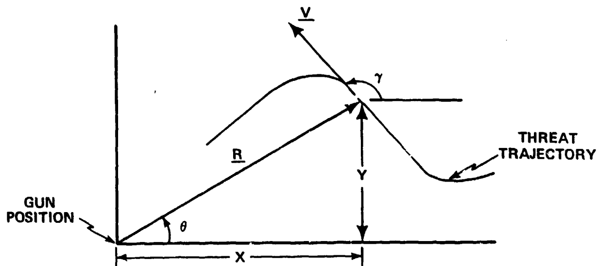
Figure 2 Engagement Geometry
