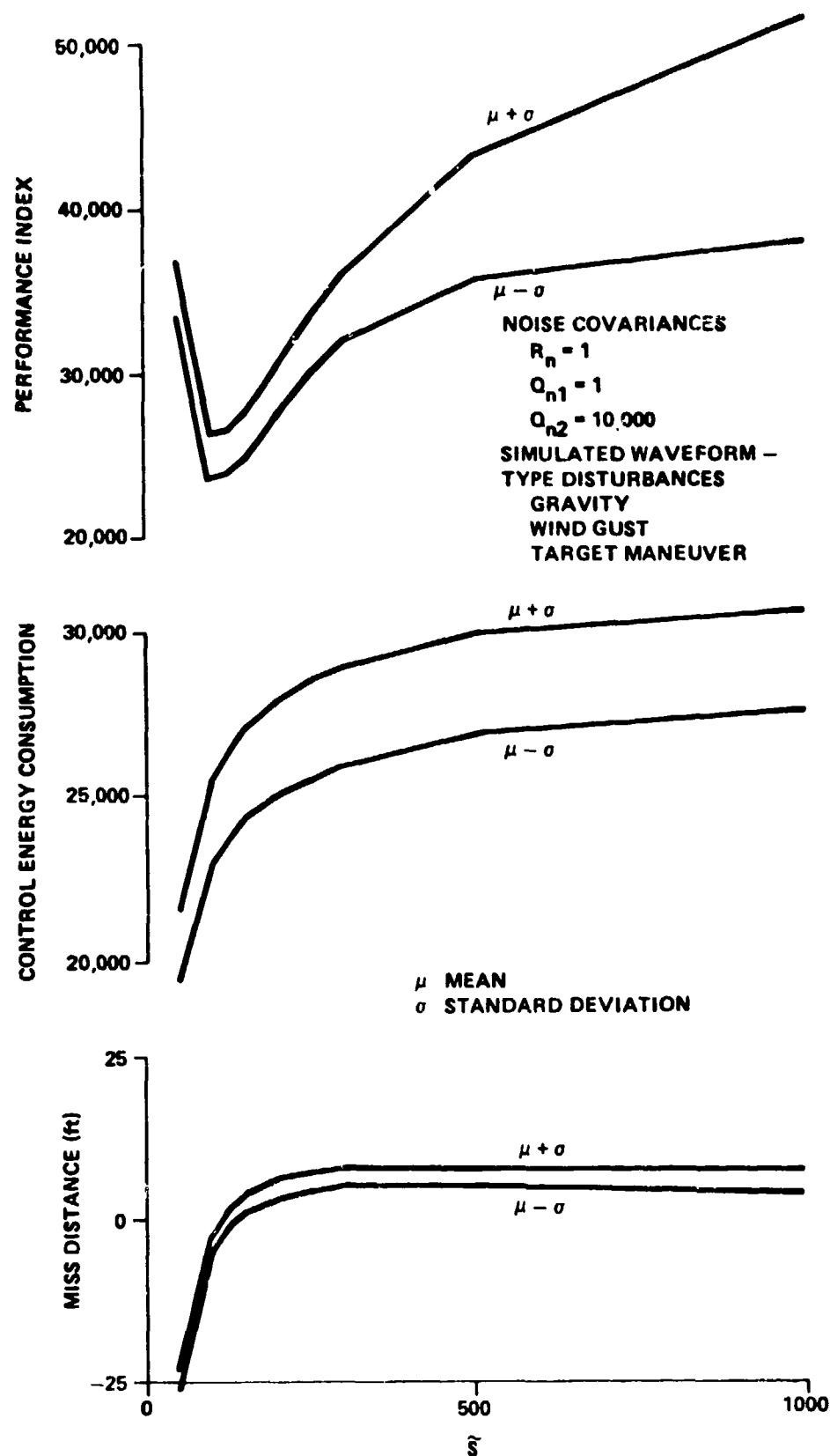
Figure 10. Monte Carlo bounds on noisy DUC performance versus terminal weighting.
