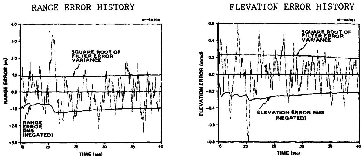
Figure 6 . Anti-Radar Missile Tracking Performance
