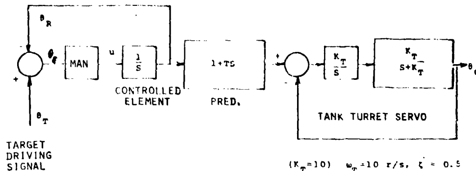
Fig. 7. Stabilized Sight-Director System.
