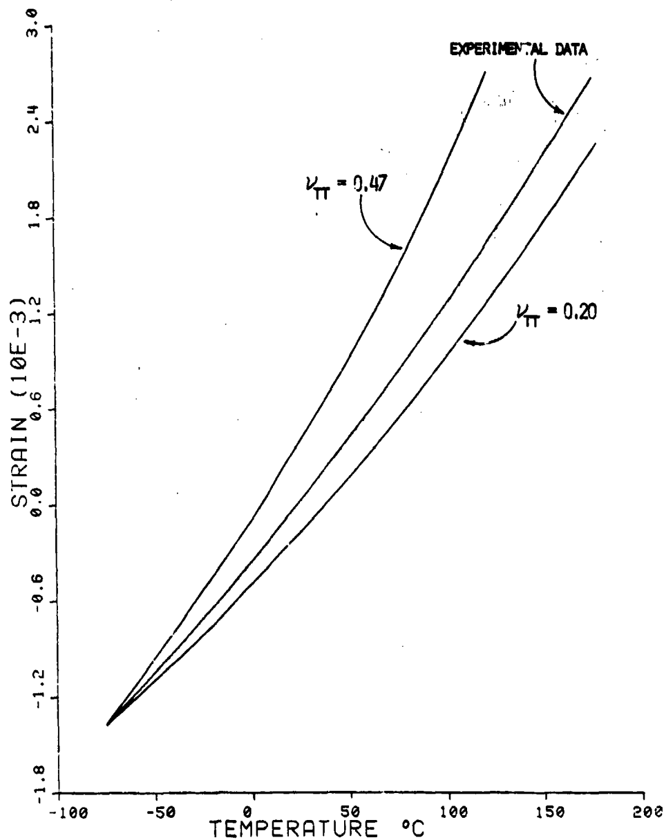
Figure 71. Unconditioned Transverse Thermal Expansion Sensitivity to Poisson's Ratio of the Matrix for S2 Glass/3501-6 Glass/Epoxy (Base Value of Matrix \nu_{\text{TT}} = 0.34 )
