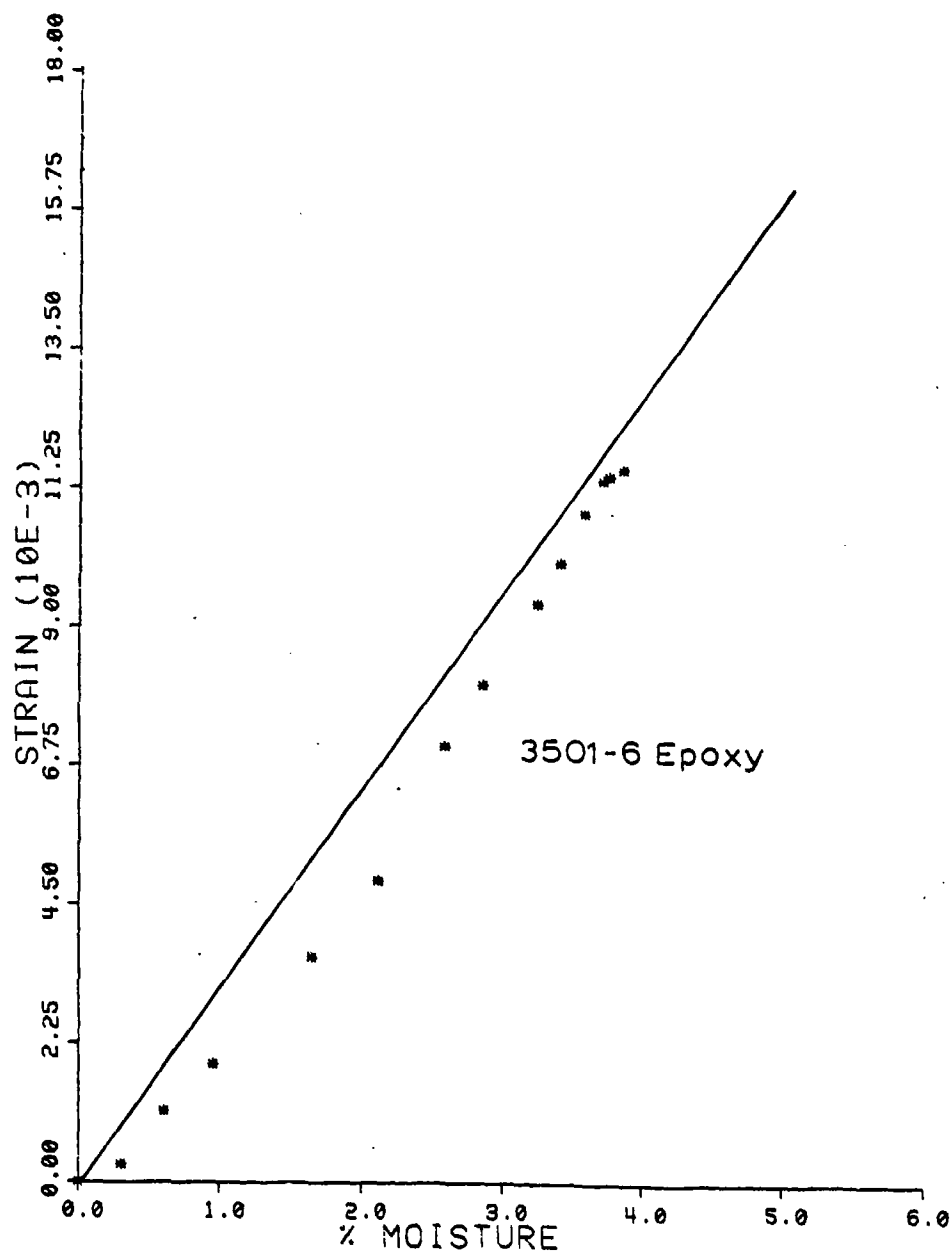
Figure D1. Results of Test 3, Station 1, 10 days @ 98% RH, 65.5°C (150°F)
