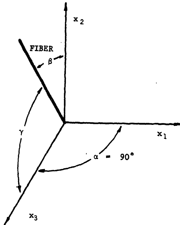
Figure A3. Planar Fiber Orientation
