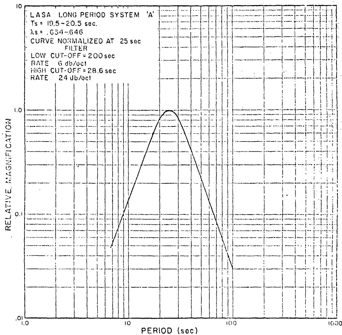
Figure 12. LASA Long Period System "A" Response
