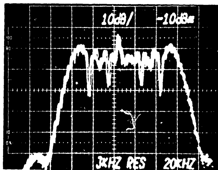
FIGURE 30 - UNCANCELLED ICS OUTPUT WITH ANTENNA SIMULATOR ON TWO-INCH CABLE
