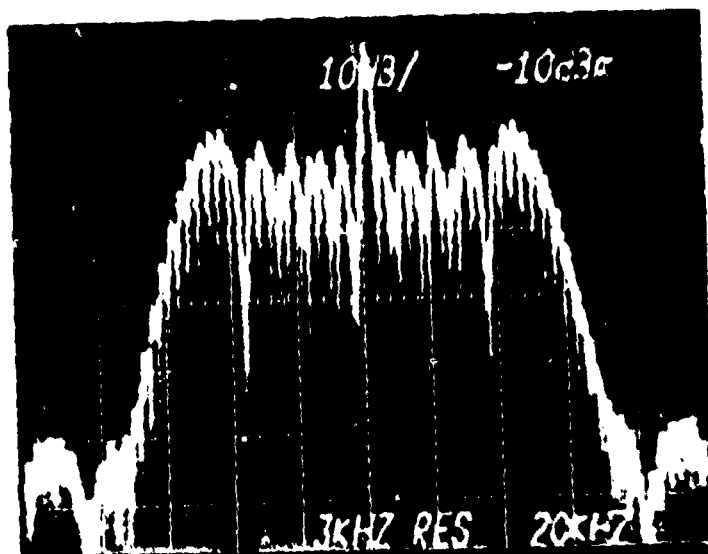
FIGURE 19(A) CW INTERFERENCE + FM PILOT REFERENCE INPUTS DISCON- NECTED (NO CANCELLATION)
