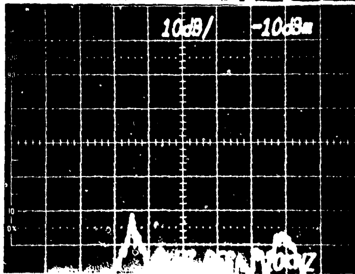
FIGURE 32 ICS OUTPUTS WITH ANTENNA SIMULATOR ON SIX-FOOT CABLE (15 DB RETURN LOSS)
