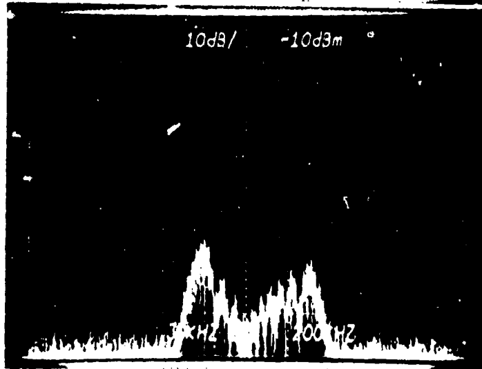
FIGURE 14 RESULTS OF TWO-CHANNEL NOTCH FILTER ICS EXPERIMENT
