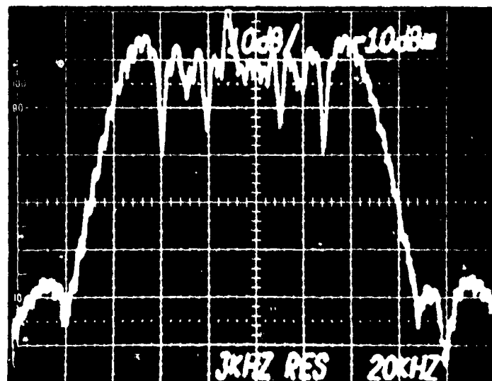
FIGURE 29- RETURN LOSS REFERENCE - ICS OUTPUT WITH ANTENNA PORT OPEN AND NO CANCELLATION
