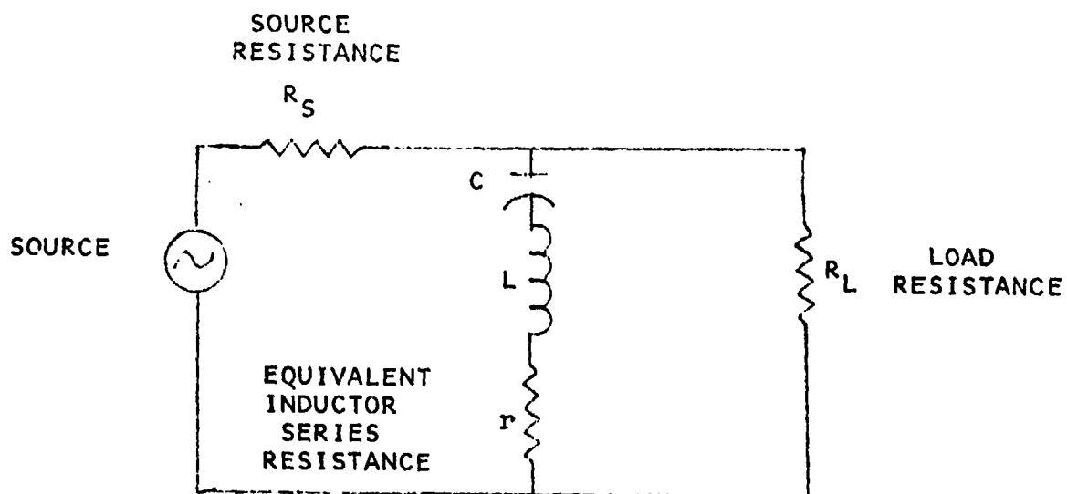
FIGURE 60B RESONANT NOTCH SHUNTING THE LOAD
