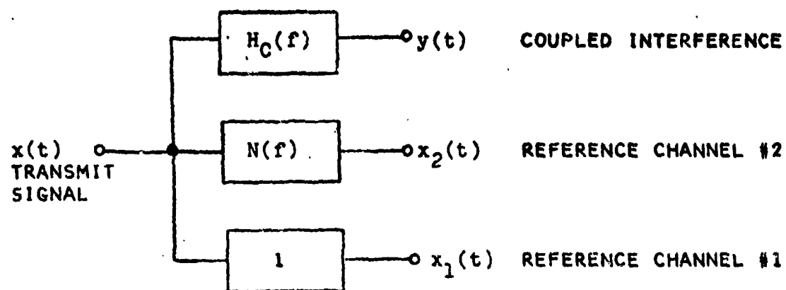
FIGURE 7 SYSTEM REPRESENTATION FOR THE COUPLED INTERFERENCE AND REFERENCE CHANNEL INPUTS
