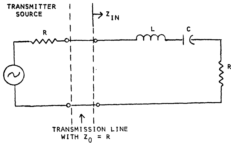
FIGURE 12 RESONANT CIRCUIT MODEL OF SFR ANTENNA
