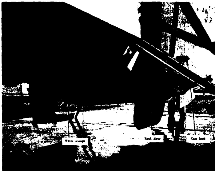
Photo 1. Water Scoops: 5-Inch Internal Diameter. Tank Doors: 30 x 60 Inches. Cam Locks: 2.5-Inch Fire Hose Connector.
