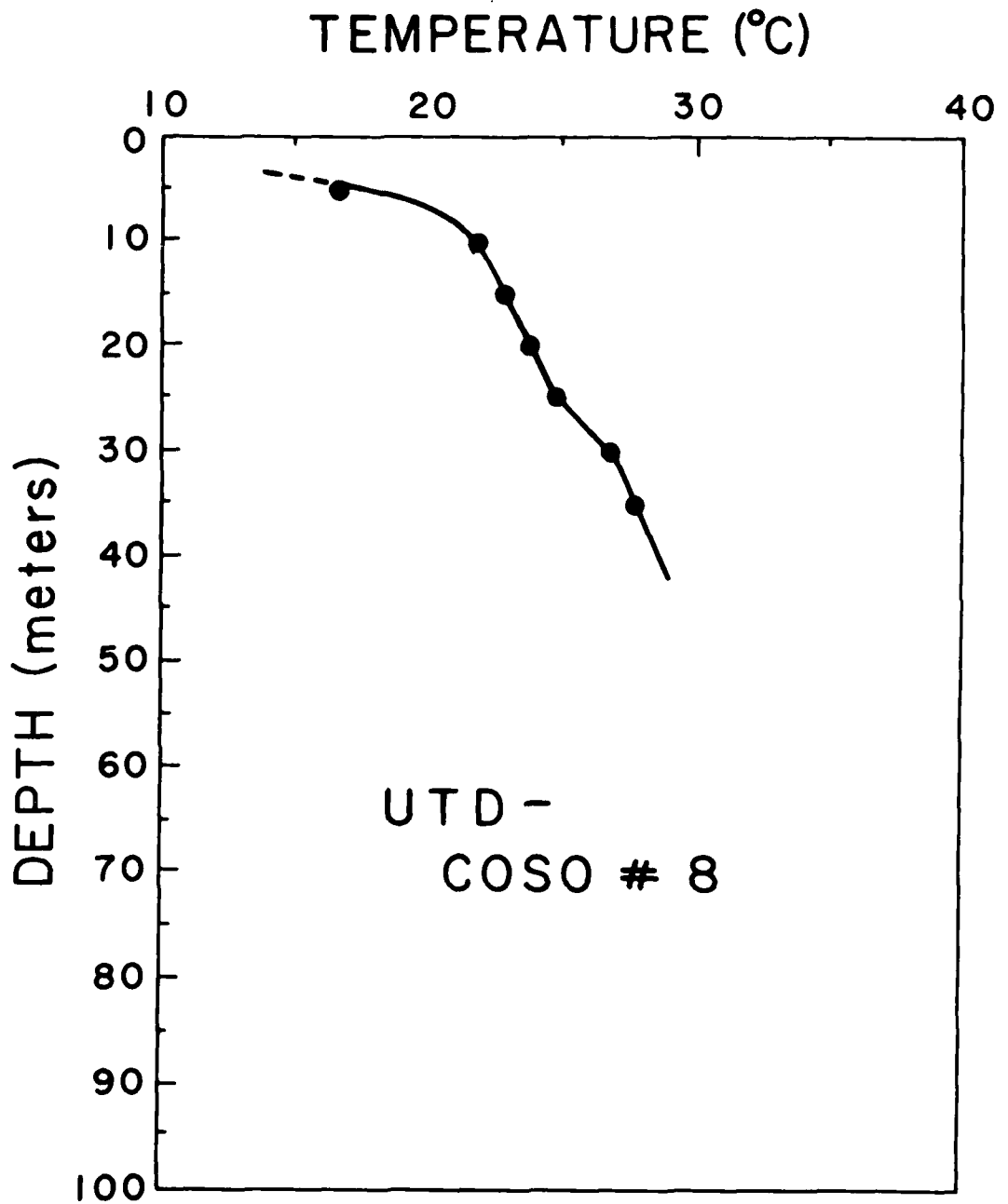
Figure I-6. Temperature-Depth Curve for Borehole UTD-Coso #8.
